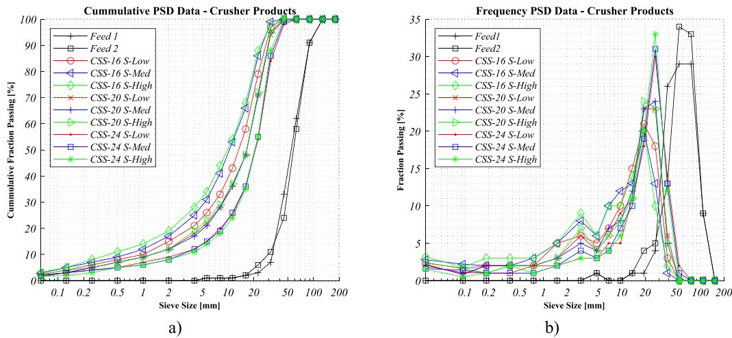
Fig. 2. Particle size distribution for the crusher feed and product from the experiments a) cumulative domain and b) frequency domain.
