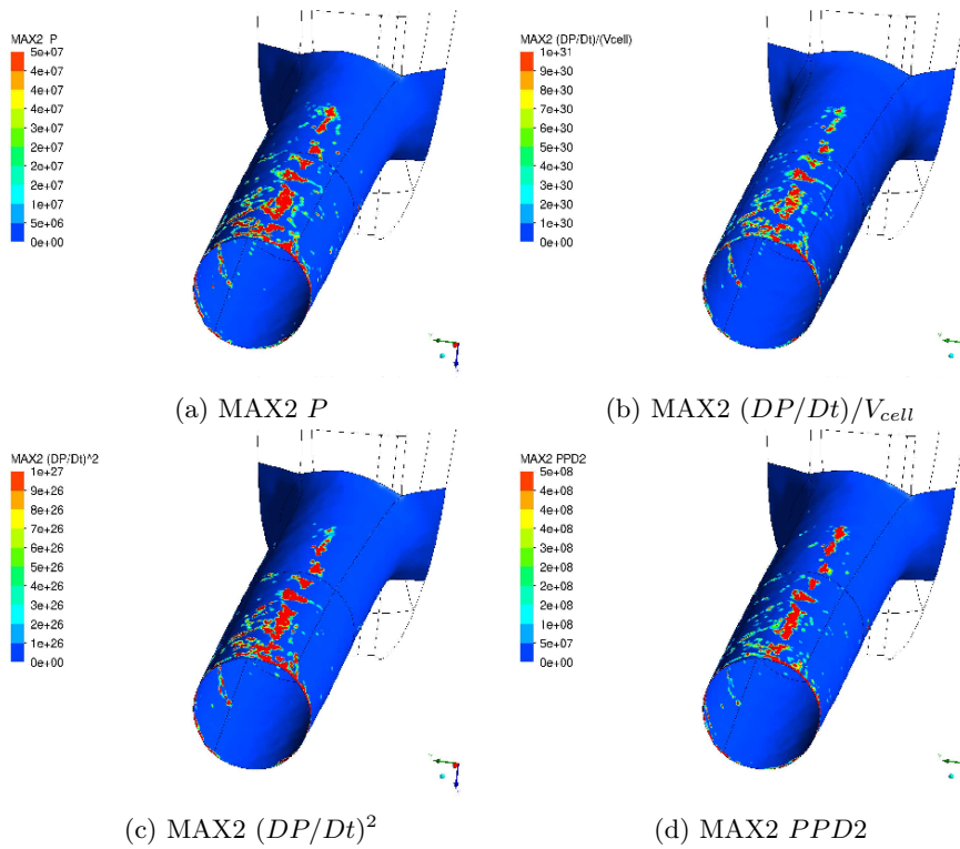
Figure 4.32: Erosion assessment results - TS Model, high lift, RANS
