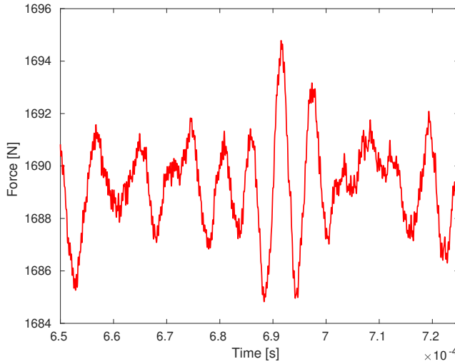
Figure 4.11: Force plot history of the overall orifice surfaces
