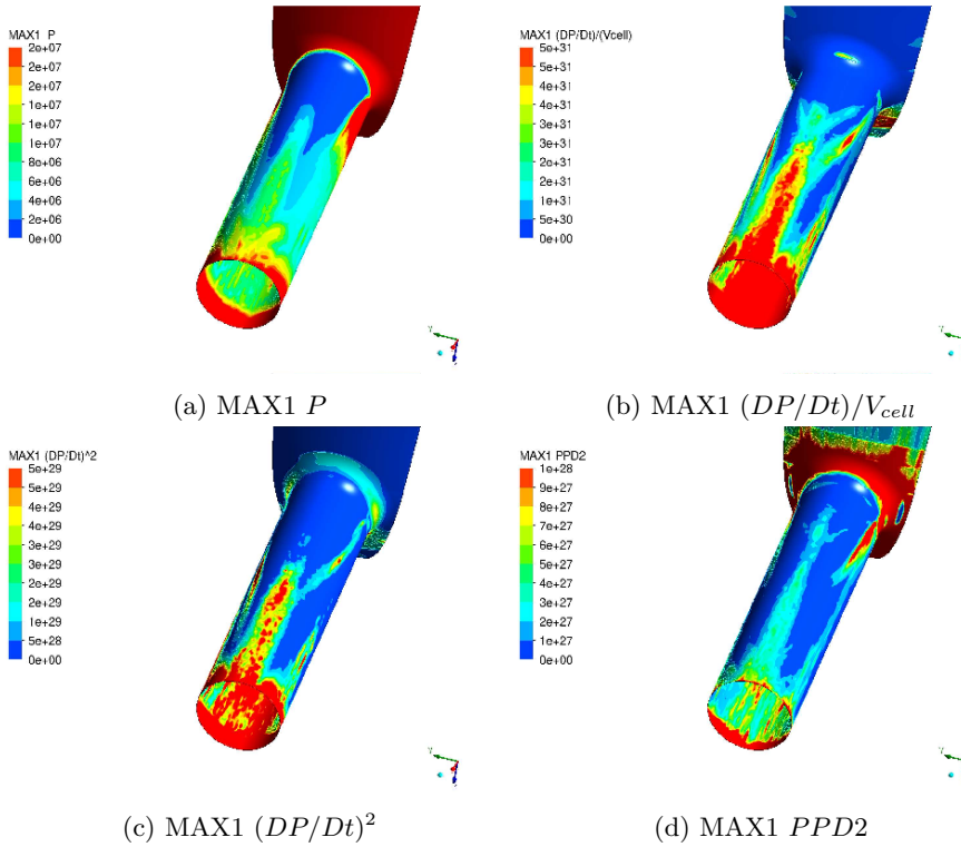
Figure 4.12: Erosion assessment results - CAD Model, high lift, LES
