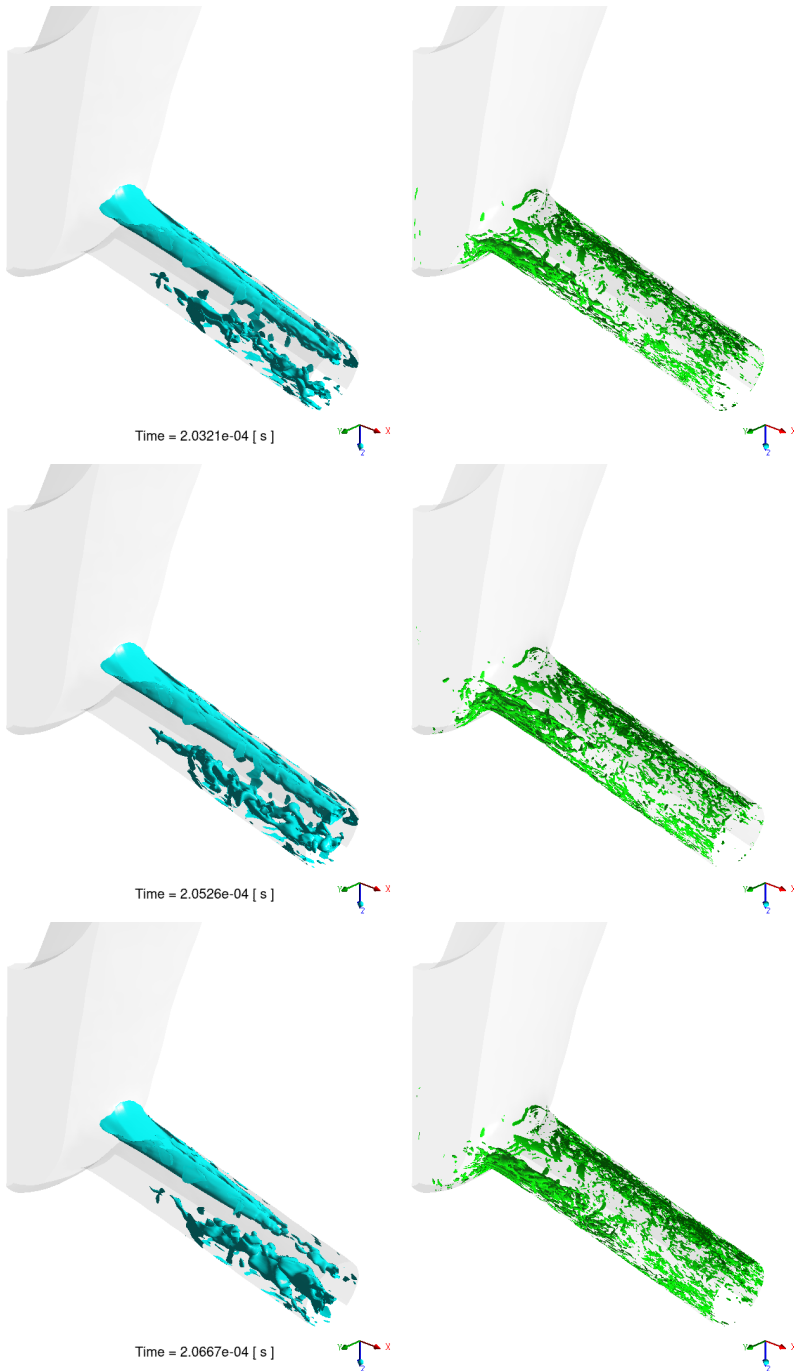
Figure 4.35: Vapor formations ( \alpha = 0.5 ) and turbulent structures ( \lambda_2 = 5 \times 10^{13} ) t4, t5, t6 - TS Model, high lift, LES
