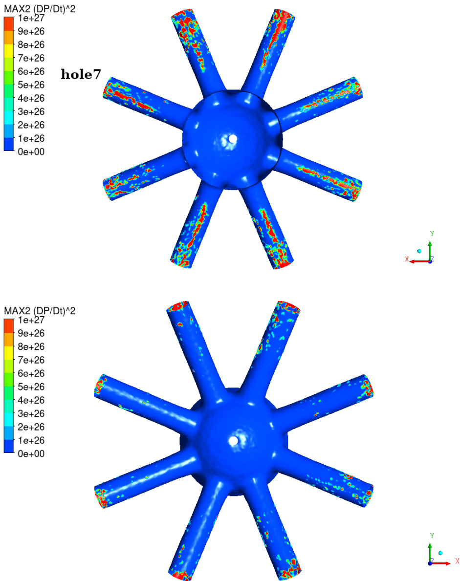
Figure 4.44: Erosion assessment with \text{MAX2 } (DP/Dt)^2 , top and bottom view to the 8-hole injector
