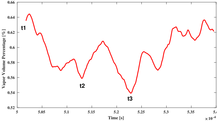
Figure 4.14: Vapor volume percentage change in time
