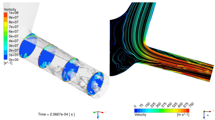
Figure 4.36: Vorticity fields on cross section cut planes together with transparent vapor structures (left) and velocity colored streamlines on injector mid-plane (right)
