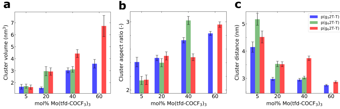
Figure 4.8: Average values of dopant cluster (a) volume, (b) aspect ratio and (c) nearest-neighbour distance. The quantification is based on tomography data of Mo(tfd-COCF 3 ) 3 doped p(g 3 2T-T), p(g 4 2T-T) and p(g 6 2T-T).
