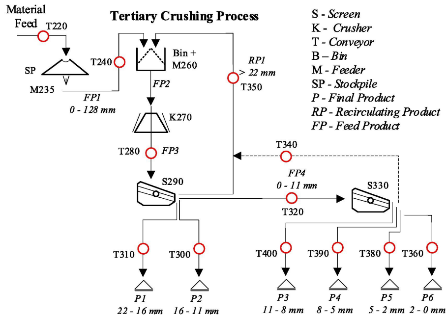
Figure 7: An example of tertiary level crushing and screening in an aggregate plant with the associated machinery needed. P1-P6 represent the final products of different quality based on size distribution of the bulk material (Bhadani et al., 2024).
