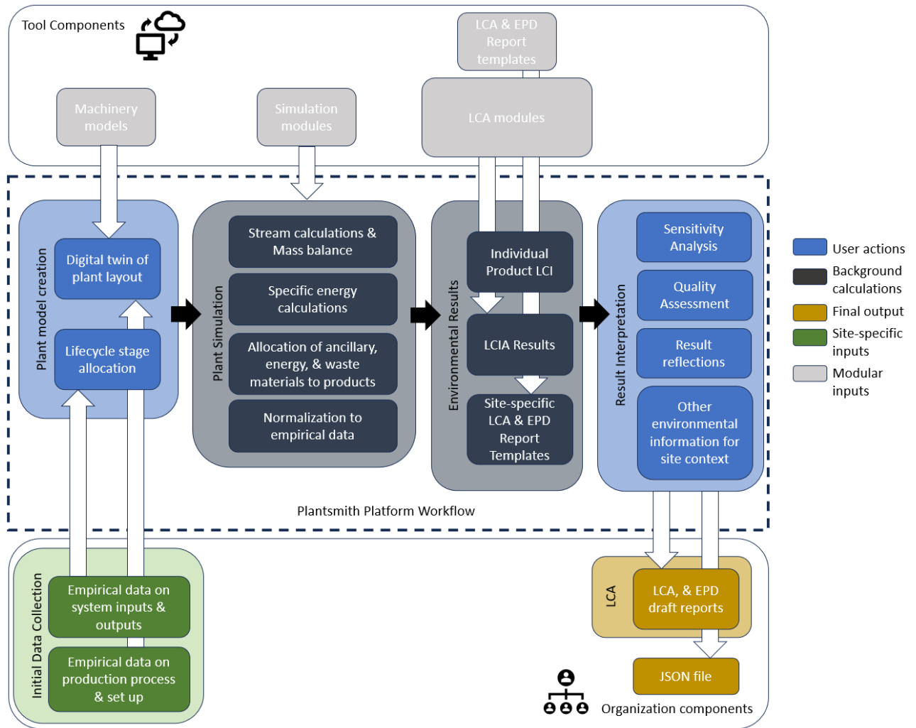
Figure 6: Schematic representation of the modular structure of the tool.
