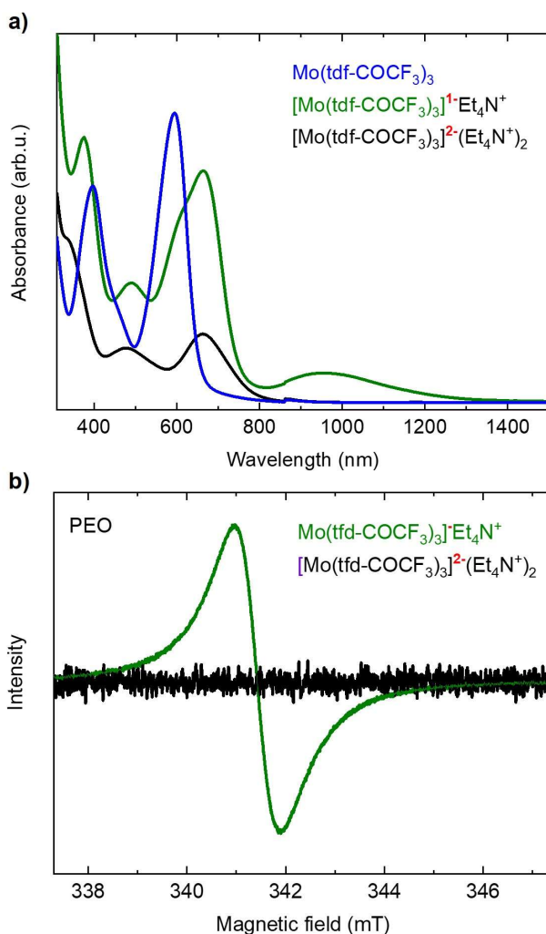
Figure 8.2. (a) UV-vis spectra of \text{Mo}(\text{tfd-COCF}_3)_3 , [\text{Mo}(\text{tfd-COCF}_3)_3]^{1-}\text{Et}_4\text{N}^+ and [\text{Mo}(\text{tfd-COCF}_3)_3]^{2-}(\text{Et}_4\text{N}^+)_2 in dichloromethane (DCM). (b) EPR spectra of [\text{Mo}(\text{tfd-COCF}_3)_3]^{1-}\text{Et}_4\text{N}^+ and [\text{Mo}(\text{tfd-COCF}_3)_3]^{2-}(\text{Et}_4\text{N}^+)_2 dispersed in a polyethylene oxide (PEO) matrix. Reprinted with permission from ref. 131, CC-BY 4.0. The measurement of the EPR spectra and data processing was conducted by Dr. Till Biskup at Saarland University.
