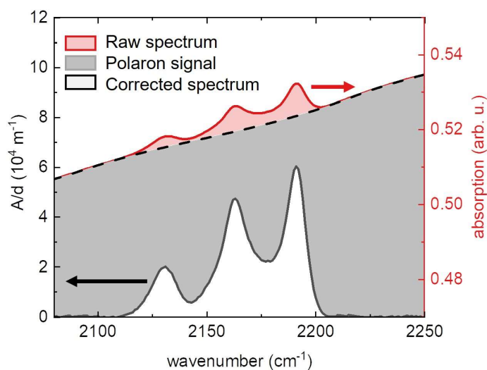
Figure 6.1. Raw FTIR spectrum of p(g 4 2T-T) film doped with 6 mol% F 4 TCNQ (red), baseline (black, dashed) by interpolating a baseline line to data points just outside the peak area and spectra corrected for the underlying polaron signal where the absorption is normalized by sample thickness (black).
