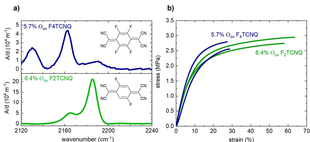
Figure 7.3. a) Transmission FTIR absorbance spectra, with the absorbance normalized by the film thickness A/d , of p(g 4 2T-T) doped with 3 mol% F 4 TCNQ (blue; O ox = 5.7%) and 6 mol% F 2 TCNQ (green; O ox = 6.4%); (b) stress–strain curves recorded at room temperature by tensile deformation of freestanding samples of p(g 4 2T-T) doped with 3 mol% F 4 TCNQ (blue) and 6 mol% F 2 TCNQ (green). Reproduced from Ref. 101 with permission from the Royal Society of Chemistry. The mechanical analysis was performed by Dr. Sepideh Zokaei.
