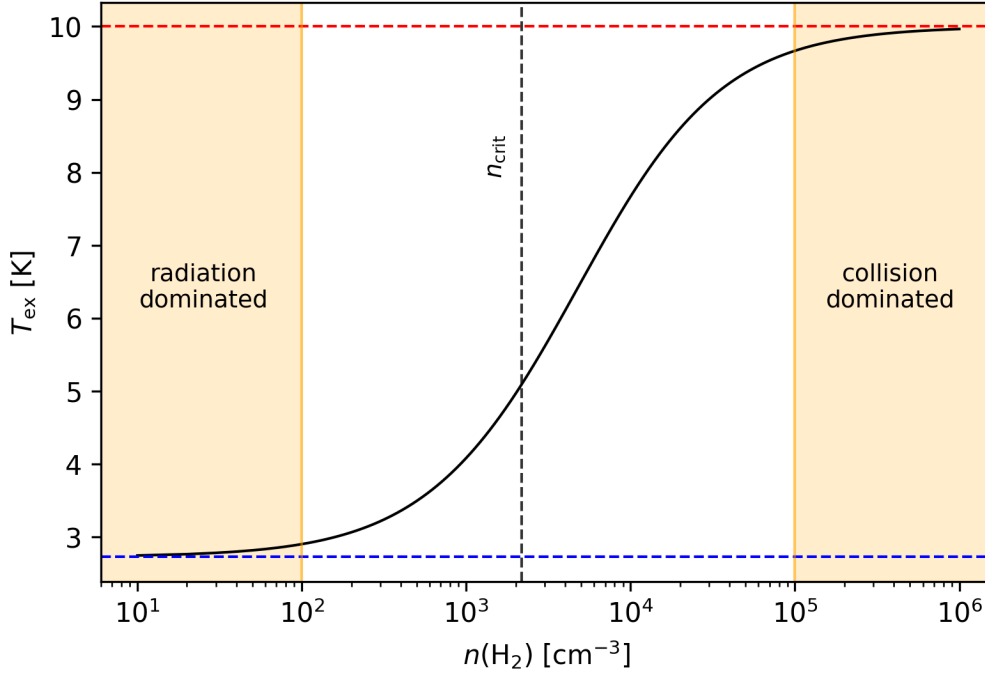
Figure 2.5: Excitation temperature T_{\text{ex}} corresponding to the level population n_u/n_l of the CO(1 – 0) two-level system as a function of \text{H}_2 density, calculated from Eq. (2.34). The population of levels is calculated from Eqs. (2.30) and (2.33). As can be seen, T_{\text{ex}} approaches the assumed background temperature (2.725 K; dashed blue line) at low densities, but the assumed kinetic temperature (10 K; dashed red line) at high densities. The shaded orange areas mark the approximate densities at which the underlying population of levels is dominated by either radiation or collisions. The vertical dashed black line labelled " n_{\text{crit}} " marks the critical density of CO(1 – 0), as calculated from Eq. (2.37).
