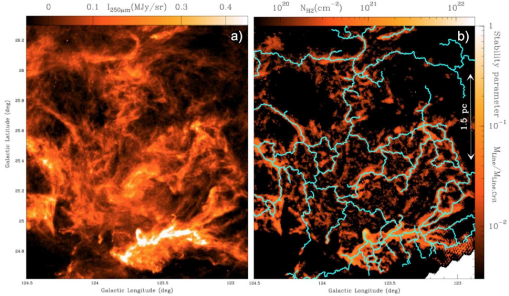
Figure 1.3: (a): HSO (Herschel Space Observatory) 250 μm dust continuum map of a part of the Polaris Flare. (b): corresponding H 2 column density map. The light blue lines indicate a network of over-dense filaments. The critical mass per unit length is expressed in terms of the stability parameter M_{\text{Line}}/M_{\text{Line,Crit}} . Credit: André et al. (2014).
