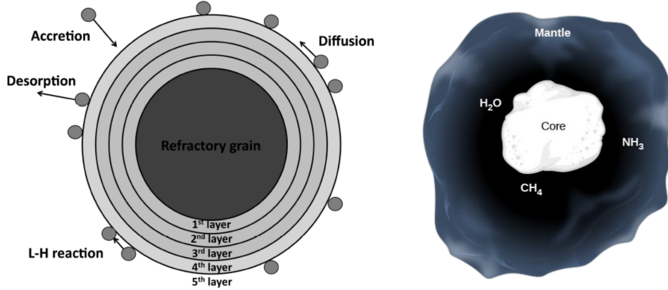
Figure 1.4: Left: gas-grain interactions (accretion, diffusion, reaction, and desorption) lead to the build up of solid ices at the surface of refractory, interstellar dust grains. Credit: Taquet et al. (2012) . Right: early ice species include \text{H}_2\text{O} , \text{CH}_4 , and \text{NH}_3 , that form by subsequent hydrogenation of O, C, and N. Credit: College Sidekick (2024) .
