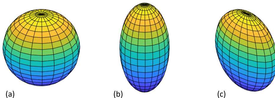
Figure 2.1: Ellipsoidal quadric surfaces resulting from different, relative MoI components ( I_a , I_b , and I_c ) in Eq. (2.2): (a) sphere ( I_c = I_b = I_a ), (b) prolate spheroid ( I_c = I_b > I_a ), (c) oblate spheroid ( I_c > I_b = I_a ). A triaxial ellipsoid ( I_c \neq I_b \neq I_a ) is a mixture of figures (b) and (c).
