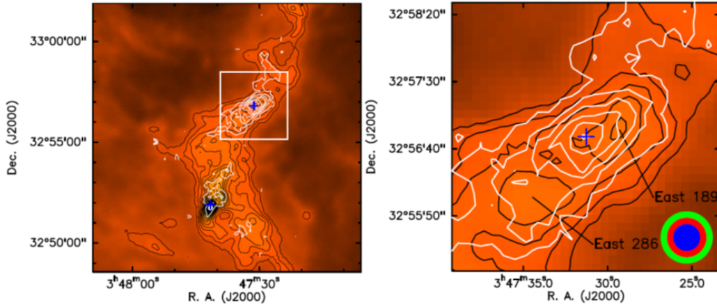
Figure 3.1: Left: Herschel/SPIRE map of the B5 dark cloud at 250\mu\text{m} (orange scale and black contours) and IRAM 30m integrated intensity map of the \text{A}^+-\text{CH}_3\text{OH}(3_0 - 2_0) transition (white contours in steps of 5\sigma , with \sigma = 50\text{ mK km s}^{-1} ); the blue crosses depict the positions of B5-IRS1 in the South and the methanol hotspot in the North. Credit: Taquet et al. (2017) . Right: enlarged view on the B5 methanol hotspot (blue cross), located in between the \text{H}_2 column density peaks East-189 and East-286. The green, red, and blue circles in the bottom right corner represent the beam sizes of the OSO 20 m, IRAM 30 m, and NRO 45 m telescopes at 3 mm, respectively. Credit: Taquet et al. (2017) .
