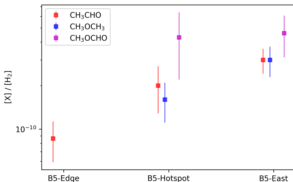
Figure 4.3: Gas phase abundances (relative to \text{H}_2 ) of acetaldehyde ( \text{CH}_3\text{CHO} ), di-methyl ether ( \text{CH}_3\text{OCH}_3 ), and methyl formate ( \text{CH}_3\text{OCHO} ) towards B5-Edge, B5-Hotspot, and B5-East. A 15 % uncertainty is assumed for the \text{H}_2 column density, which is derived from HGBS data. For B5-Hotspot, column density data for \text{CH}_3\text{OCH}_3 and \text{CH}_3\text{OCHO} is taken from Taquet et al. (2017), and for \text{CH}_3\text{CHO} from Carl et al. (2023).
