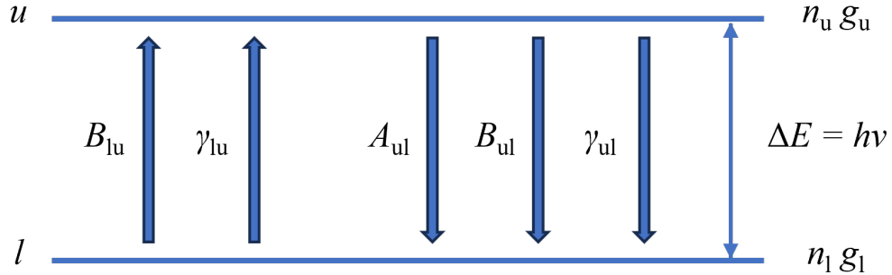
Figure 2.4: Transitions between the energy levels of a two-level system are driven by radiative processes ( B_{lu} , B_{ul} , and A_{ul} ) and collisional processes ( \gamma_{lu} and \gamma_{ul} ). \Delta E is the energy separation between both levels, n_u and n_l are the numbers of molecules in the upper and lower levels, respectively, and g_u and g_l are the statistical weights of both levels.
