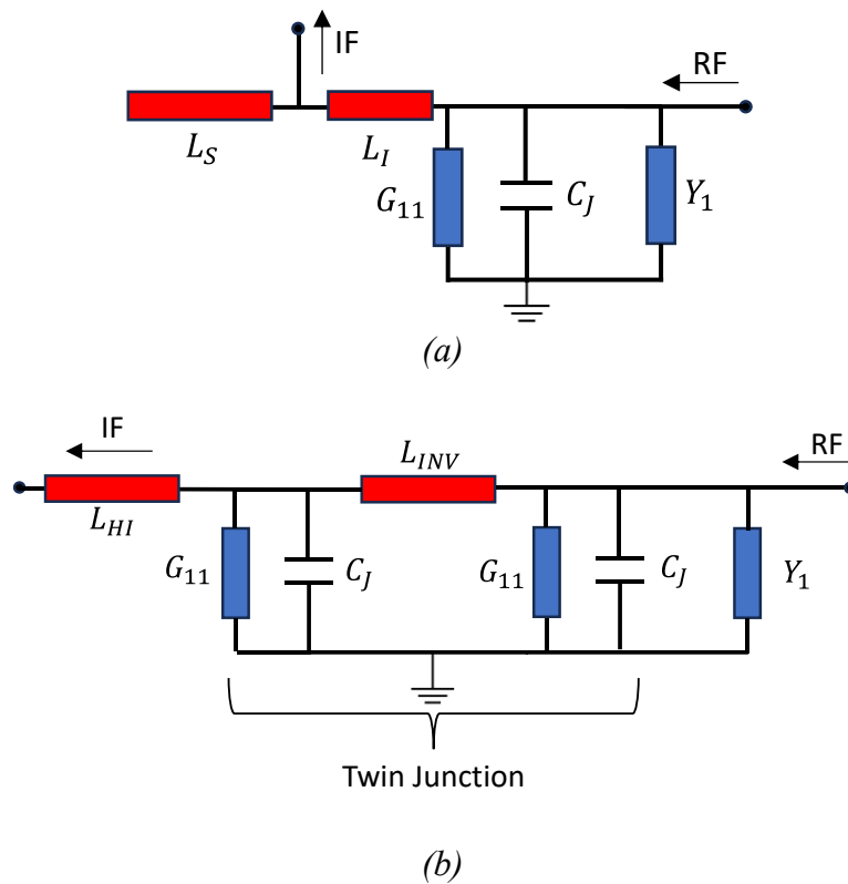
Fig. 4.4. Equivalent circuits for SIS RF matching. The IF extraction point is shown in each case. Note that to increase the RF/LO rejection a filter is commonly employed at the IF extraction. (a) A single SIS junction with an inductive piece of line L_I for susceptance compensation and open \lambda/4 stub to create a point for IF extraction. (b) RF equivalent circuit for twin junction. The piece of line L_{INV} between the junctions acts as an impedance inverter to cancel the capacitive susceptance. A high-impedance line L_{HI} is commonly employed for IF extraction.
