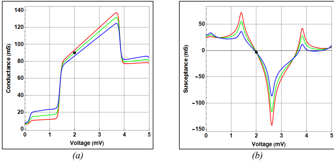
Fig. 4.2. Example of simulated real and imaginary parts of the complex admittance for the SIS junction at RF. The nominal bias point is marked with a black dot. (a) RF conductance for 3 values of \alpha , 0.5 (blue), 0.8 (green), and 0.9 (red). (b) RF susceptance for 3 values of \alpha , 0.5 (blue), 0.8 (green), and 0.9 (red). Note that the design's nominal bias voltage is generally chosen in the middle of the first photon step before the gap voltage V_g where B_{1,1} is closer to 0.
