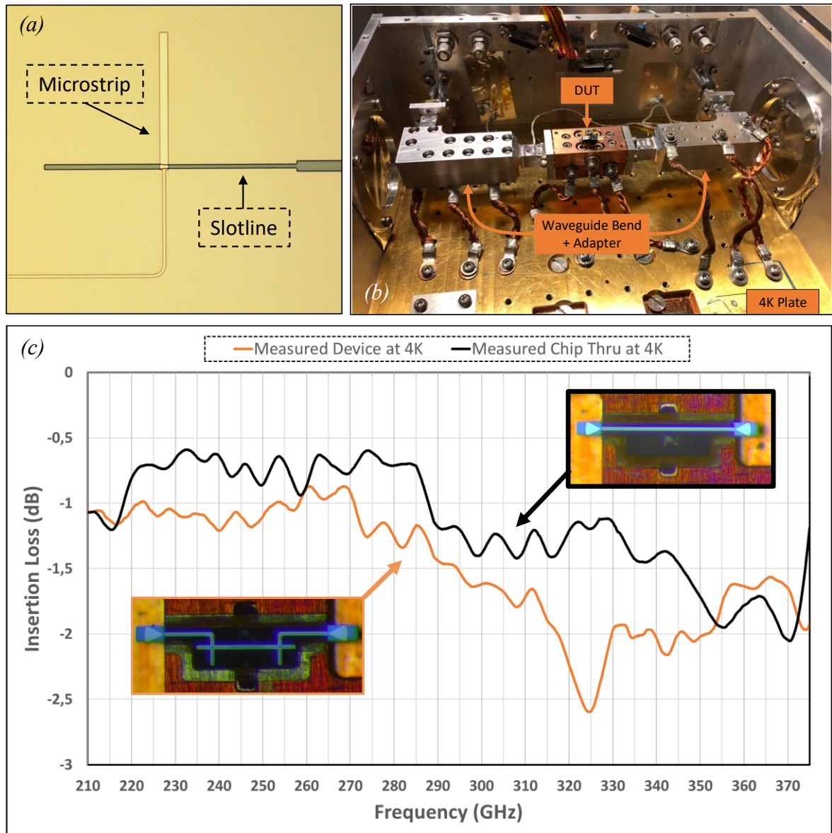
Fig. 3.5. Marchand Balun transition proposed in [Paper E]. (a) A photograph of the fabricated Microstrip to Slotline transition is depicted. (b) Measurement setup inside a closed cycle cryostat. (c) Insertion loss measurements at cryogenic temperatures of the chip with thru connection and the chip with the Marchand balun structure.
