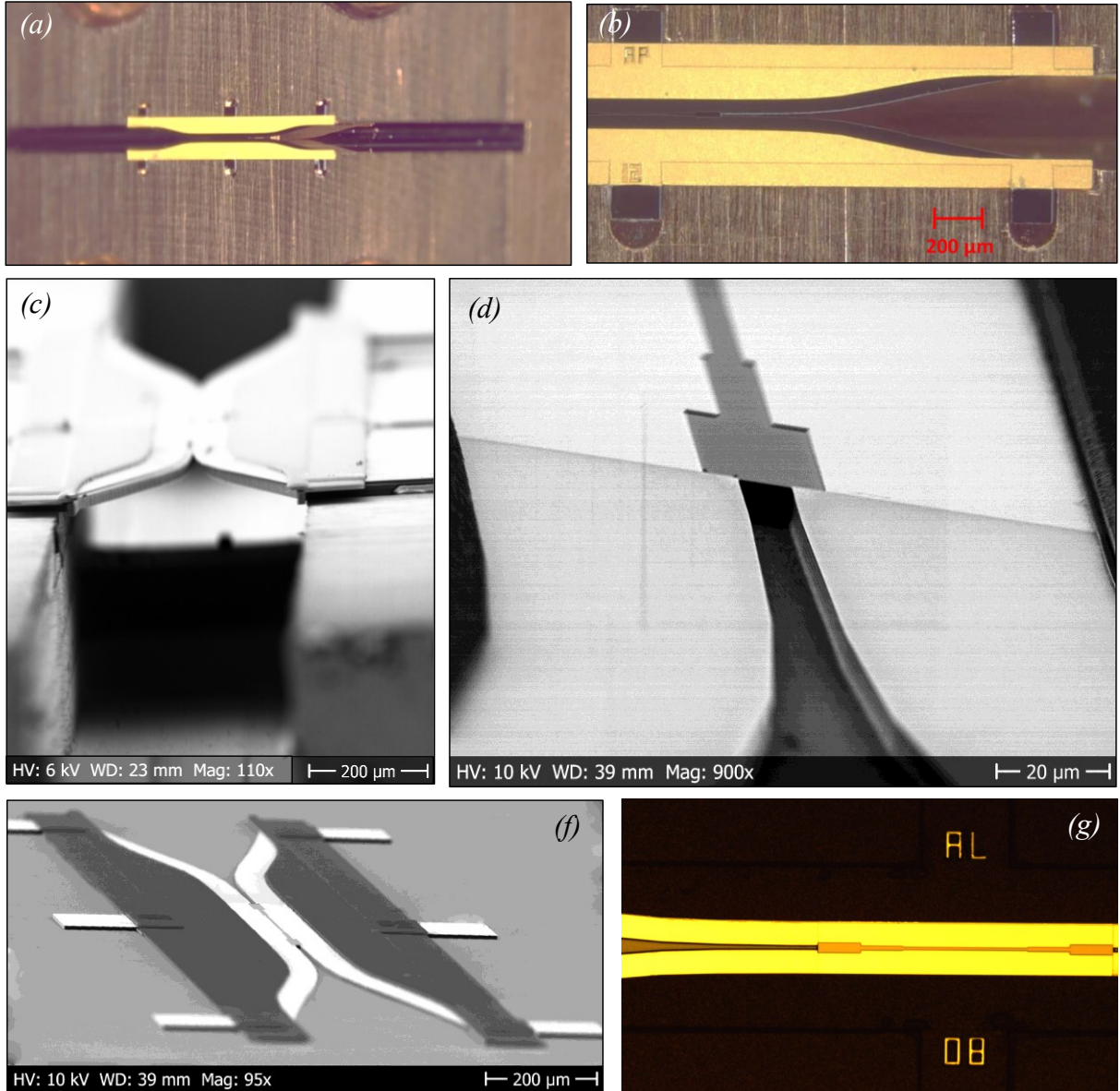
Fig. 3.4. Fabricated waveguide to substrate transition. (a) Finline mounted in the tellurium-copper waveguide block with dimension 800 \times 400 \mu\text{m} (b) Magnified image of the mounted finline. (c) Scanning electron microscope (SEM) image of the fabricated back-to-back device mounted into the split-block. (d) SEM picture of the finline structure after etching the first 5 \mu\text{m} of the Si device layer. The verticality of the side walls could be appreciated. (e) SEM picture of the device before release. (f) Detail of the central slotline transformer in a back-to-back configuration.
