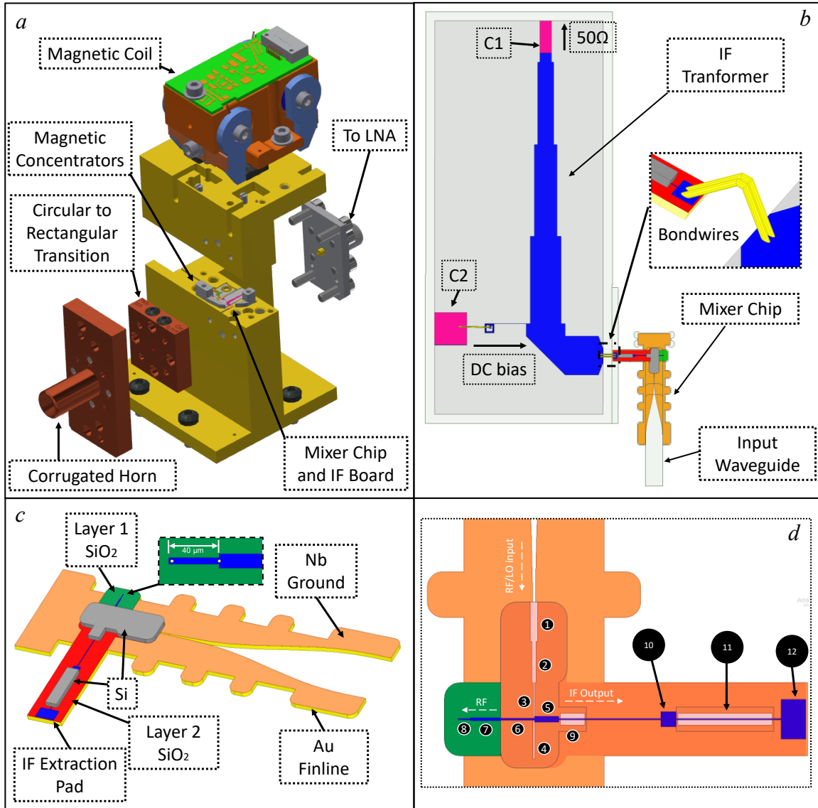
Fig. 4.4. Proposed Mixer Chip in [Paper G]. (a) Exploded view of the DSB block 3D model. (b) Detailed view of the IF board and a layout of the mixer chip. (c) Mixer chip's different layers. (d) Detail of the RF matching and IF output circuitry integrated on the metallic chip. Slotlines 1 and 2 are employed for reducing the impedance from 100 Ohm to 60 Ohm, facilitating a smoother transition from slotline to microstrip. The Marchand Balun is formed by slotlines 3 and 4, and microstrips 5 and 6. This transition is employed for further impedance transformation, acting as a bridge between the higher impedance slotlines and the lower impedance required by the SIS junctions. Microstrips 6 and 7 are a two-section Chebyshev transformer for a broadband impedance match to the SIS junctions. Line 8 is the impedance inverter of the twin junction. Lines 9 to 12 constitute the IF extraction circuitry, forming the RF/LO filter. Suspended microstrips are employed as high-impedance lines.
