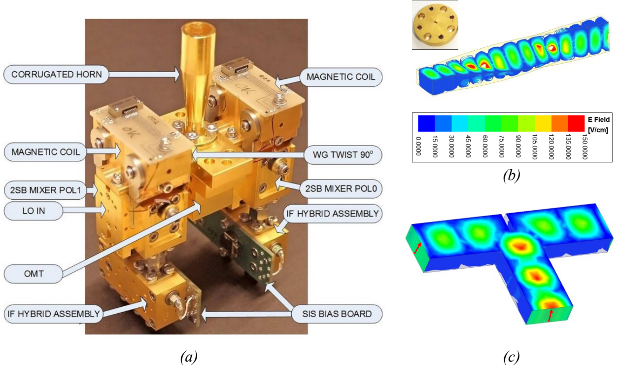
Fig. 2.1. (a) Example of S2B mixer assembly, ALMA Band 5 [38]. Various waveguide components are shown: For instance, corrugated horn, OMT, 90^\circ continuous Waveguide Twist, IF hybrids (b) E-field magnitude simulation of a continuous twist. It is appreciated how the E-field of the rectangular waveguide main mode is gradually rotated along the continuous twist. Top:left image of continuous 90^\circ waveguide twist employed in [38]. (c) E-field magnitude simulation of a classical waveguide power divider based on T-Junction with septum.
