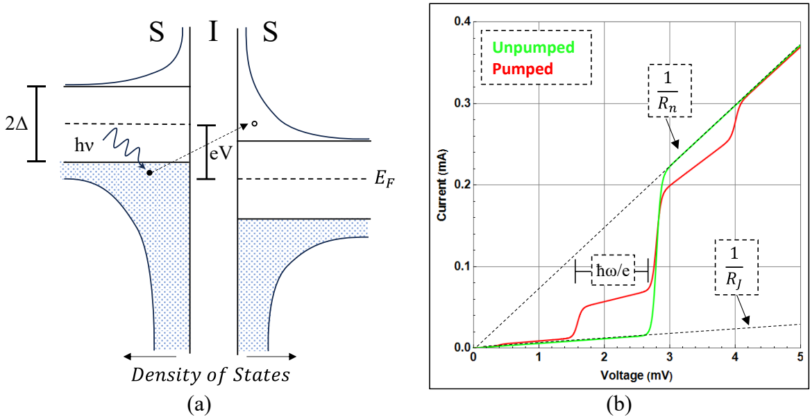
Fig. 1.3. SIS principle of operation. (a) Energy bands of a biased superconducting-insulating-superconducting (SIS) structure. The copper pair is broken by the incoming photon which allows the quasiparticle to tunnel through the insulator. (b) Simulated current voltage curve (IVC) for Unpumped (green), i.e., without LO power applied to the junction, and Pumped (red), i.e. when LO power is applied to the junction. Moreover. The photon assisted tunneling step below the gap is shown. Note that V_g is 2.8 mV. The normal resistance of the junction and the subgap resistance ( R_n ) are indicated as the inverse of the slope for the normal and subgap regions of the SIS. Since R_J is related to the subgap leakage current, the relation R_J/R_n is employed as a measure of the quality of the junction.
