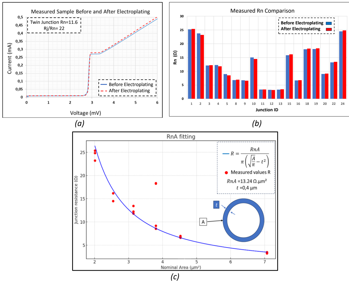
Fig. 4.7. Cryogenic measurements of the SIS junctions. (a) Measured IV curve before and after electroplating. (b) R_n variation before and after electroplating of each fabricated junction. (c) R_n A fitting. The R_n A of the batch results is 13.24 \Omega \cdot \mu\text{m}^2 with a fabrication offset of t=0.4 \mu\text{m} .
