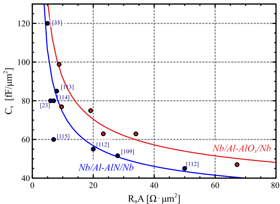
Fig. 4.5. Specific capacitance as a function of R_n A for SIS barriers of \text{AlO}_x and AlN for various authors. The Nb/Al- \text{AlO}_x /Nb data points are extracted from [111]. The graph was adapted from [109]. The C_s capacitance data for the junctions are approximated with the relation C_s = a / \ln(R_n A) [110], where a is equal to 211 [111] for the Nb/Al- \text{AlO}_x /Nb junctions and 170 for Nb/Al-AlN/Nb junctions [112].
