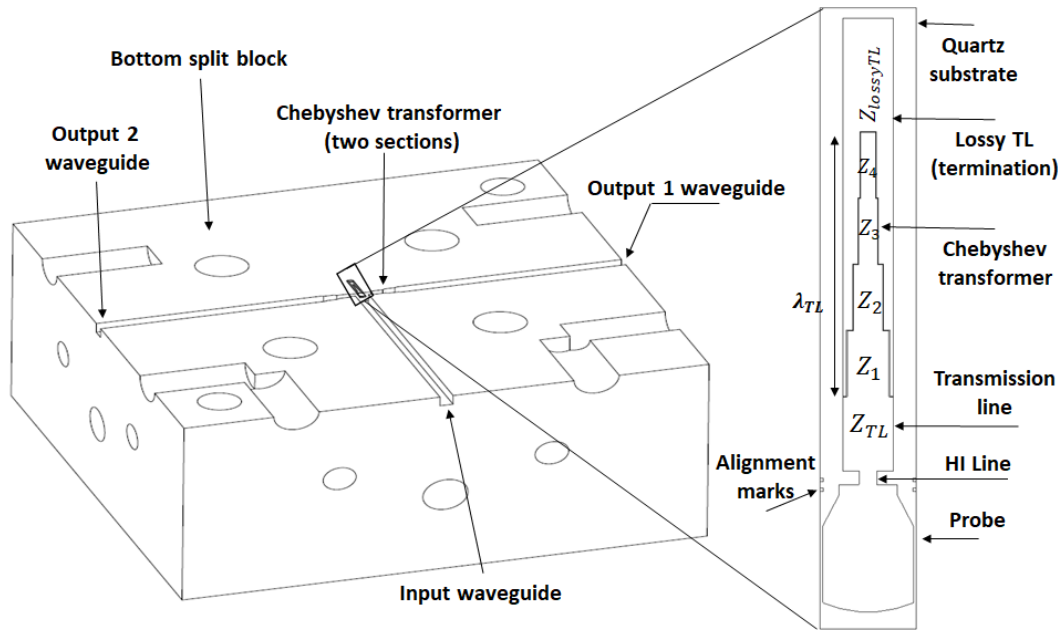
Fig.2.3. Power divider presented in [Paper C]. Detailed 3D drawing of the bottom waveguide split block and the overall chip layout.
