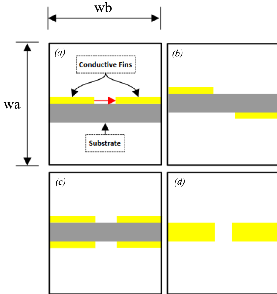
Fig. 3.2. Cross section of four commonly used finline configurations. Dimensions a and b of a standard rectangular waveguide are indicated as wa and wb . (a) In the unilateral finline configuration the fins are located on only one side of the substrate. The red arrow illustrates the electric field excitation of the fin-gap. (b) Antipodal configuration. (c) Bilateral. (d) Metallic Finsline.
