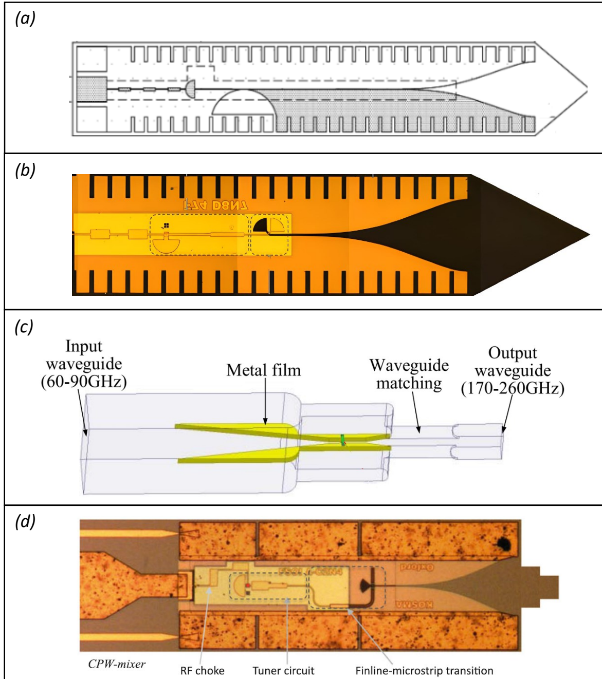
Fig. 3.3. Examples of finline devices (a) Antipodal SIS finline mixer designed for 350 GHz operation. [81] (b) SIS mixer fabricated on 60 \mu\text{m} quartz substrate. The finline transition makes use of a triangular notch in the substrate to improve matching. In addition, serration chokes are employed to guard against the propagation of substrate mode. [83] (c) Metallic finline employed for a Schottky frequency tripler [84] (d) SIS mixer fabricated over 15 \mu\text{m} Si substrate. Note that a multi-stage silicon matching notch is employed. Since the Si substrate is extremely thin, no serration is needed to preclude substrate modes from propagating. [83].
