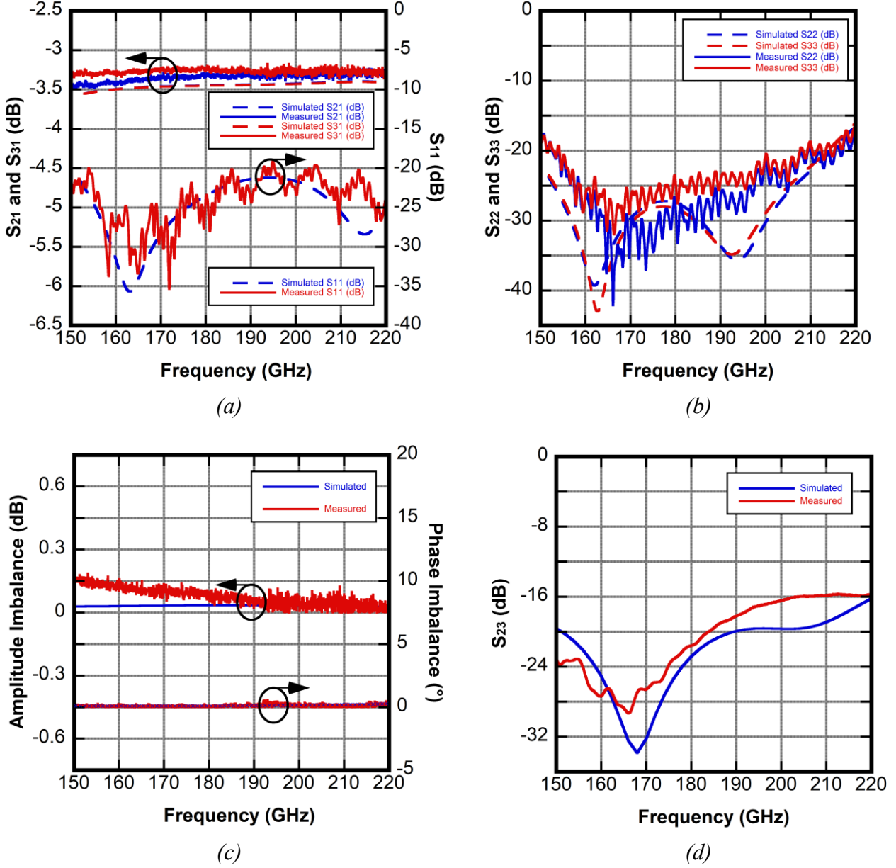
Fig.2.4. Simulation and Measurement results for Waveguide Power Divider proposed in [Paper C]. (a) insertion loss and input return loss, (b) output return loss, (c) amplitude and phase imbalance, and (d) isolation of the power divider.
