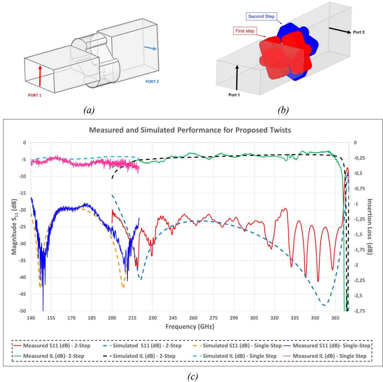
Fig. 2.2. Compact wideband waveguide twists. Note that dashed lines indicate simulated performance and continuous lines depict measurements results. (a) Layout for the single-step twist described in [Paper A] (b) Layout for the 2-step twist presented in [Paper B] (c) Measured and simulated performance for proposed waveguide twists.
