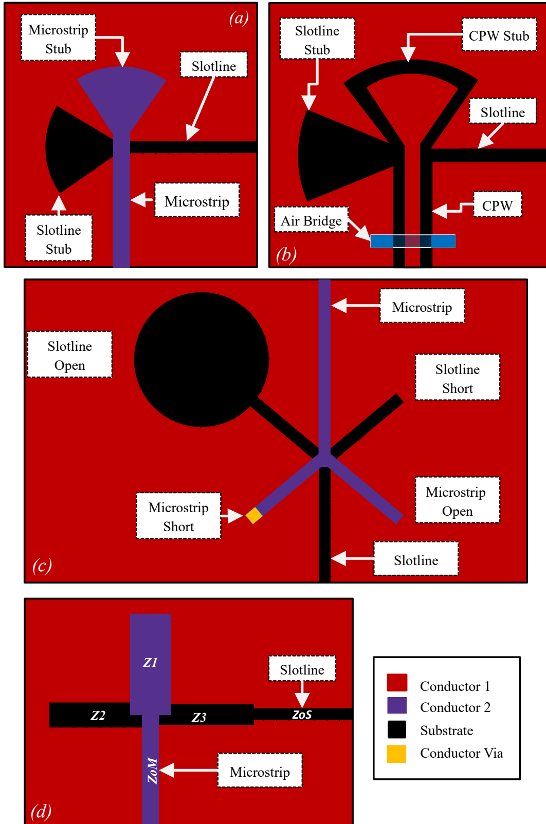
Fig. 3.6. Slotline to microstrip transitions. It is important to note that the dielectric layer located between the conductors is not shown in the images for clarity. (a) Cross-junction transition. (b) Indirect transition with CPW. (c) Double Y balun transition (d) Marchand balun transition.
