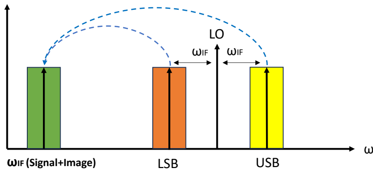
Fig. 1.4. Illustration of the downconversion employing DSB mixer configuration.
