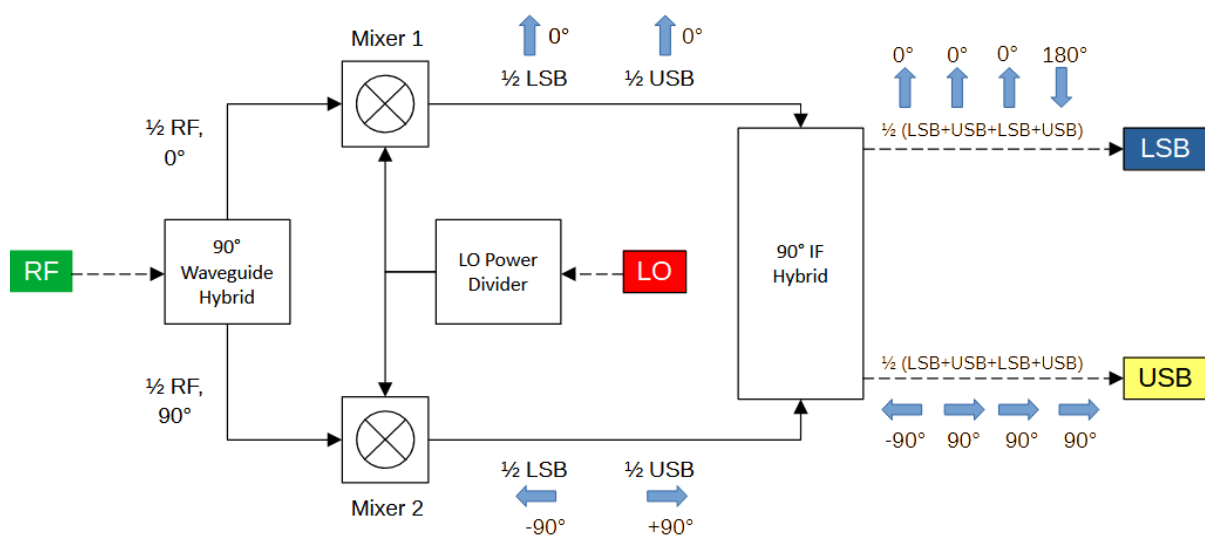
Fig. 1.5. Block Diagram of a Sideband Separating Mixer 2SB. The signal phasor for each sideband illustrates the sideband separation process.
