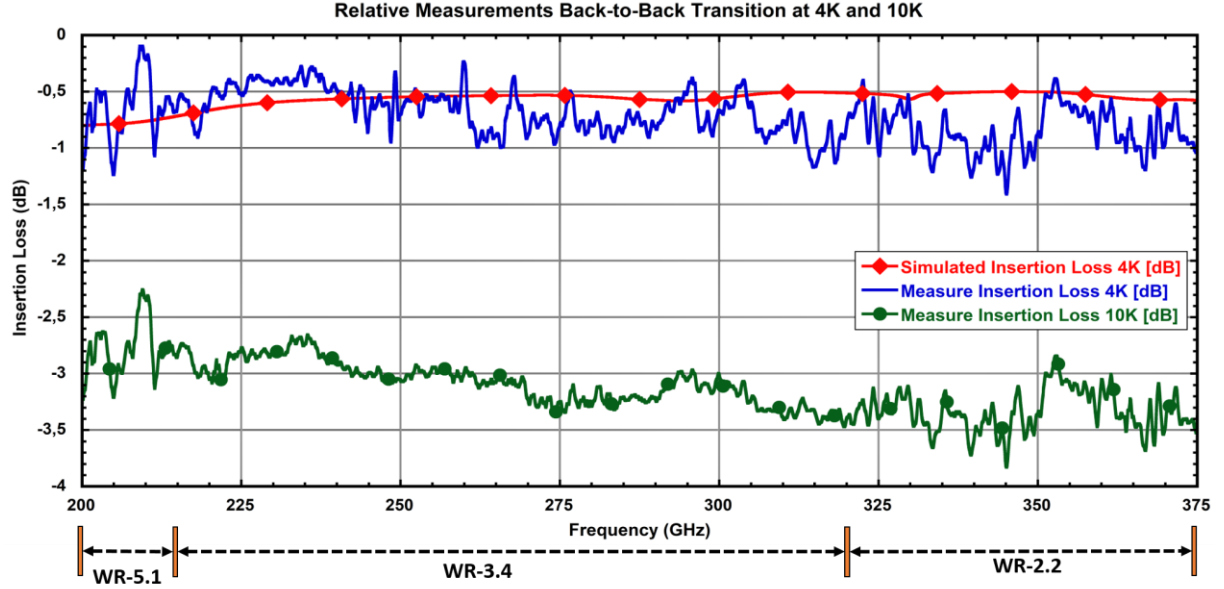
Fig. 3.5. Measured Insertion loss of the proposed finline in [Paper D] at the physical temperature of 4K and 10K. It can be seen how the losses above the transition temperature for Nb increase considerably. The simulation at 4K is shown in red. Three different VNA extension modules were used in the experiment to be able to cover the frequency range of 200-375GHz.
