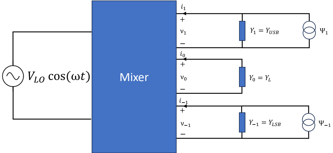
Fig. 4.1. Circuit model for 3 port heterodyne mixer presented in [24]. A sinusoidal LO frequency is applied generating 2 sidebands and an IF output. The RF signal applied to each sideband is represented by the current sources \Psi_1 and \Psi_{-1} for the USB and LSB, respectively.
