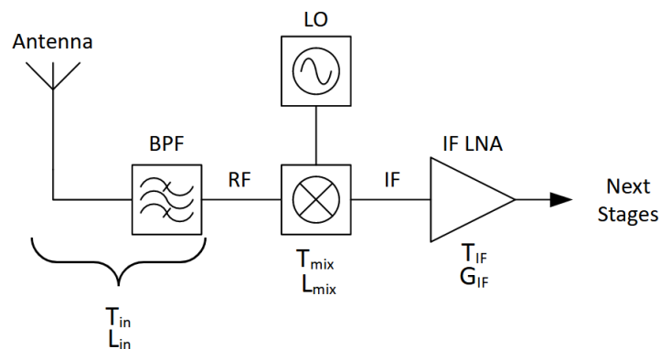
Fig. 1.6. Simplified block diagram for heterodyne receivers for radio astronomy applications.
