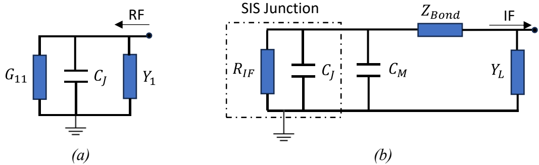
Fig. 4.3. Equivalent circuits for SIS at RF and IF. (a) RF equivalent circuit for a single junction bias at nominal voltage. G_{1,1} is the conductance of the SIS and C_J its geometric capacitance. Y_1 is the embedded admittance of the mixer, i.e. the admittance showed to the junction by the waveguide-to-substrate transition and the RF matching circuitry. (b) Simplified IF equivalent circuit for a single SIS junction. C_M corresponds to the capacitance added by the RF matching circuitry. Y_L is the load impedance that might be adjusted to control the conversion efficiency of the mixer. It is important to consider the impedance of the bonding wires for IF extraction Z_{Bond} .
