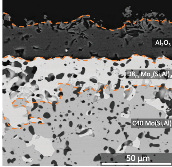
Figure 2.10: Cross-section of an oxidised \text{Mo}(\text{Si},\text{Al})_2 sample. The \text{Mo}_5(\text{Si},\text{Al})_3 layer is seen in bright contrast between the oxide and \text{Mo}(\text{Si},\text{Al})_2 .
