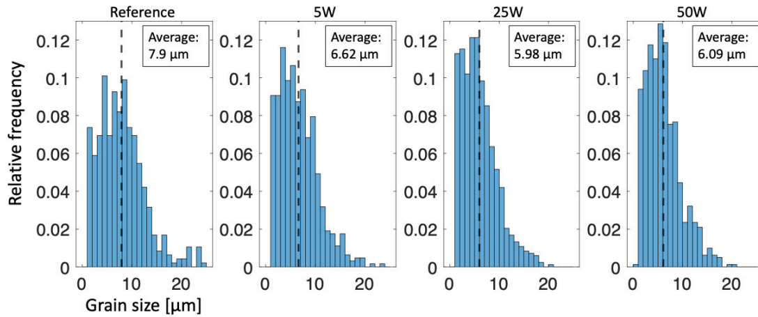
Figure 5.21: Grain size distribution of the reference and W-alloyed materials.
