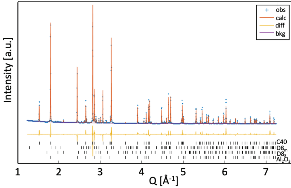
Figure 4.12: Rietveld refinement of \text{Mo}(\text{Si,Al})_2 using GSAS-II. R_w=2.10\% .
