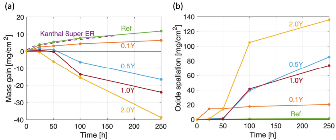
Figure 5.25: (a) The mass gain of Y-alloyed \text{Mo}(\text{Si},\text{Al})_2 materials oxidised in air at 1500 °C, and Kanthal Super ER oxidised in dry air at 1500 °C [60]. (b) The mass of spalled oxide from the Y-alloyed materials.
