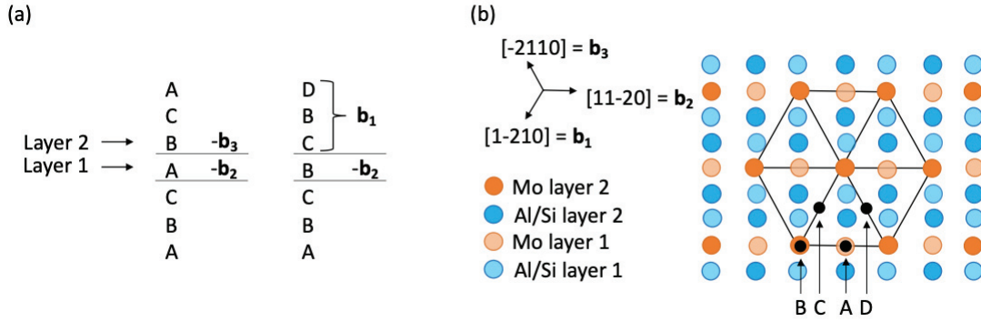
Figure 2.4: (a) Synchroshear mechanism giving rise to the total displacement of \mathbf{b}_1 for Layer 2 and all layers above, (b) stacking of C40 basal layers. The bright atoms are positioned in Layer 2 above Layer 1 (faded atoms). Position A, B, C and D indicate possible sites for Mo atoms in layers positioned above Layer B. The possible Burgers vectors for a glide along the basal plane are shown in the top left corner.
