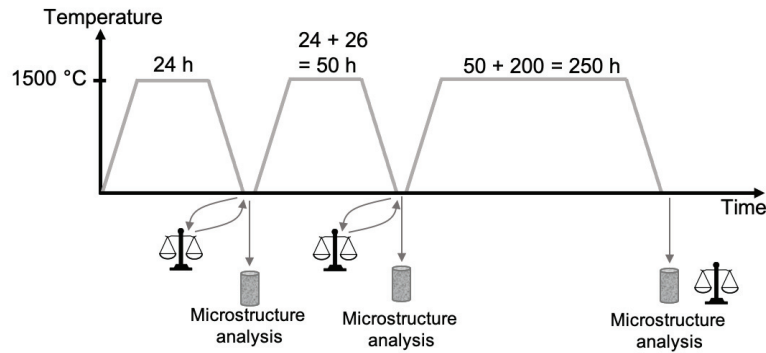
Figure 4.7: Schematic illustration of the oxidation cycle.
