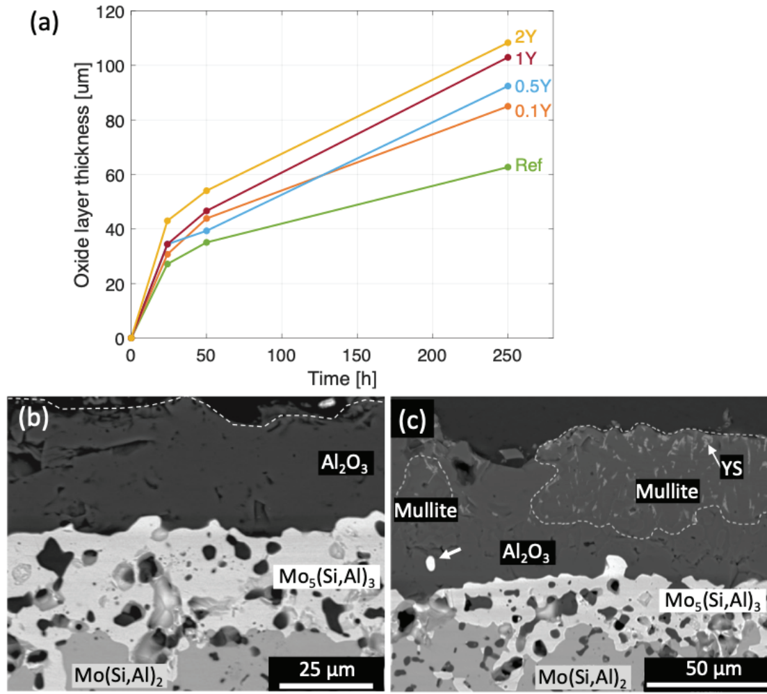
Figure 5.26: (a) Oxide thickness as a function of exposure time, (b) BSE image of the reference material, (c) BSE image of 2Y oxidised for 50 h at 1500 °C. A detached \text{Mo}_5(\text{Si,Al})_3 grain is indicated by the arrow.
