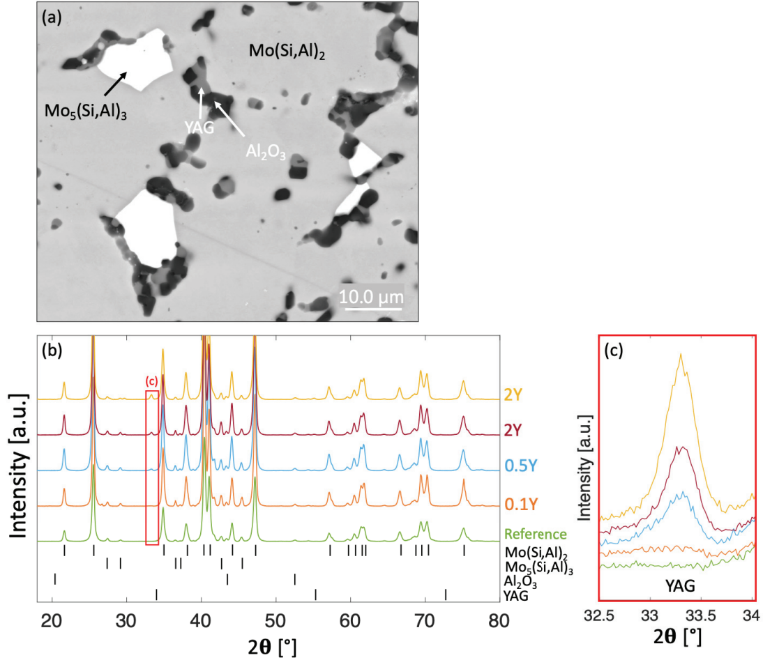
Figure 5.24: (a) BSE of the 2Y material, (b) LXRd diffractograms of the Y-alloyed \text{Mo}(\text{Si},\text{Al})_2 materials, (c) close up showing a YAG peak.
