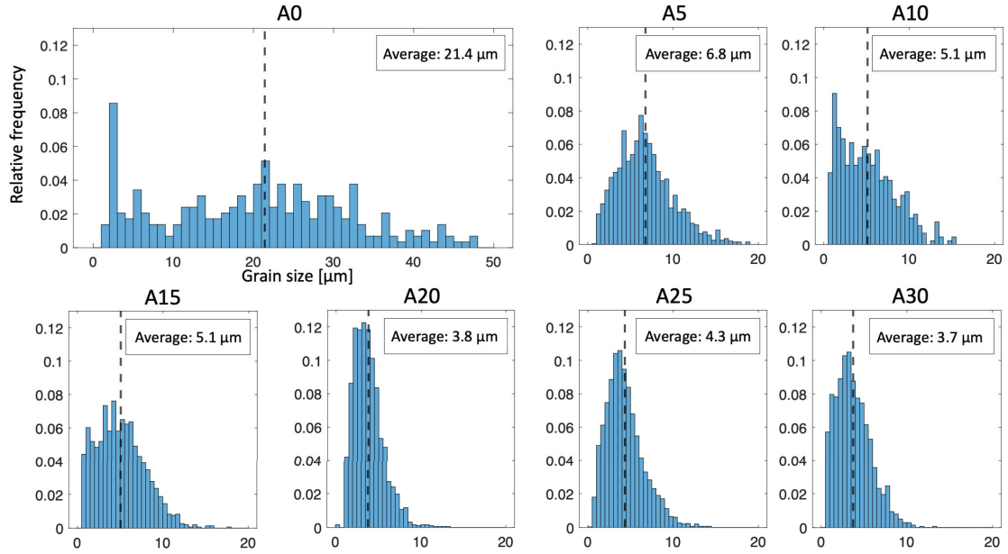
Figure 5.11: Grain size distribution of the as-sintered \text{Mo}(\text{Si,Al})_2\text{-Al}_2\text{O}_3 composites.
