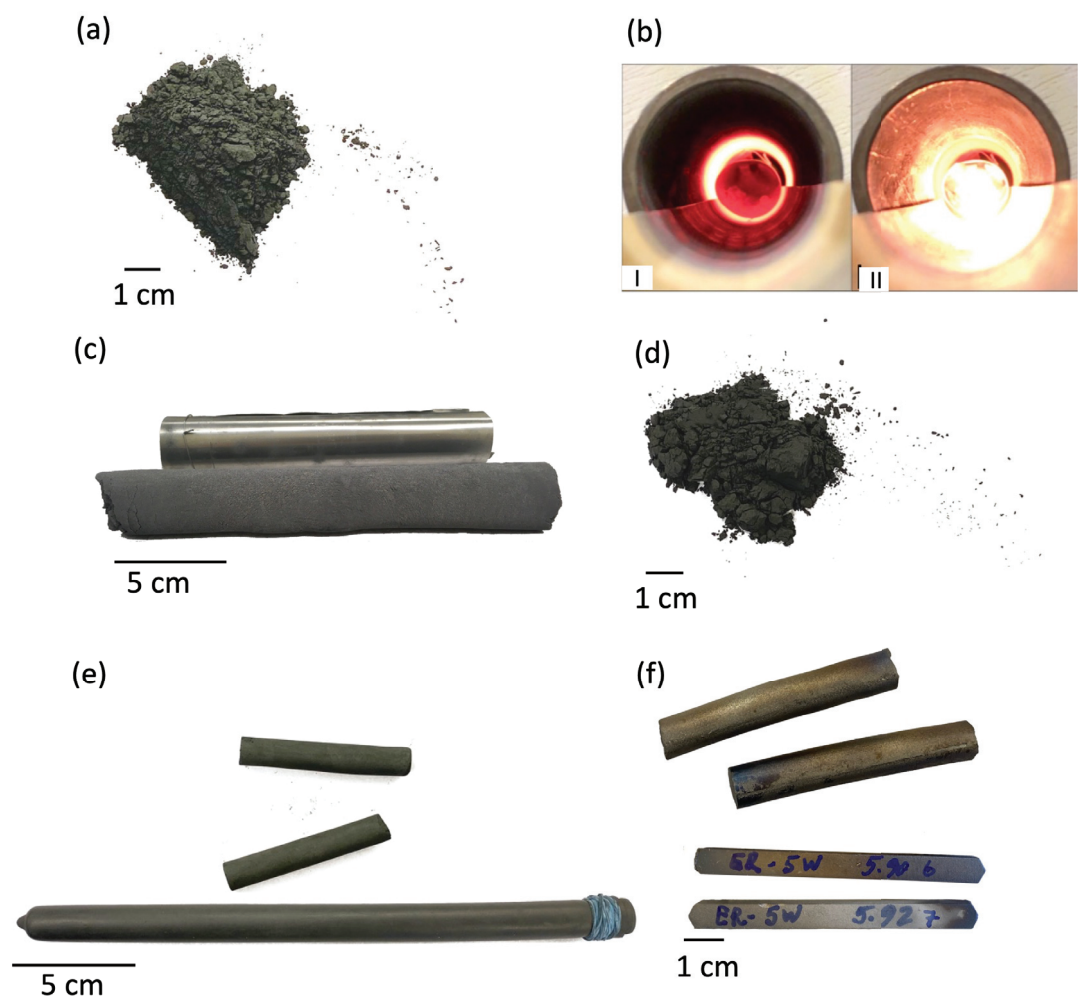
Figure 3.1: From powder to sintered material: (a) mixed powder before reaction, (b) powder before (I), and during (II), the self-propagating reaction in tube furnace, (c) cooled reaction product and Mo-cylinder, (d) reacted powder after milling, (e) CIP mould filled with powder and green bodies after compaction, (f) rod and rectangular Mo(Si,Al) 2 after sintering. The scale bars are approximate.
