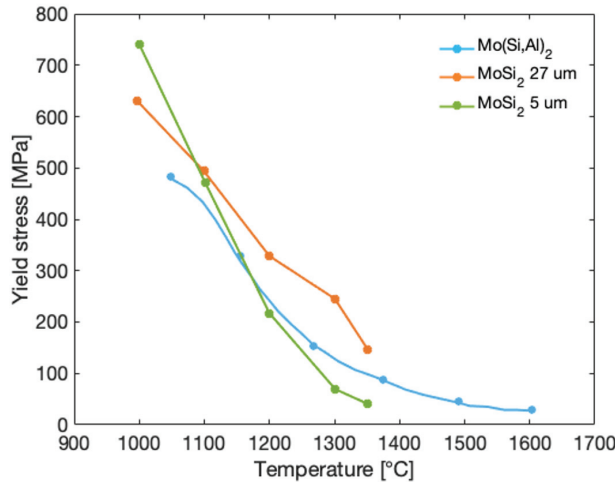
Figure 2.6: Temperature dependence of yield stress in polycrystalline Mo(Si,Al) 2 and MoSi 2 (grain size: 5 μm and 27 μm). The figure is based on data from [16] and [26].
