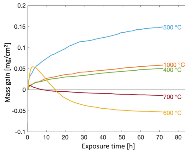
Figure 2.8: The mass gain as a function of exposure time for the \text{Mo}(\text{Si},\text{Al})_2 -based material exposed in synthetic air at different temperatures. Based on data from [52].
