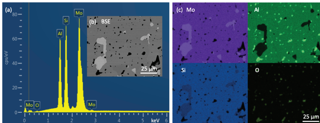
Figure 4.14: (a) Energy spectrum from \text{Mo}(\text{Si,Al})_2 , (b) BSE image, (c) EDS maps (Mo, Al, Si, and O) of the same region.
