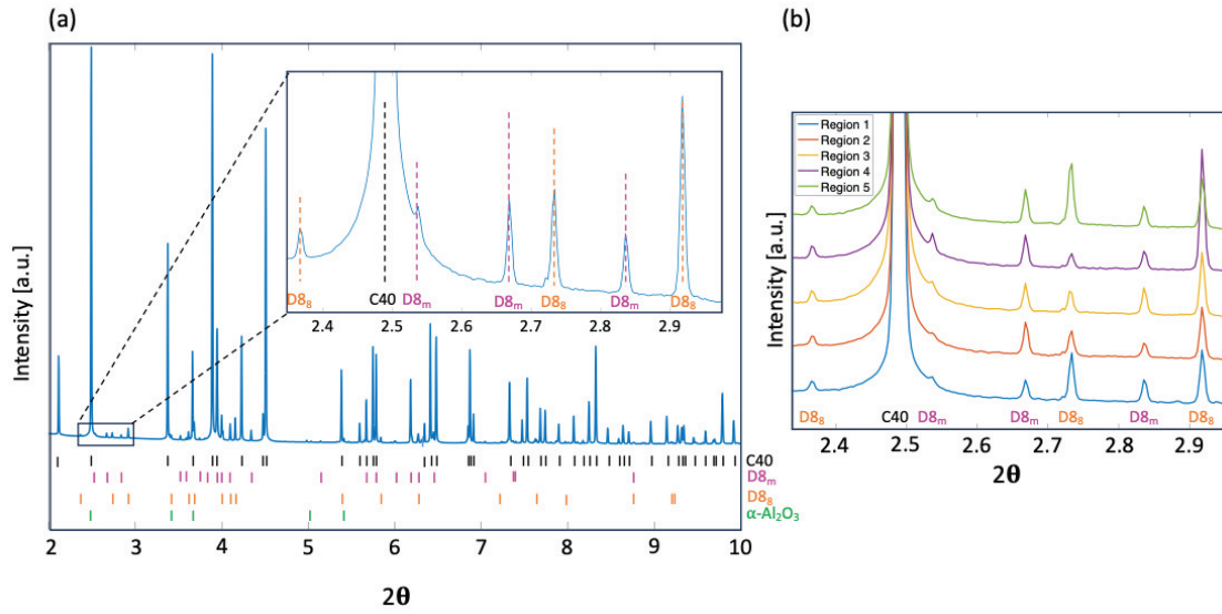
Figure 5.2: (a) SXR D pattern of the \text{Mo}(\text{Si},\text{Al})_2 material. The magnified region shows the presence of \text{D8}_m and \text{D8}_s , (b) the five individual SXR D patterns used to construct the SXR D pattern shown in (a).
