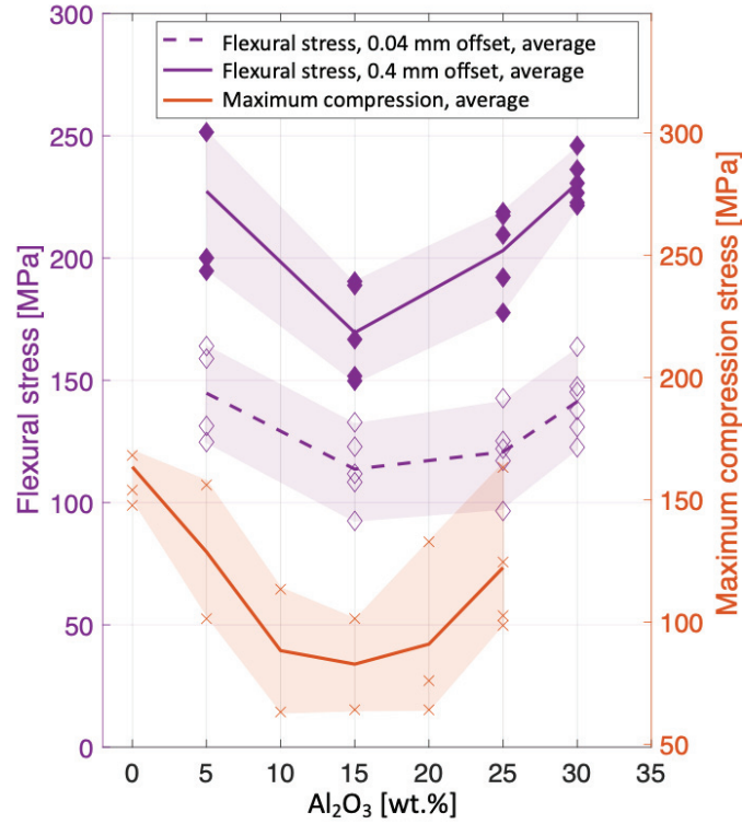
Figure 5.14: Maximum stress from compression testing, and flexural stress at 0.4 and 0.04 mm displacement from four-point bending testing of \text{Mo}(\text{Si},\text{Al})_2\text{-Al}_2\text{O}_3 composites.
