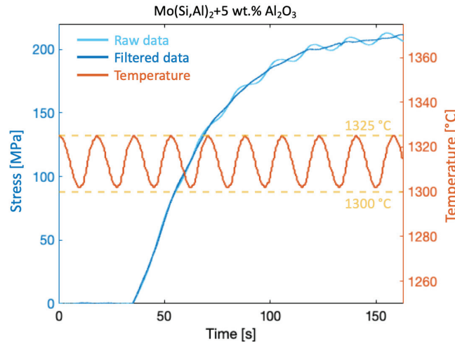
Figure 4.5: Temperature fluctuation and stress as a function of time in four-point bending of \text{Mo}(\text{Si,Al})_2\text{-Al}_2\text{O}_3 composite.
