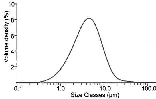
Figure 3.2: Particle size distribution of milled powder.
