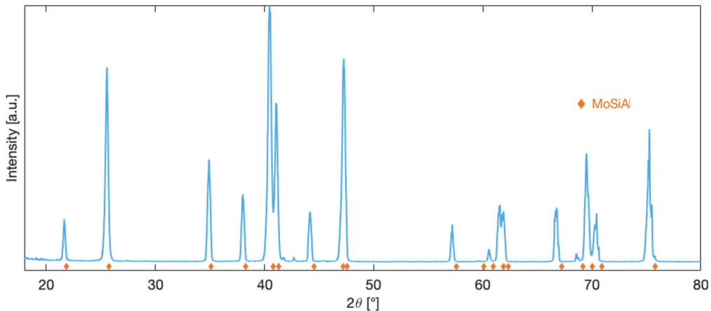
Figure 4.9: XRD pattern of a \text{Mo}(\text{Si},\text{Al})_2 material. The slight shift in 2\theta is due to small differences in the chemical composition of the analysed material and the material on which the XRD card was based (PDF 00-057-0374).
