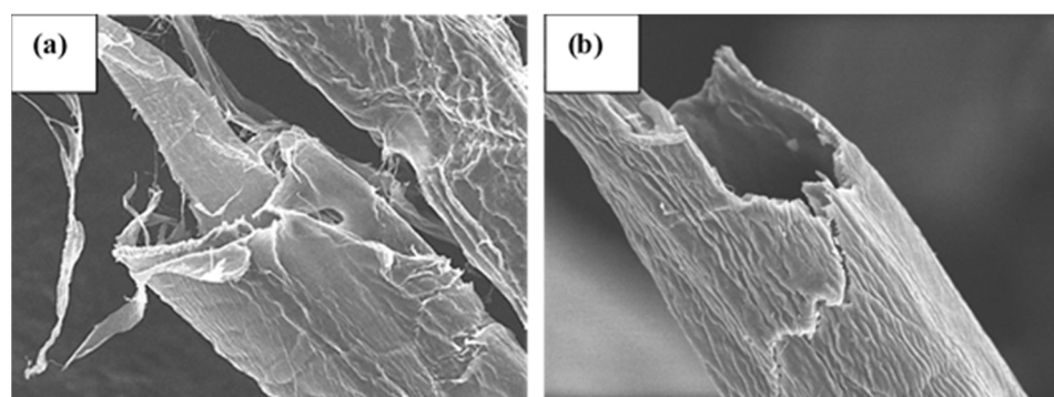
Figure 2. Scanning electron micrographs of fibers at a magnification of 2500: (a) pulp; (b) DAC with a degree of oxidation of 40%.
