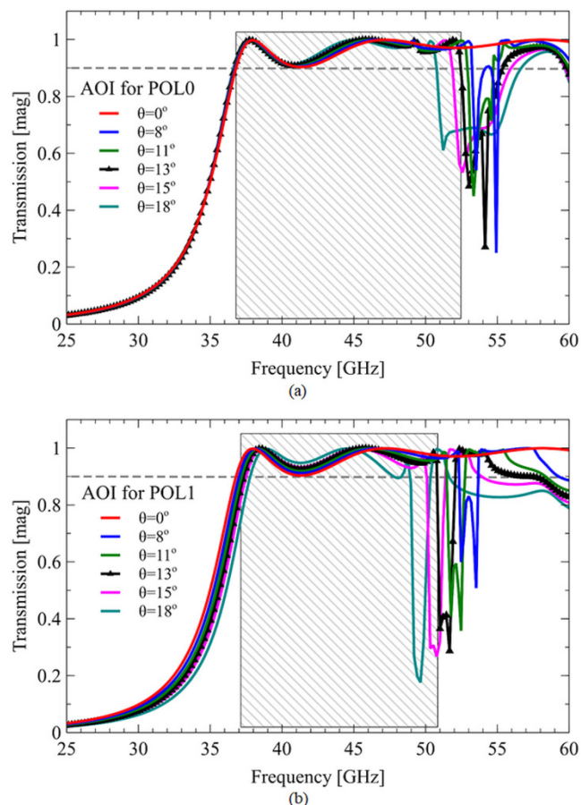
Fig. 4. The simulated transmission of the designed dichroic filter as a function of the frequency at various values of AOI: (a) for horizontally ( E_H ) oriented E-field (POL0); (b) for vertically ( E_V ) oriented E-field (POL1). The frequency ranges with transmission exceeding 90% at the design value of \theta=13 degrees, are indicated by the hatched areas. This transmission level is indicated by a grey dashed line.
