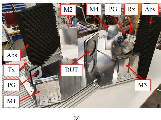
Fig. 7. The designed optical system for the characterizing the dichroic filter: (a) the schematic layout of the optical assembly, the grey-shaded volume represents the calculated quasi-optical beam indicating the path of the beam within the system; (b) a photograph of the measurement setup. The following components are marked: DUT – the dichroic filter; M1-M4 – ellipsoidal 1 focusing mirrors; PG – polarization grids; Tx and Rx – transmitting and receiving conical horns, respectively; Abs – absorber material.
