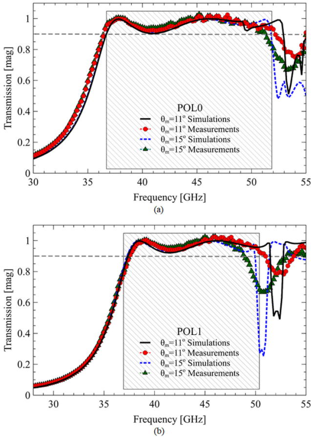
Fig. 9. Simulated and measurement results of the dichroic filter at nominal \theta=13 degrees and \Delta\theta=\pm 2 degrees: (a) for horizontally ( E_H ) oriented E-field (POL0); (b) for vertically ( E_V ) oriented E-field (POL1). The black solid and blue dotted lines depict the simulation results at \theta_m=11 and 15 degrees, respectively. The dash lines accompanied by red circles (at \theta_m=11 degrees) and green up-triangles (at \theta_m=15 degrees) represent the measured transmission data of the dichroic plate. The hatched area in the graph indicates the frequency range with measured transmission exceeding 90%, which is marked with a grey dashed line at \theta_m=\theta=13 degrees from Fig.8.
