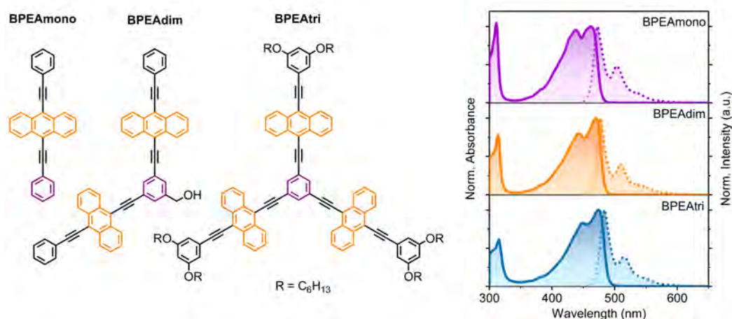
Figure 5.1: Molecular structures of BPEAmono , BPEAdim and BPEAtri together with their normalized steady state absorption and emission spectra.
