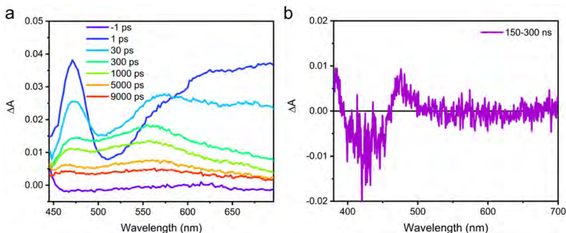
Figure 6.3: a) fsTA and b) nsTA spectra of DPIBF-C6 attached to ZrO 2 in toluene using an excitation wavelength of 405 nm.
