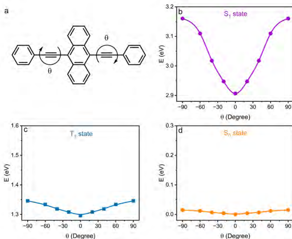
Figure 5.5: a) Molecular structure of BPEAmono indicating the dihedral angle \theta between the two phenyls and anthracene. Calculated energy of the b) S_1 c) T_1 and d) S_0 states as a function of \theta . Adapted from reference [135] with permission from the Royal Society of Chemistry. 135
