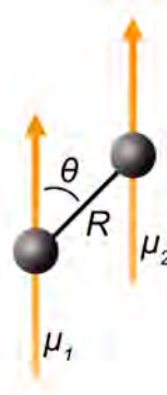
Figure 2.5: Illustration of the relative orientation of two TDMs in a J-aggregate \theta < 54.7^\circ and H-aggregate 54.7^\circ < \theta < 90^\circ .
