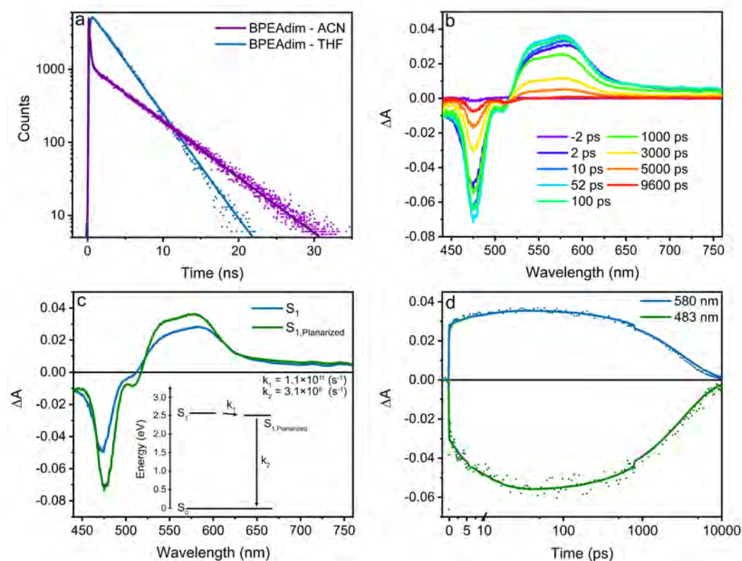
Figure 5.3: a) Time resolved emission of BPEAdim in ACN and THF obtained with \lambda_{ex} = 405 nm and monitored at 473 nm. b) fsTA analyses of BPEAdim in a dilute solution of THF ( \sim 10 \mu\text{M} ); excitation at 420 nm. c) Species associated spectra of the SVD analysis using the kinetic model shown in the inset. d) Selected kinetics of ground-state bleach and stimulated emission at 483 nm and S_1 excited state absorption at 580 nm with the model data shown as a solid line.
