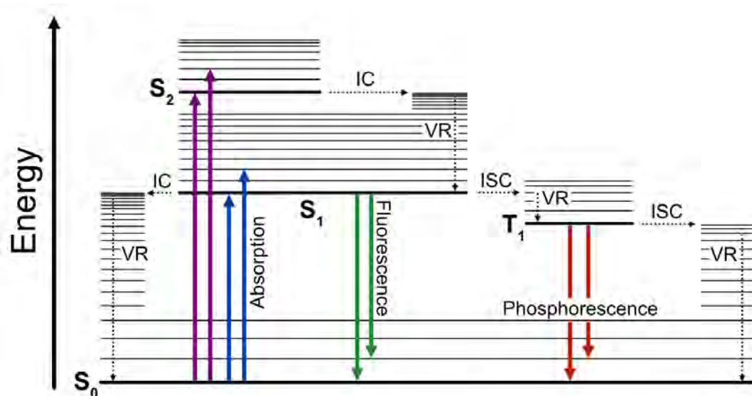
Figure 2.3: Jablonski diagram with singlet (S) and triplet (T) energy levels shown as horizontal lines. Thick lines depict the electronic levels and thinner horizontal lines are the vibrational levels. The diagram illustrates a selection of common photophysical processes such as absorption, fluorescence, phosphorescence, internal conversion (IC), vibrational relaxation (VR) and intersystem-crossing (ISC). Photoexcitation and radiative decay processes are marked as solid lines and non-radiative processes are marked as dotted lines.
