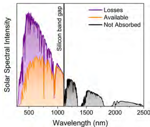
Figure 1.1: The solar spectrum at sea level. 6 The orange region represents the part of the solar spectrum that can be effectively harnessed by silicon. Below band gap photons can not be absorbed, leading to the losses marked as grey. The purple region represents the thermalization losses. 7
