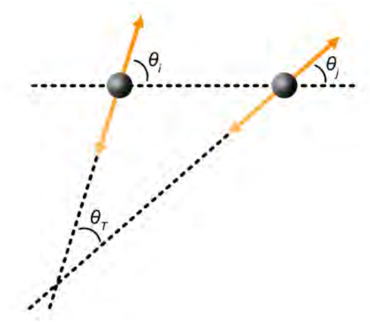
Figure 2.7: Illustration of the relative orientation of the TDMs and definition of the angles in Equation 2.8.
