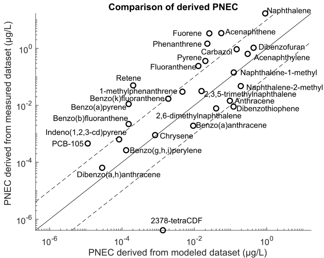
Figure 4-3. Comparison of 27 PNEC values ( \mu\text{g/L} ) derived from method 1 (only including experimentally measured ecotoxicological data) and scenario 2 (only including model output). The full line marks the 1:1 ratio and the dashed lines define one order of magnitude deviation. Substance names are indicated for each point.
