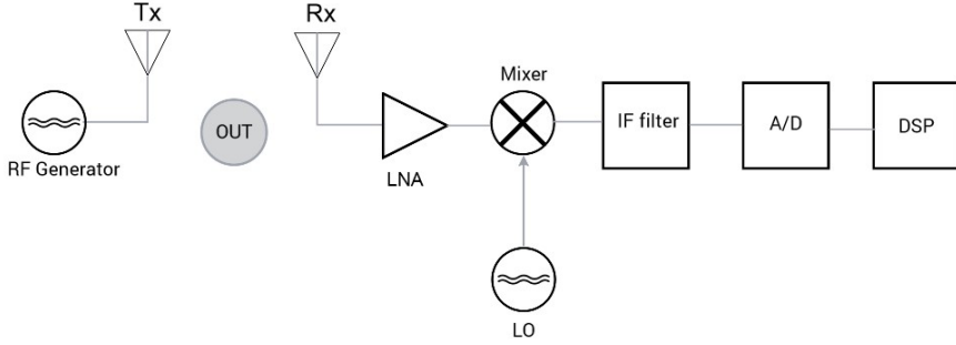
Figure 2.2: System architecture of VNA for microwave imaging.
