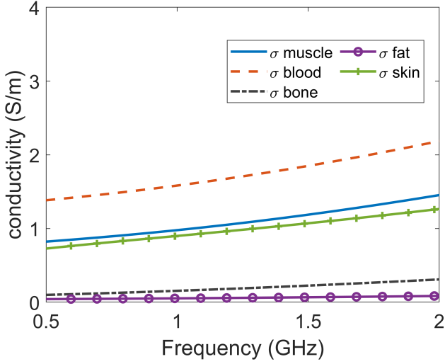
(b) Conductivity \sigma (S/m)
