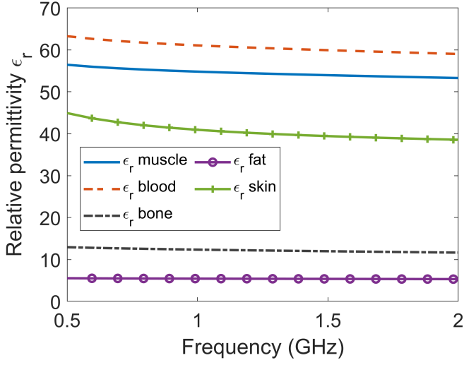
(a) Relative permittivity \epsilon_r
