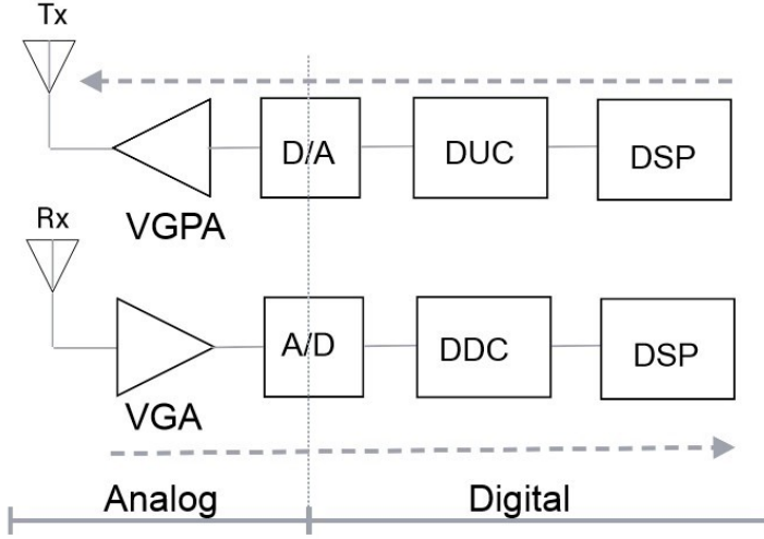
Figure 2.3: Simplified system architecture of SDR.
