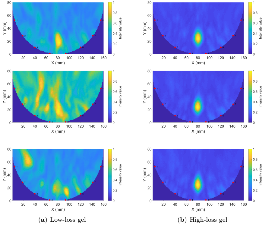
Figure 3.1: Sample reconstructions using phantom measurements: (a) low-loss gel; (b) high-loss gel. Taken from paper A.
