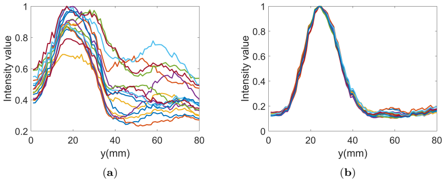
Figure 3.2: Reconstructed data along the line through the center of the imaging domain for 15 images: (a) low-loss gel; (b) high-loss gel. Taken from paper A.
