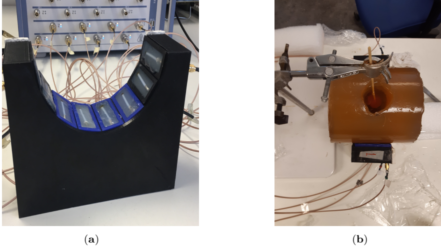
Figure 2.6: Measurement setup for probe measurements and image reconstruction: (a) semicircular antenna array consisting of 8 antennas; (b) muscle phantom in the antenna array, with probes taken from paper A.
