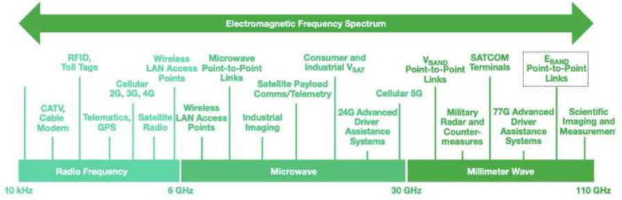
Figure 1.1: Millimeter wave spectrum overview. [5]
