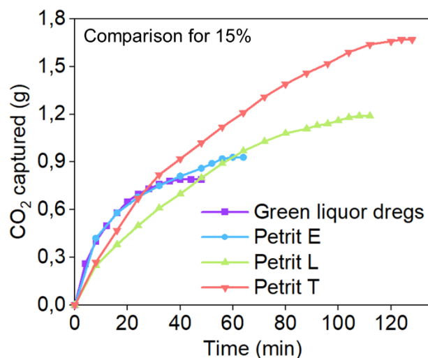
Figure 16. CO 2 captured evolution with time for all the materials at 15 w/v%.
