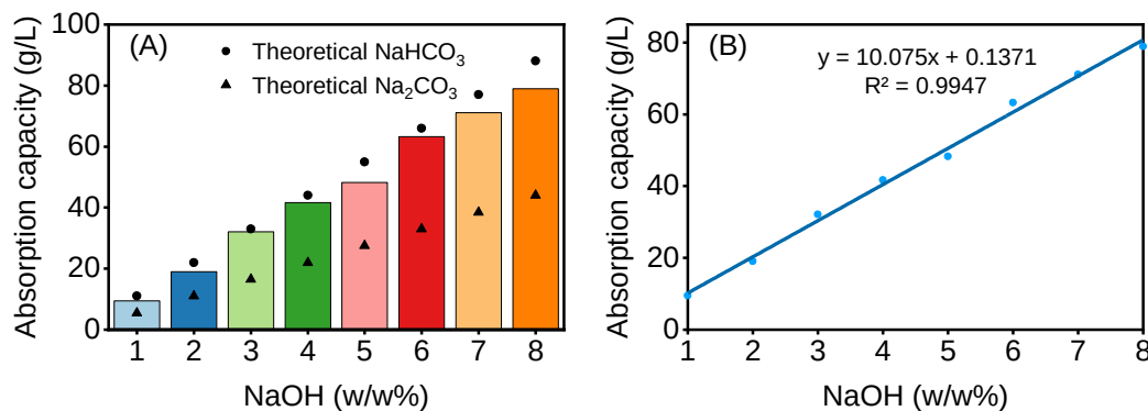
Figure 14. Obtained and theoretical absorption capacities for NaOH solutions of 1 to 8 w/w% NaOH. A total conversion of \text{CO}_2 to carbonate and \text{HCO}_3^- was assumed to estimate the theoretical capacities using Eq 3 and 5 (A). Linear regression based on the experimental data, indicating that the concentration of NaOH and the absorption capacity correlate linearly (B).
