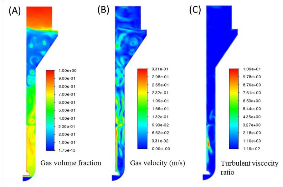
Figure 7. Contour plots of the gas volume fraction (A), gas velocity (B) and turbulent viscosity ratio (C) obtained from the CFD simulations.
