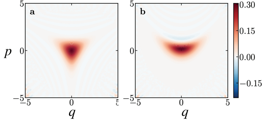
Figure 3.2: Wigner functions of (a) the trisqueezed state with triplicity t = 0.055 and (b) the target cubic phase state with squeezing parameter \xi_{\text{target}} = 0.5 and cubicity r = 0.05 .
