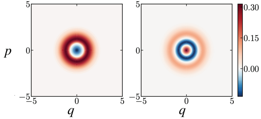
Figure 3.1: Wigner functions of (a) the one-photon state and (b) the two-photon state.
