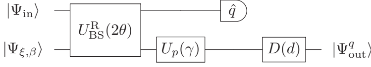
Figure 4.1: The circuit of our probabilistic Gaussian conversion protocol in Paper A. We start from two states and mix them in a beam-splitter U_{\text{BS}}^{\text{R}}(2\theta) . After a rotation U_p(\gamma) , we post-select the homodyne measurement on the first mode to value q = 0 and displace the second mode with D(d) .
