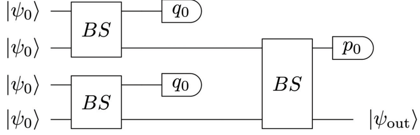
Figure 4.2: Sketch of our Gaussian conversion protocol with two iterations. Two binomial states |\psi_0\rangle are combined in a real balanced (50:50) beam-splitter. We then use a homodyne detector to measure the first modes' \hat{q} quadrature. In the second iteration, we instead measure the \hat{p} quadrature of one of the beam-splitter outputs.
