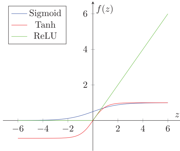
Figure 6.2: Common Activation Functions
