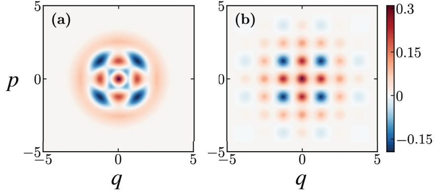
Figure 3.3: Wigner functions of (a) the binomial state with N = 2 and K = 3 , and (b) the target qunaght state in Paper B, with 4.95 dB effective squeezing.
