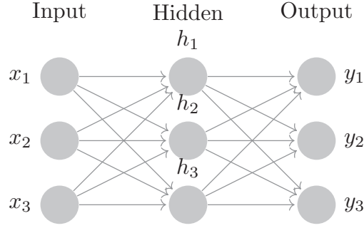
Figure 6.1: Illustration of a feedforward neural network with annotated neurons. The input layer neurons are denoted x_1, x_2, x_3 , the hidden layer neurons are h_1, h_2, h_3 , and the output layer neurons are y_1, y_2, y_3 .
