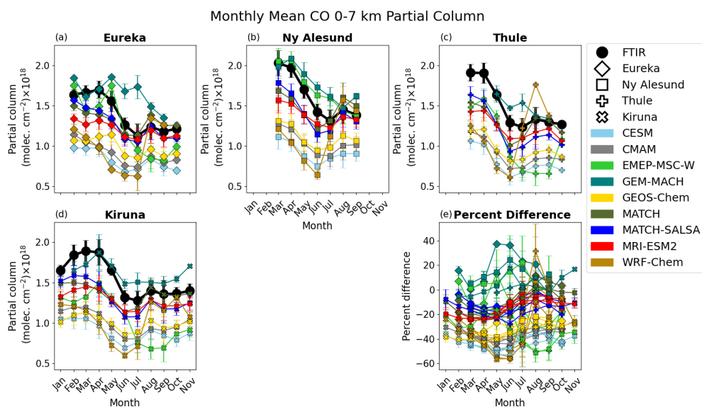
Figure 7. (a–d) Monthly mean FTIR (black) and smoothed model (colour) 0–7 km partial columns of CO ( \text{PC}_{\text{F,monthly},j} and \text{PC}_{\text{M,monthly},j} , respectively), for each location, shown with the same y axis. Error bars represent the standard deviation of the monthly mean. (e) Model–measurement mean percent difference by month ( \Delta_{\text{monthly},j} ) for each model (by colour) and location (by marker). Error bars represent standard deviation of the monthly mean percent difference.
