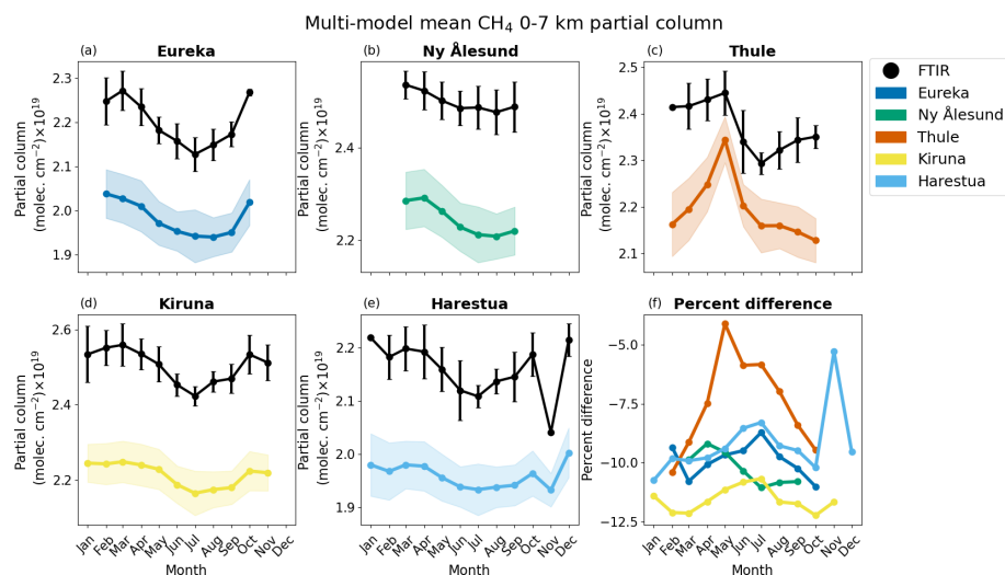
Figure 6. (a–e) Monthly mean FTIR (black) and multi-model mean (coloured) 0–7 km partial columns of \text{CH}_4 ( \text{PC}_{\text{F,monthly},j} and \text{PC}_{\text{MMM,monthly},j} , respectively), with error bars and shaded areas representing the standard deviation of the mean. (f) Monthly mean percent difference in the MMM ( \Delta_{\text{O,MMM}} ) for all locations.
