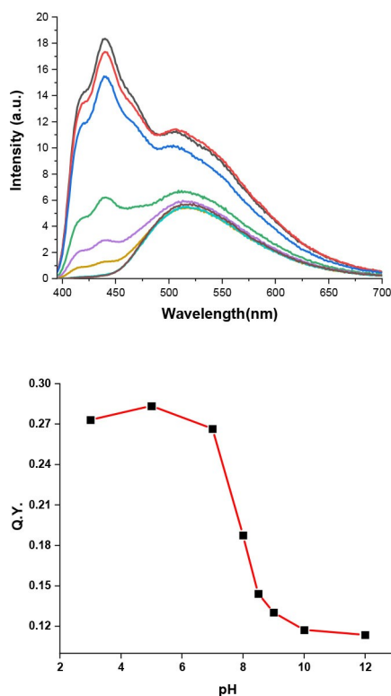
Figure 5. (Top) Emission spectra of qU recorded at different pH (pH 3, black; pH 5, red; pH 7, blue; pH 8, green; pH 8.5, violet; pH 9, dark yellow; pH 10, cyan; pH 12, wine), (bottom) Emission QY vs pH plot.
