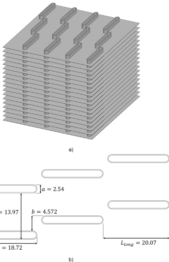
Fig. 4. (a) 3d representation of the 9.1–0.737-S finned flat tube heat exchanger geometry. In this image it features three banks of tubes ( N_{banks} ). (b) Cross-sectional view of the heat exchanger tube and their relative position to each other (units in millimeters).
