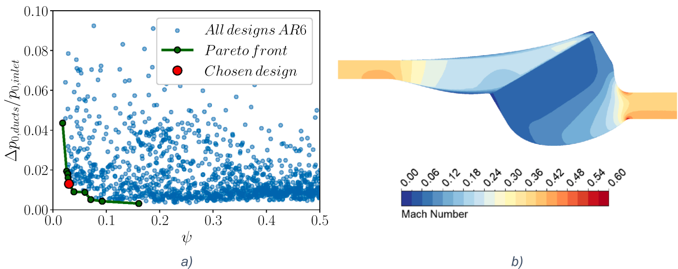
Fig. 13. (a) Pareto front for the ar6 optimization for the two objective functions, flow non-uniformity \psi and duct total pressure loss. (b) Chosen duct design (Case 1631) from the AR6 optimization and its Mach number distribution.
