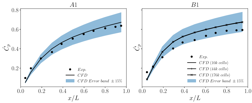
Fig. 11. Comparison between the computed and experimentally obtained averaged pressure coefficient, \widehat{C}_p = (\widehat{p} - p_{in})/q_{in} distributions for geometry A1 and geometry B1.
