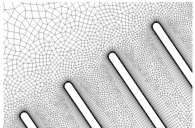
Fig. 22. Close-up of the mesh generated near the leading edge of the fins.
