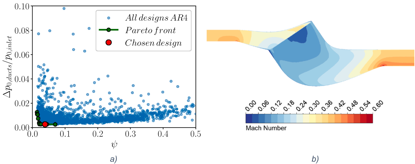
Fig. 12. (a) Pareto front for the ar4 optimization for the two objective functions, flow non-uniformity \psi and duct total pressure loss. (b) Chosen duct design (Case 1792) from the AR4 optimization and its Mach number distribution.
