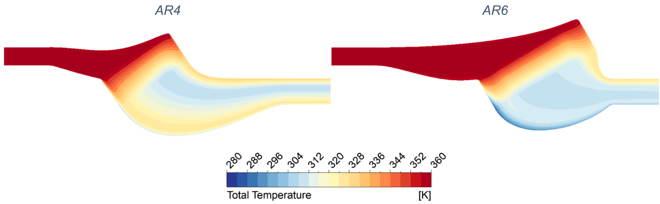
Fig. 14. Total temperature contour for the AR4 and AR6 duct designs.
