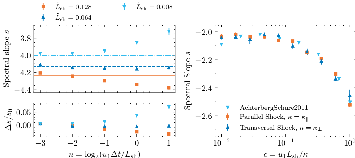
Figure 4. Left: Resulting spectral slope depending on the time step \Delta t in relation to the shock width L_{sh} . The upstream speed \tilde{u}_1 = 1 . The compression ratio is q = 2 , thus for an ideal shock we expect s = -4 . With larger shock widths, the shock produces steeper spectra as calculated by [52]. Slopes of the predicted stationary solutions are indicated by the colored lines for the respective shock width. Right: Resulting spectral slope depending on the ratio of upstream velocity and shock width to the diffusion coefficient. Data from [44] is shown for comparison. Here \tilde{u}_1 = 1 , q = 4 and \tilde{L}_{sh} = 0.004 with \Delta \tilde{t} = 0.001 is used while \kappa is varied. The free escape boundaries are \tilde{L}_{\pm} = 10 . With higher diffusion coefficient the spectral slope approaches the predicted value s = -2 . We already show the results for a transversal shock wave and taking perpendicular diffusion into account, which is discussed in section 4.1.
