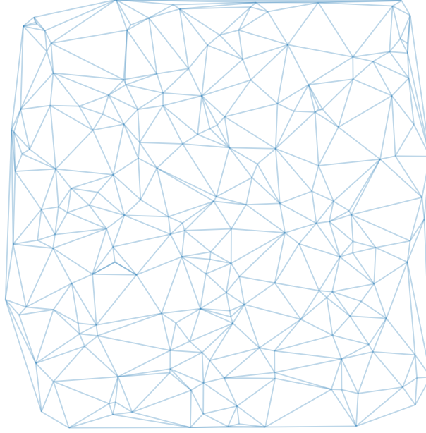
Figure 2.1: An example of a graph \mathcal{G}(\mathcal{V}, \mathcal{E}) , with lines representing edges between vertices.
