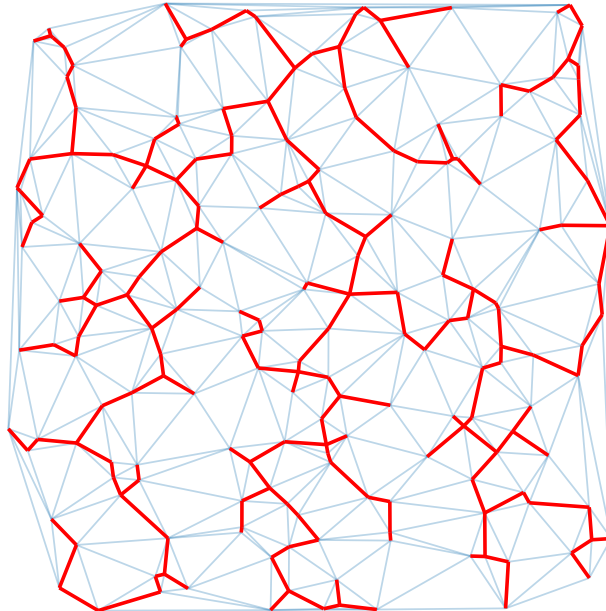
Figure 2.4: Minimum spanning tree (in red) of a weighted undirected graph \mathcal{G}(\mathcal{V}, \mathcal{E}, \mathbf{w}) , with the lengths of the edges (i.e., the Euclidean distance between the incident vertices of each edge) used as edge weights.
