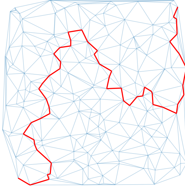
Figure 2.3: Minimax path (in red) through a weighted graph \mathcal{G}(\mathcal{V}, \mathcal{E}, \mathbf{w}) , with the lengths of the edges (i.e., the Euclidean distance between the incident vertices of each edge) used as edge weights.
