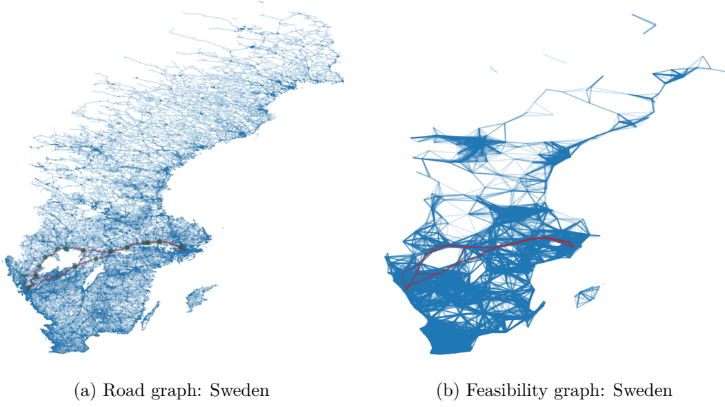
Figure 3.3: Road and feasibility graphs for Sweden, with Thompson sampling exploration of paths in red and charging stations in green, where the opacity indicates degree of exploration for both.
