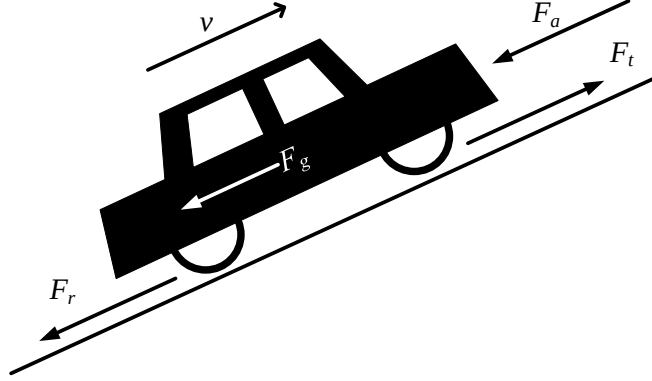
Figure 2.5: Longitudinal forces acting on a vehicle during motion.
