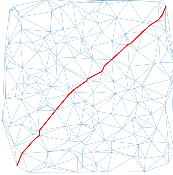
Figure 2.2: Shortest path (in red) through a weighted graph \mathcal{G}(\mathcal{V}, \mathcal{E}, \mathbf{w}) , with the lengths of the edges (i.e., the Euclidean distance between the incident vertices of each edge) used as edge weights.
