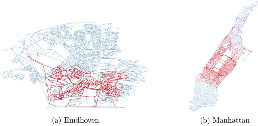
Figure 3.2: Exploration of minimax paths in Paper 2, using Thompson sampling (explored paths in red, with higher opacity indicating more visits).
