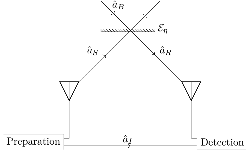
Figure 3.1: Schematic overview of the QI protocol. An entangled signal-idler pair is prepared. The signal mode \hat{a}_S is sent to interact with an unknown channel \mathcal{E}_\eta , modelled as a lossy Bosonic channel. From the channel the return mode \hat{a}_R is jointly measured with the retained idler \hat{a}_I , and a detection is declared if the detector finds sufficient statistical evidence that \eta > 0 . Otherwise the detector stays silent. [Reproduced from Fig. 2 of Paper I .]
