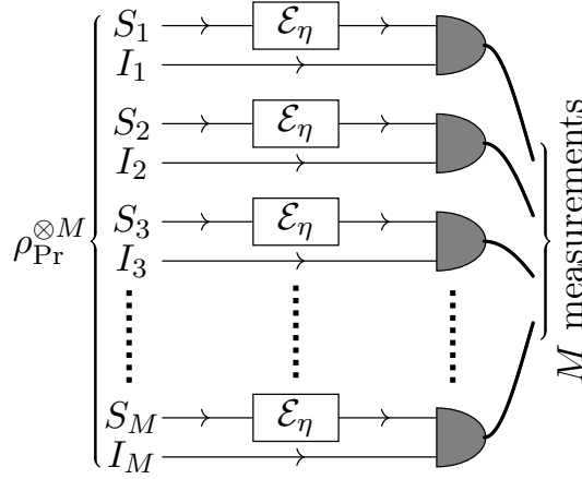
Figure 3.2: Illustration of M probes with respective entangled ancilla idlers are passed through the channel \mathcal{E}_\eta and then measured separately. The most general protocol would jointly measure all 2M modes. [Reproduced from Fig. 1 of Paper III .]
