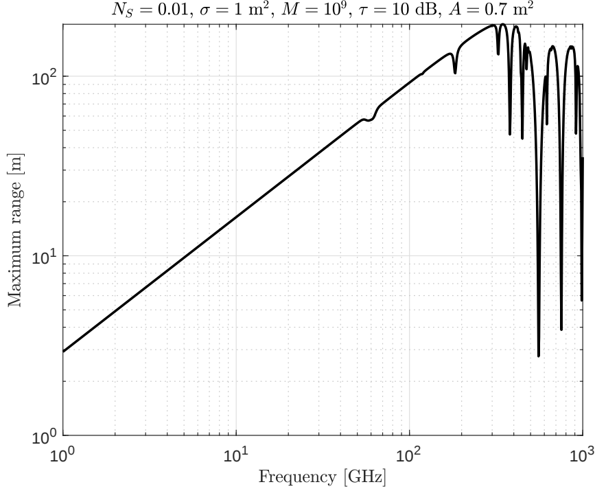
Figure 4.3: Example of maximum operating range of a quantum enhanced radar system with a fixed antenna size footprint of A = 0.7 \text{ m}^2 , a detection threshold of \tau = 10 and a target RCS of \sigma = 1 \text{ m}^2 . The benefit of operating at higher frequencies is explained by larger antenna directivity. The losses at frequencies larger than 300 GHz are due to significant atmospheric attenuation. [Reproduced from Fig. 1 of Paper II ]
