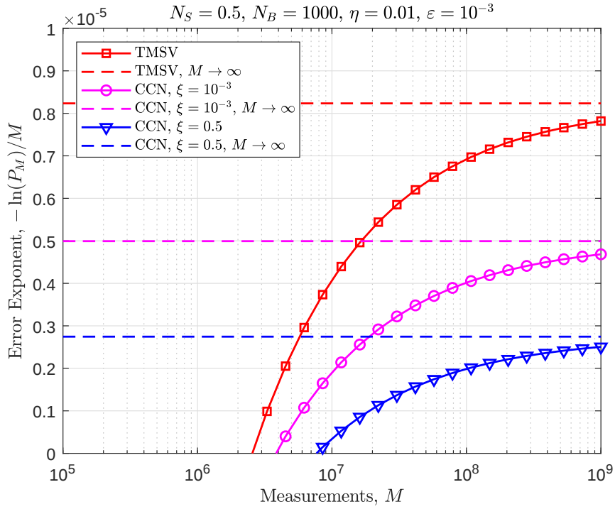
Figure 4.2: Semi-asymptotic behaviour of the error exponent with increasing number of repeated trials. The TMSV state probe outperforms the optimized CCN probe, illustrating together with Fig. 4.1 how double heterodyne measurement is non-ideal. Here, \xi refers to the balance parameter \beta in the text. [Reproduced from Fig. 5 of Paper I. ]
