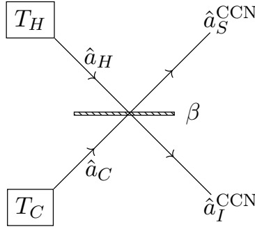
Figure 2.1: Overview of how two correlated thermal modes can be generated by mixing two independent thermal modes on a \beta -parametric beamsplitter. If the two thermal sources have different average number of photons N_H \neq N_C , the output modes will be correlated. [Reproduced from Fig. 1 of Paper I .]
