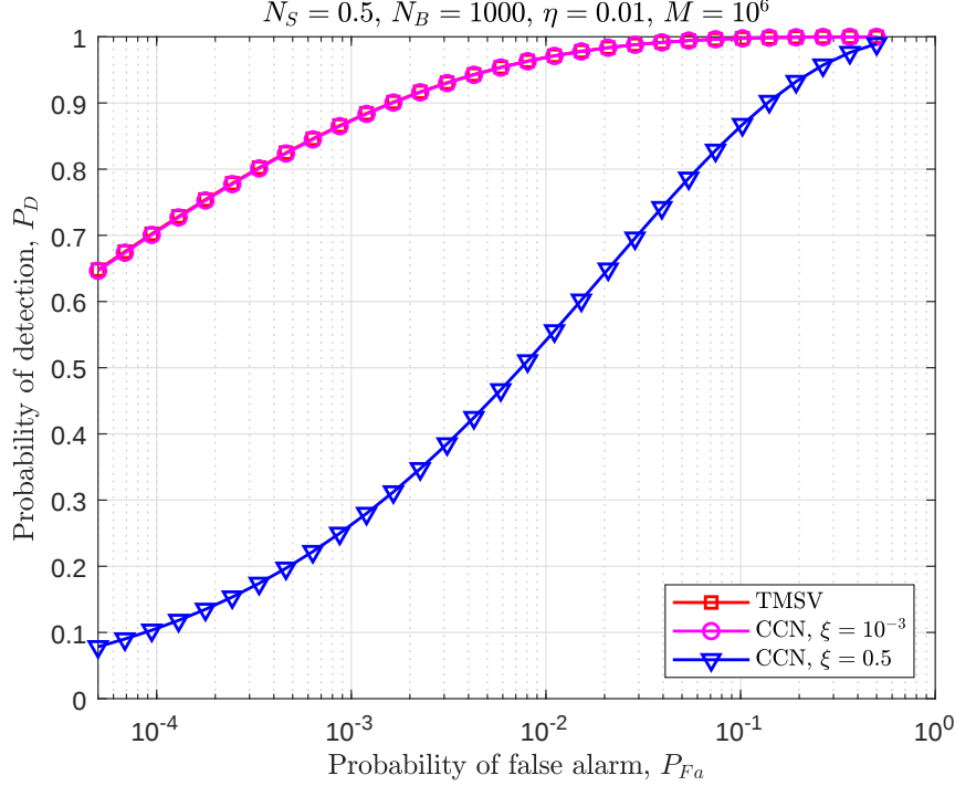
Figure 4.1: Receiver Operating Characteristic for the TMSV state probe and CCN state probe given ideal heterodyne detection of the return- and idler mode. Here, \xi refers to the balance parameter \beta in the text. [Reproduced from Fig. 4 of Paper I. ]
