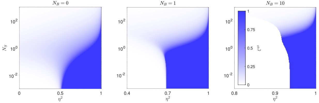
Figure 4.4: Optimal trade-off of between squeezing ( \xi = 1 ) and displacement ( \xi = 0 ) for the single-mode QFI for three different average numbers of background photons. For finite background ( N_B > 0 ) and few probe photons ( N_S \lesssim 1 ), a sharp transition between coherent state and squeezed vacuum being the optimal state is observed at low signal brightness. [Reproduced from Fig. 2 of Paper III .]
