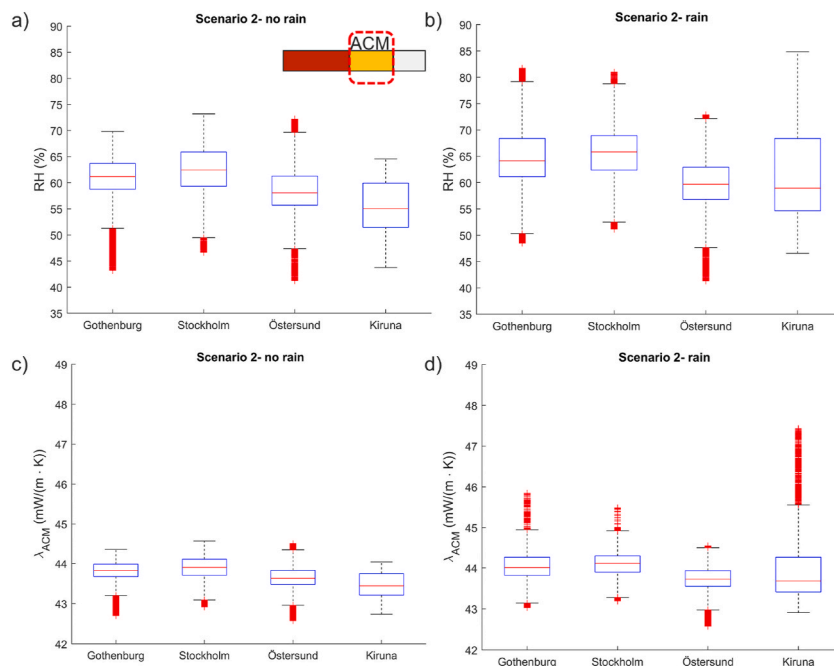
Fig. B 3. a,b: Simulated average RH in the layer of ACM. c,d: Calculated moisture-dependent thermal conductivity of the ACM. Left: No rain. Right: Rain.
