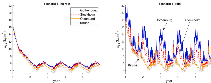
Fig. 10. Simulated water content in the test wall with ACM-system in various locations. Left: No rain. Right: Rain.
