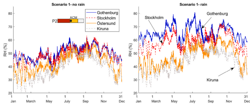
Fig. 11. Simulated RH at the interface between the ACM and brick (P2), corresponding to the last year of simulations for all four cities. Left: No rain. Right: Rain.
