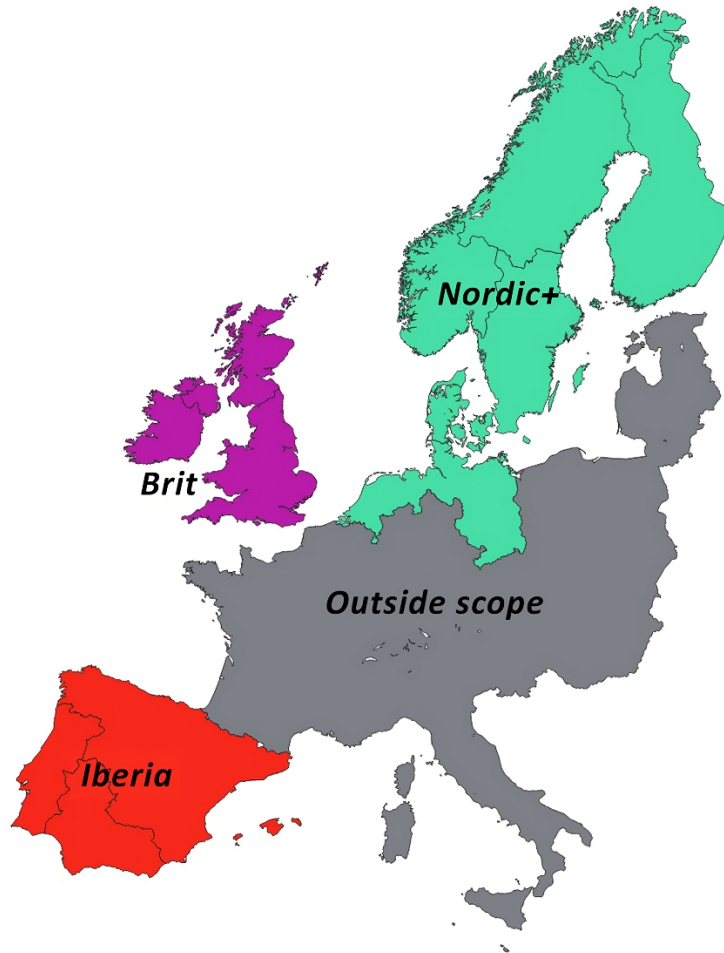
Figure 3. Map illustrating the three regional cases applied in Papers II and III with respect to existing generation and transmission capacities, VRE potentials and generation profiles, and electricity loads and load profiles. Brit: England plus Wales, Scotland, Northern Ireland, and Ireland; Iberia: north-eastern Spain, south-western Spain, and Portugal; Nordic: Finland, northern Sweden + northern Norway, southern Norway, southern Sweden + eastern Denmark, and Netherlands + western Denmark + north-eastern Germany.
