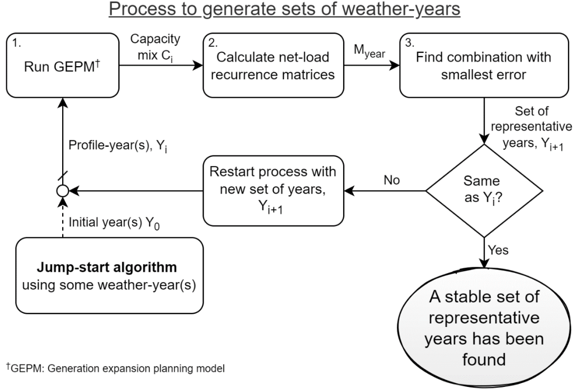
Figure 6. Flowchart illustrating the algorithm for finding a set of weather-years that represents the net-load variations in the 40-year period of 1980–2019.
