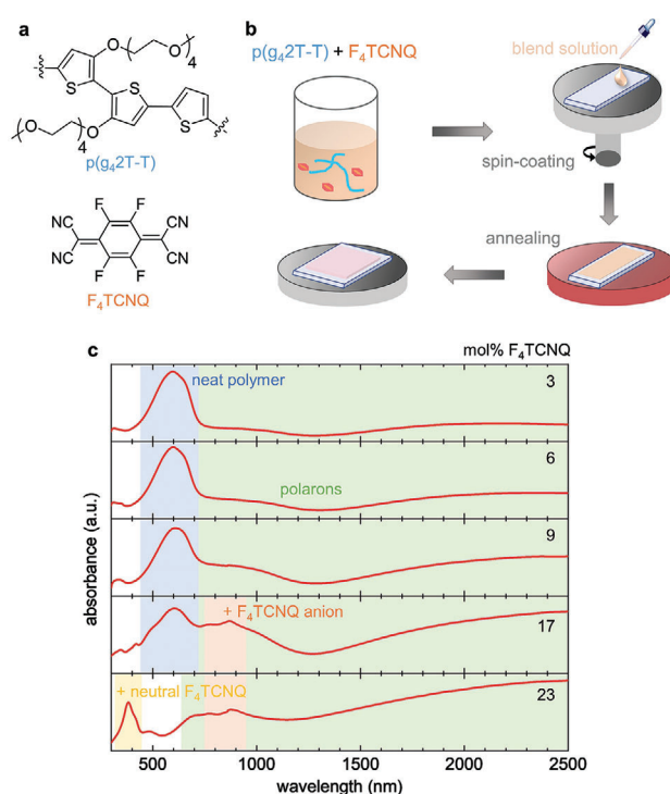
Figure 1. Co-processing of doped polymer films. a) The chemical structures of p(g_42T-T) and F_4\text{TCNQ} ; b) schematic of solution co-processing; c) UV-vis-NIR absorption spectra of co-processed p(g_42T-T):F_4\text{TCNQ} thin films with a thickness of 90–160 nm; highlighted areas correspond to the absorption peaks of neat polymer (blue), polarons (green), F_4\text{TCNQ} anions (red), and neutral F_4\text{TCNQ} molecules (yellow).
