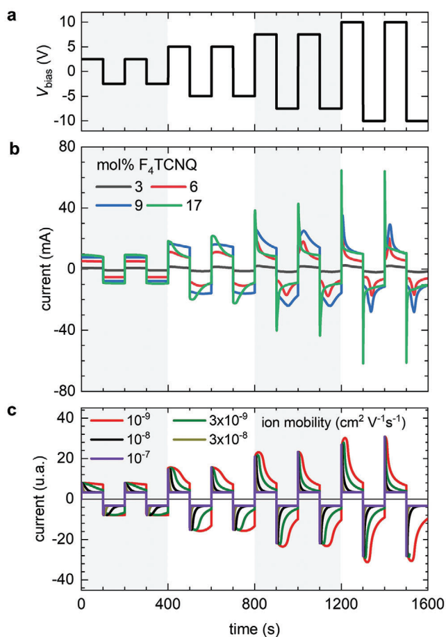
Figure 2. Current transients during electrical programming of doping gradients. a) Bias voltage V_{bias} applied between the inner electrodes; b) current between the outer electrodes at various constant V_{bias} of alternating polarity for p(g 4 2T-T) films doped with 3 to 17 mol% F 4 TCNQ; and c) simulated current transients during electrical programming of doping gradients for different mobilities of the dopant ions.
