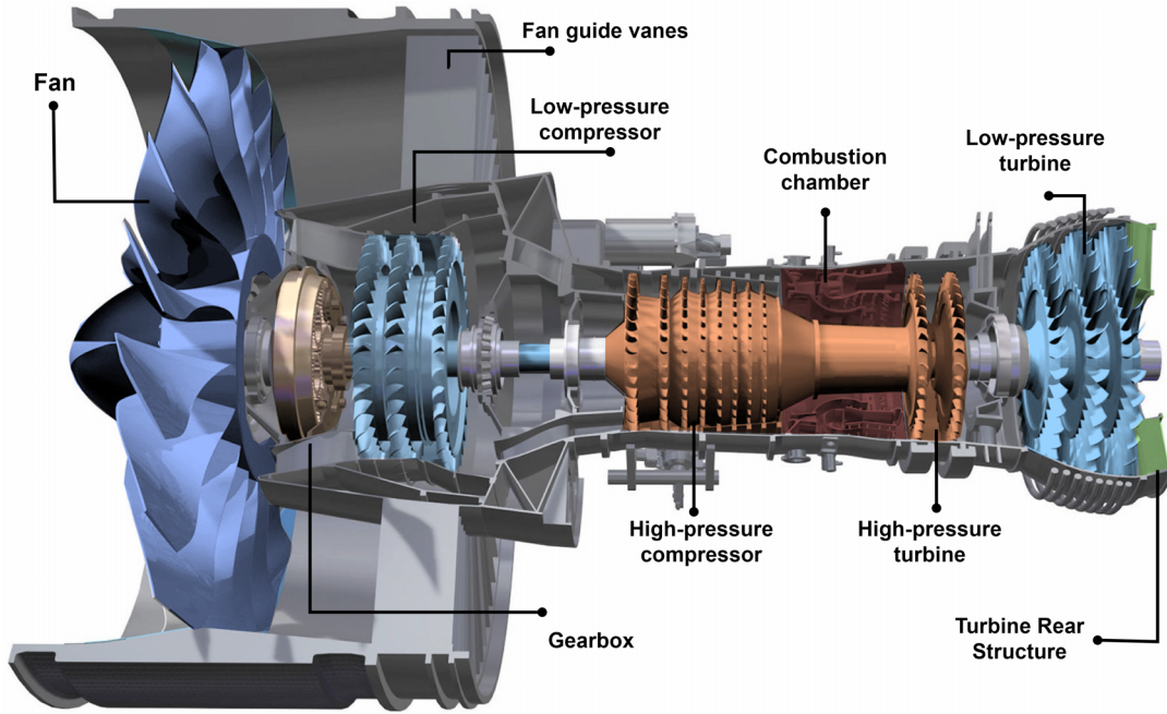
Figure 1.2: Schematic representation of the PW1100G's internal configuration. Adapted from [22].
