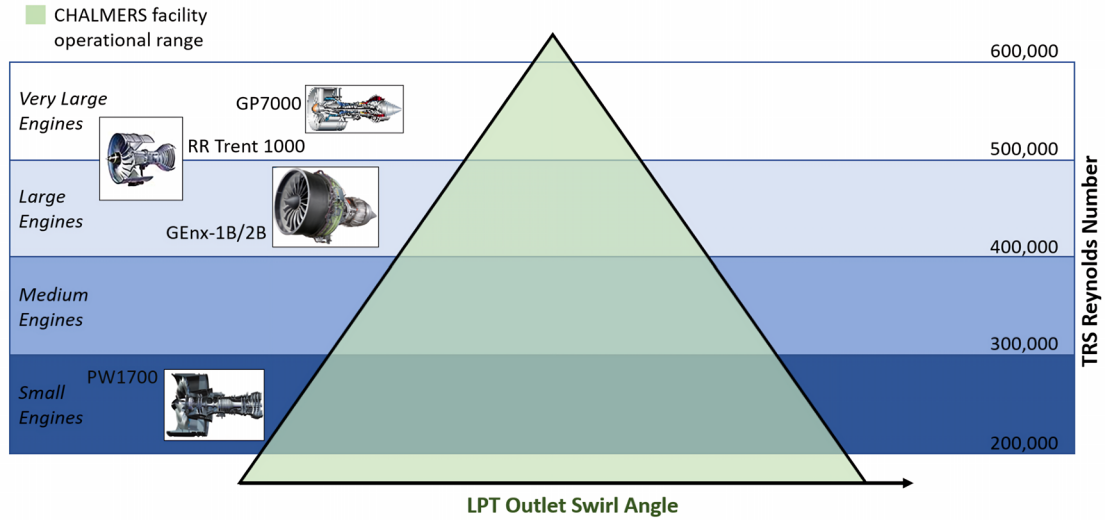
Figure 2.3: Chalmers LPT-OGV test facility operational space. Adapted from [44].
