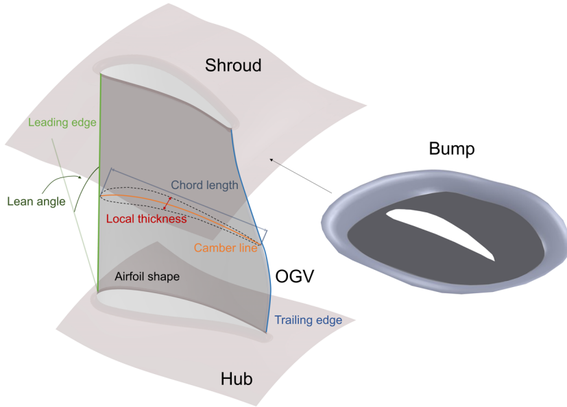
Figure 1.4: A 3D model of OGV with primary OGV nomenclature, hub, shroud and bump surfaces.
