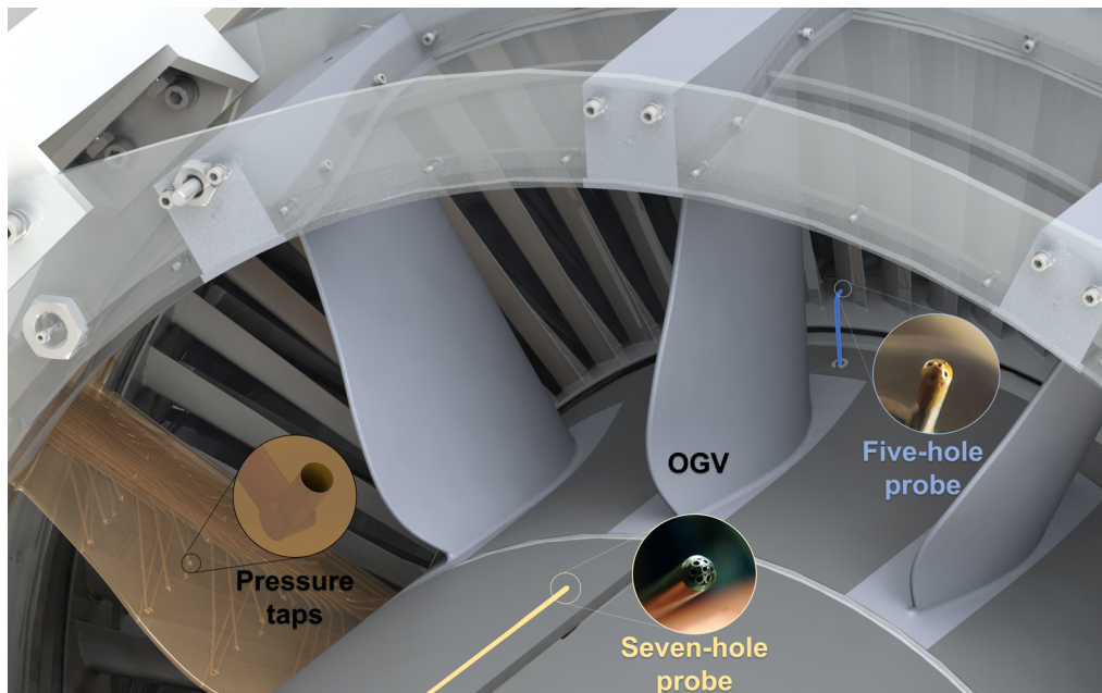
Figure 3.1: Isometric view of the test section with instrumented 5- and 7-hole aero probes and OGV with integrated pressure taps.
