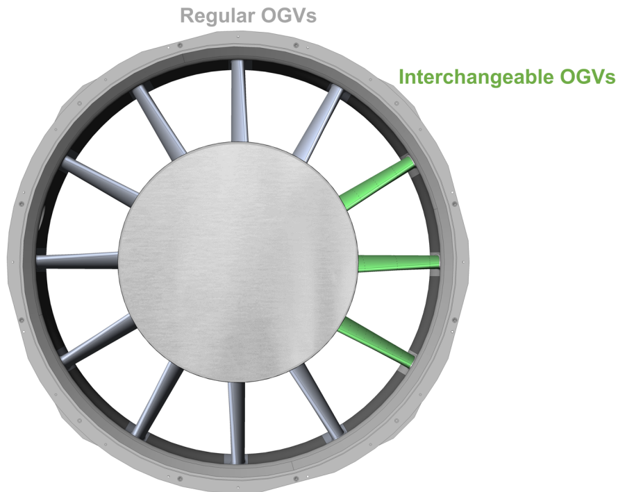
Figure 2.5: Baseline (C1) TRS configuration with instrumented interchangeable OGVs.
