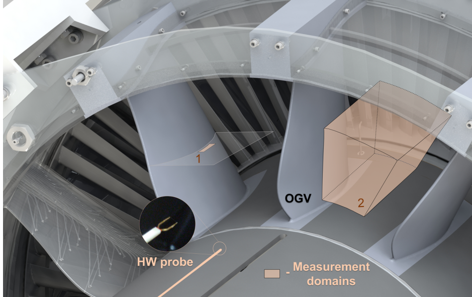
Figure 3.3: Isometric view of the test section with measurement domains for hot-wire measurements: 1 – boundary layer measurements; 2 – volume measurements between OGVs.
