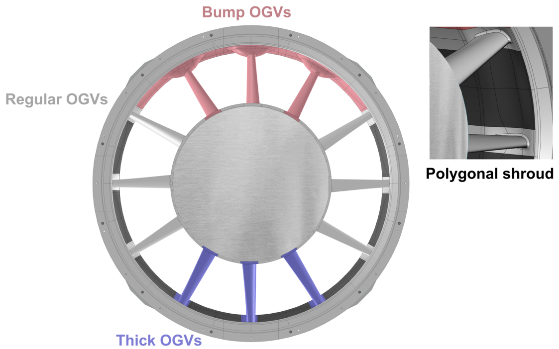
Figure 2.8: State-of-the-art TRS configuration with polygonal shroud and three types of OGVs: regular, thick and bump.
