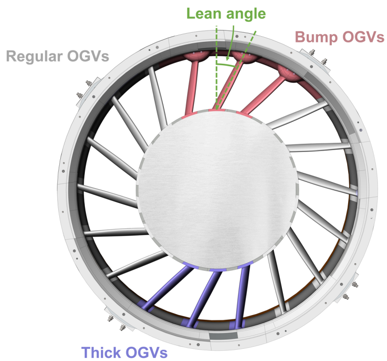
Figure 2.9: State-of-the-art TRS configuration with three types of leaned OGVs: regular, thick and bump.
