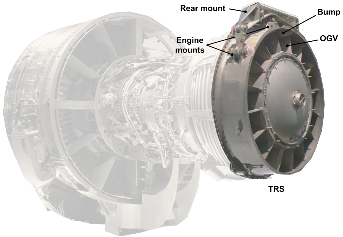
Figure 1.3: Rear view of a CFM56-5 aero engine. Adapted from [23].
