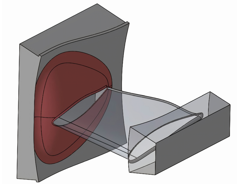
Figure 2.7: A 3D model of OGV with a mount bump marked with red.
