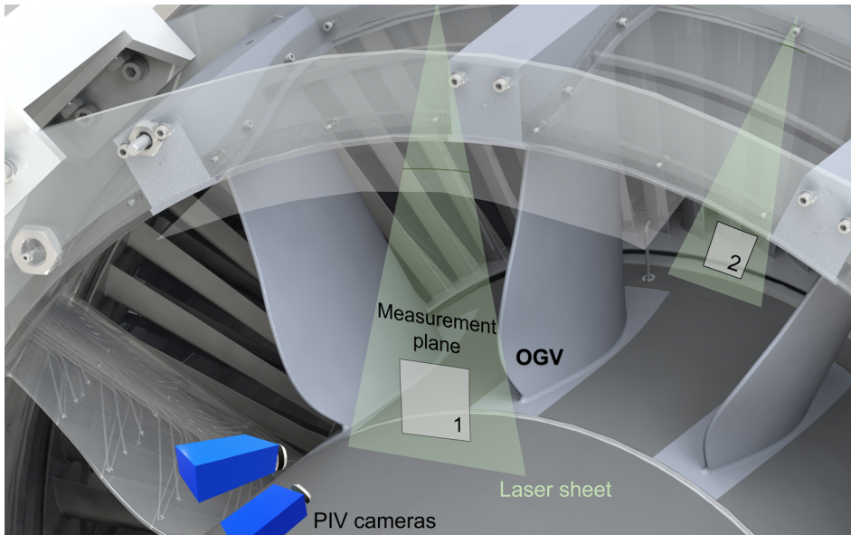
Figure 3.4: Isometric view of the test section with PIV cameras, measurement and laser planes: 1 – downstream plane in the OGV wake region; 2 -upstream plane.
