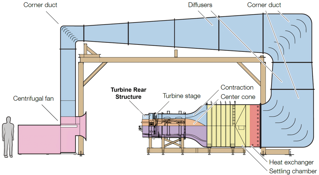
Figure 2.1: Chalmers LPT-OGV facility. Adapted from [45].
