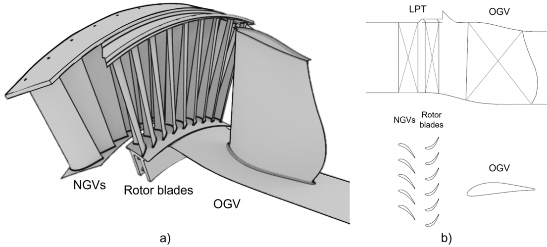
Figure 2.2: The schematic of LPT and TRS: (a) isometric view (b) meridional view with midspan profiles.
