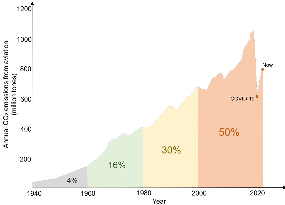
Figure 1.1: Annual global CO 2 emissions from aviation (1940-2023) with % of total cumulative emissions broken down into 20 year periods . Adapted from [2].
