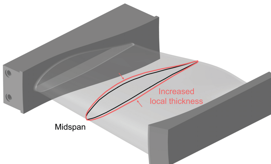
Figure 2.6: A 3D model of a thick OGV with midspan profile (solid red line) compared to regular vane midspan profile (solid black line)
