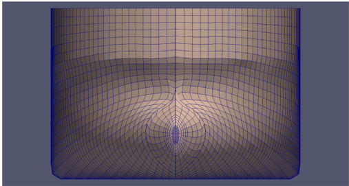
Fig. 6. Bow view of hull mesh with approximately 7000 panels.
