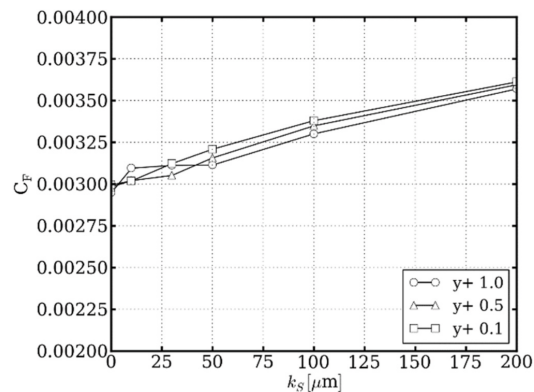
Fig. 4. y^+ sensitivity for EASM turbulence model with Auupoix-Colebrook roughness model at Re = 6.9 \times 10^6 .
