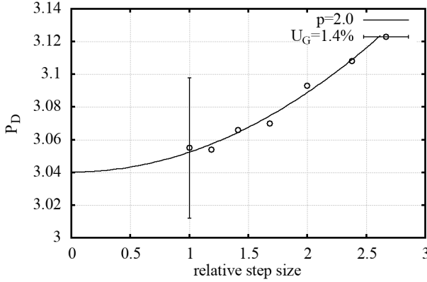
Figure 3.2: RANS grid convergence of delivered power, full-scale.
