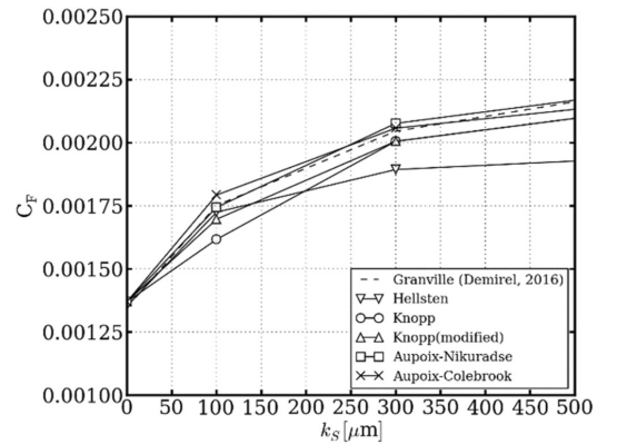
Fig. 19. Roughness model comparison for a flat plate at \text{Re} = 2.89 \times 10^9 , EASM, k_s range 0–500 \mu\text{m} .
