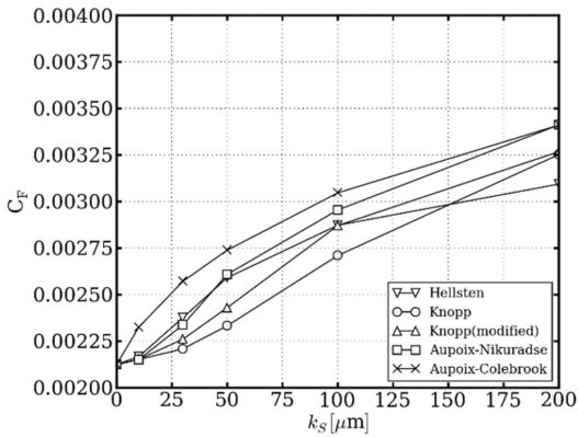
Fig. 16. Frictional resistance coefficient at \text{Re} = 7.6 \times 10^7 , EASM.
