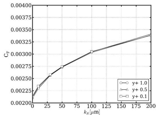
Fig. 5. y^+ sensitivity for EASM turbulence model with Auupoix-Colebrook roughness model at Re = 7.6 \times 10^7 .
