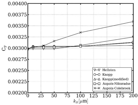
Fig. 15. Frictional resistance coefficient at \text{Re} = 6.9 \times 10^6 , EASM.
