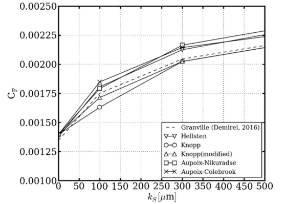
Fig. 17. Roughness model comparison for a flat plate at \text{Re} = 2.89 \times 10^9 , k-\omega SST, k_s range 0–500 \mu\text{m} .
