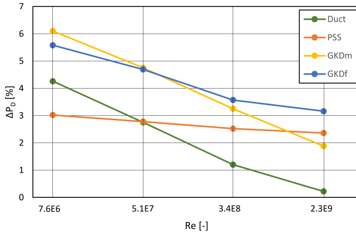
Figure 3.11: Power reduction by Duct, PSS and optimized GKD at different Reynolds numbers.
