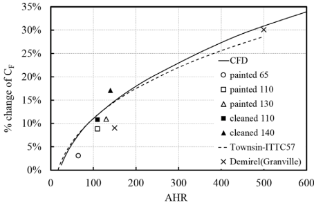
Fig. 6. Comparison of CFD simulations ( AHR/k_S = 5 ) with Granville/Grigson extrapolated rough flat plates and Townsin estimated increase of C_F . KCS conditions, L = 230 m, Rn = 2.89 \times 10^8 .
