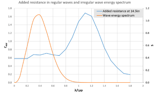
Fig. 16. Irregular wave energy spectrum and ship added resistance coefficient in regular head waves at 14.5 knots.
