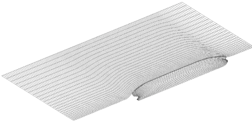
Fig. 3. Free surface and hull meshes used in XPAN simulations.
