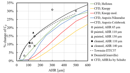
Fig. 26. Comparison of extrapolated measured values, simulations with correlation factor 5, and Townsin's formula for a flat plate at Re = 2.89 \times 10^9 .
