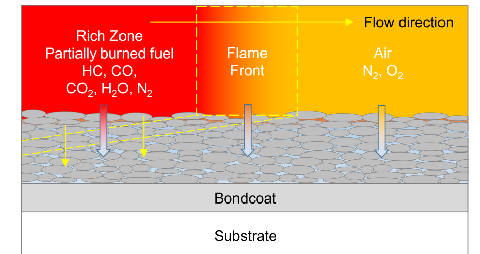
Figure 13. Entrainment of partially burned fuel from the core of the jet and flame front into the porous TBC during compression and combustion.
