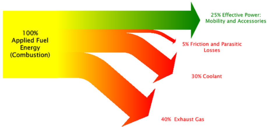
Figure 1. Engine energy flow distribution; typical coolant losses are between 20 to 35% of the total fuel energy.
