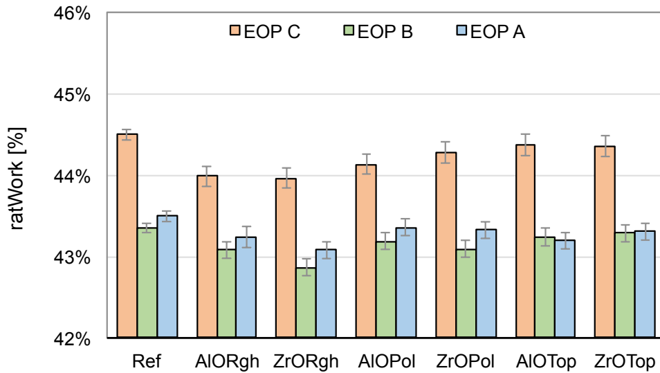
Figure 27. Estimation of the indicated efficiency from the modeled data. No EGR for EOP A and B, high rail pressure level for EOP C. Error bars show the 95% CI.
