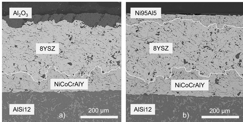
Figure 24. Electron microscope images of the TBC with a) alumina and b) nickel alloy sealing layers. The white lines at the interfaces are added for clarity.
