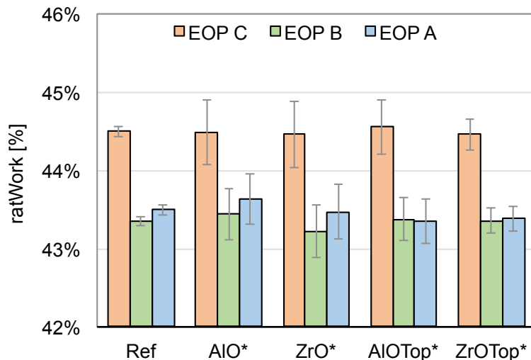
Figure 28. Predicted indicated efficiency (ratWork) with R_a = 1.3 \mu\text{m} , CR = 15.5 for all pistons. The error bars show 95% CI. The stars on the labels mark that these are predictions for coatings with modeled properties.
