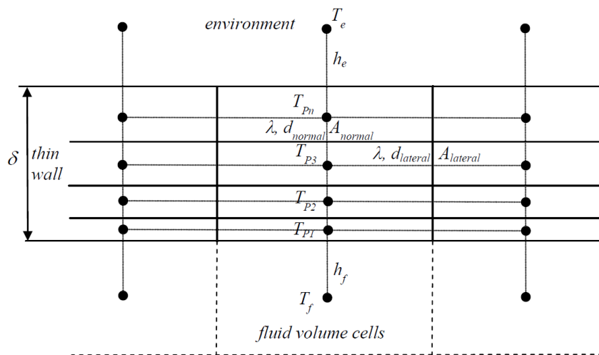
Figure 11. Principal design for thin wall mesh (from AVL Fire manual).
