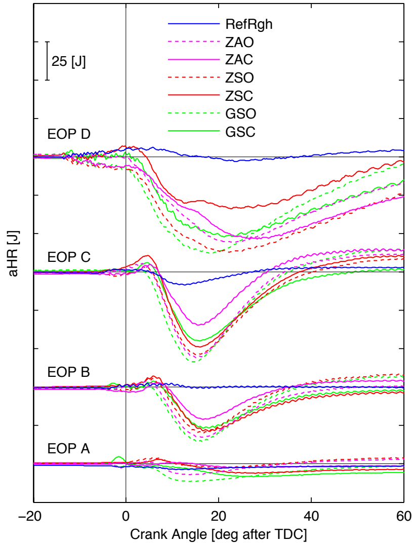
Figure 37. Apparent cumulative heat release for the rough uncoated piston and the coated pistons, relative to the stock reference piston. Explanation for the labels is found in Table 8.
