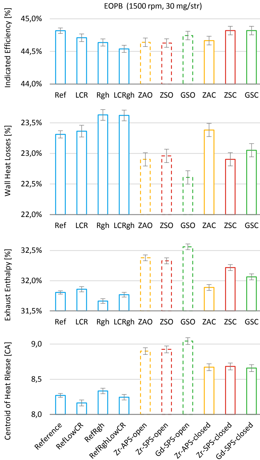
Figure 35. Fuel energy distribution for EOP B as measured. The error bars show the 95% confidence intervals. Explanation for the labels is found in Table 8.
