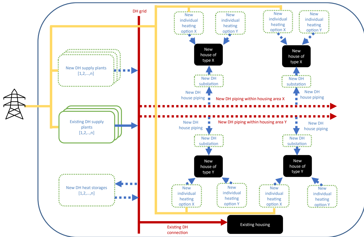
Figure 1. Schematic overview of the heating system. Figure adapted from Paper V. Heat storages are only included in Papers IV and V. In addition, in Papers I–III, the piping within a specific housing area is not distinguished from the piping going into a specific house.
