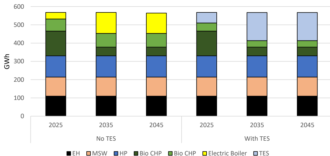
Figure 5. DH heat output for the different sources in the coldest month of the selected years for the High2030 electricity price case in Paper IV.
