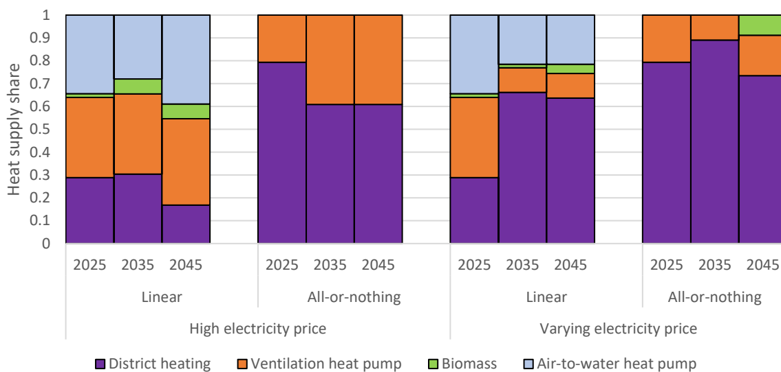
Figure 6. Heating solutions for new large apartments buildings constructed in 2020, for different electricity price cases. The figure is adapted from Paper III. The linear category indicates where there is no minimum investment cost and that the cost of installing a certain technology increases linearly with the installed capacity. The all-or-nothing categories indicate where new installations have to be of sufficient size to cover the full heat demand during all time periods. The ventilation HPs can, however, cover part of the heat demand.
