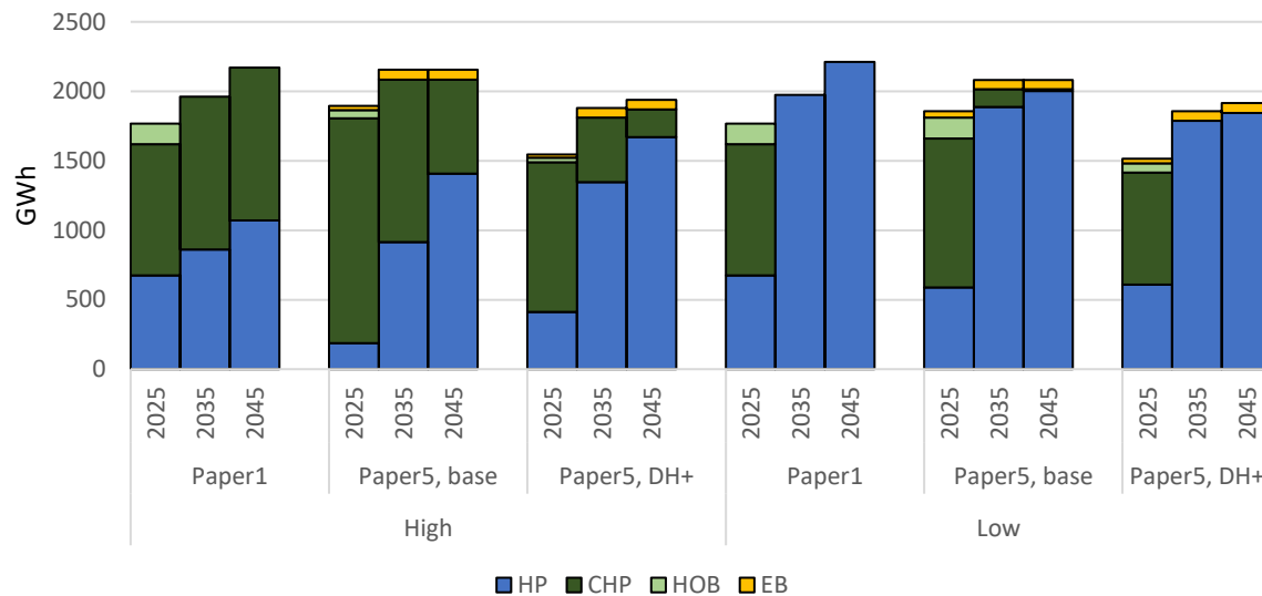
Figure 3. DH heat production levels (in GWh) from the different sources (HP, bio CHP, bio HOB and EB) for different electricity price cases and years. Values adapted from Papers I and V. Paper 5 DH+ indicates a scenario in which there is a decrease in the DH temperature and there is addition of a new low-grade industrial EH source, but there is no TES. For all the presented graphs, the EH and MSW incineration values have been omitted to improve readability.
