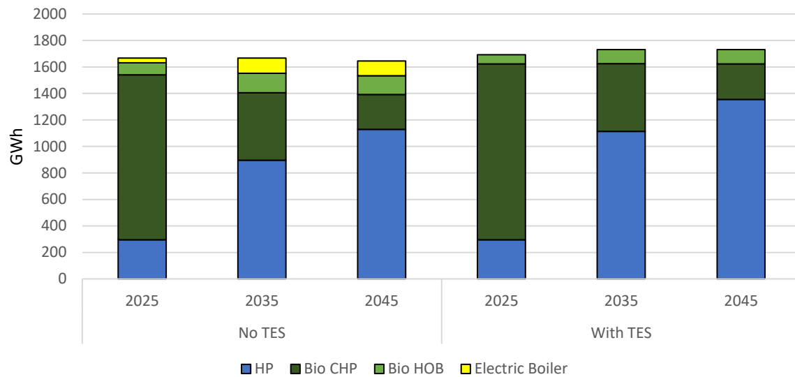
Figure 4. Annual DH production levels of heat in the High2030 electricity price scenario in Paper IV. The values for EH and MSW incineration have been omitted to improve readability.
