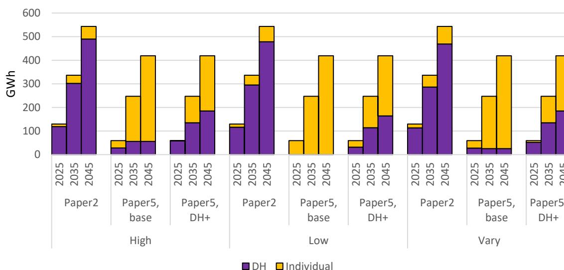
Figure 2. DH heat production levels (in GWh) from DH and individual heating sources for the new housing added to the heating system for different electricity price cases and years. Values are adapted from Papers II and V. The values acquired from Paper V are for the base scenario (base), and in which the circumstances for DH are favorable (DH+), i.e., a decrease in the DH temperature and the addition of a new low-grade industrial EH source, but without TES. The lower total heat demand in Paper V, as compared to Paper II, is due to the later starting year in Paper V compared to Paper II.
