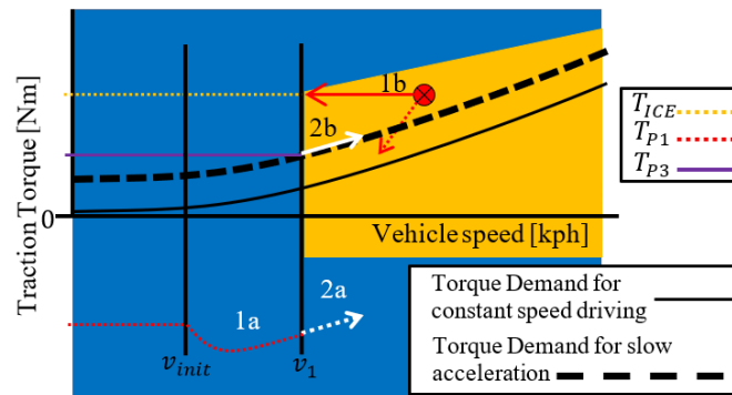
Figure 30 Mode switch for slow acceleration
