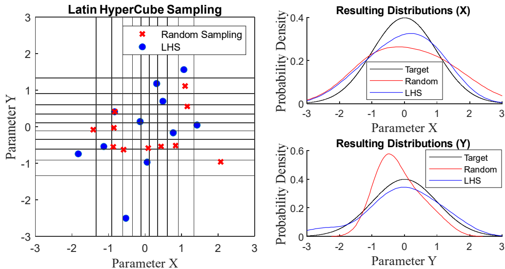
Figure 13. On the left, a parameter space is sampled via random sampling (red x's) and Latin Hypercube Sampling (LHS—blue dots). For the LHS sampling, the x and y dimensions are stratified at intervals of equal probability. On the right, the probability density functions (PDFs), resulting from random (red line) and LHS sampling (blue line), are compared against the target distributions (black line) for the x and y dimensions. These PDFs are estimated via kernel density estimation (see Section 4.4).
