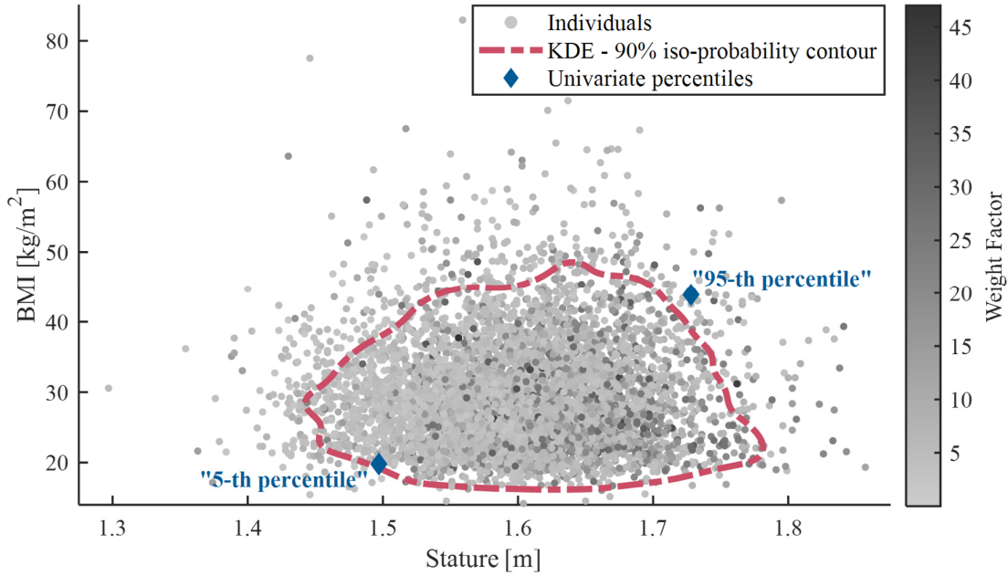
Figure 21. Bivariate distribution of stature and BMI for the female US population. Individuals are depicted with grey dots, and the intensity reflects the weight of the data point to make it representative of the US population. An iso-probability contour line in red, generated using KDE, brackets 90% of the population. The 5 th and 95 th percentile females (using univariate analysis on the same population) are represented with blue diamonds.
