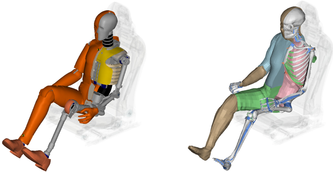
Figure 9. Illustration of numerical models of an ATD (on the left) and an HBM (on the right). The ATD is a mechanical surrogate model of an occupant. In contrast, the HBM is a direct numerical model of an occupant.
