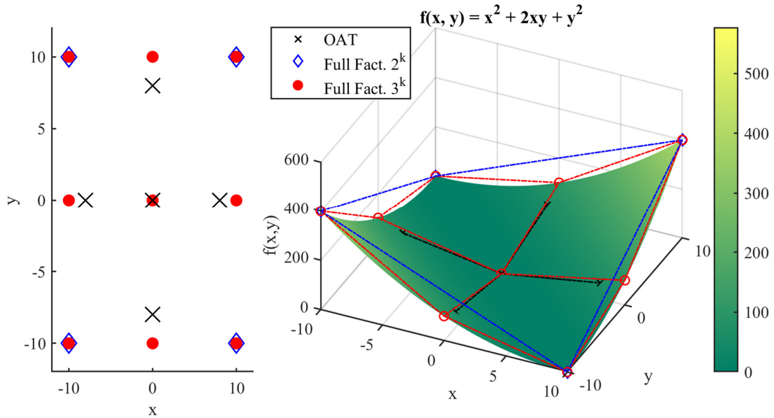
Figure 14. On the left, an example of a One-At-a-Time (marked by black x's) design and two full factorial designs ( 2^k and 3^k , represented with blue diamonds and red dots, respectively) can be seen. On the right, the response surface of an example function is illustrated with a colour map indicating the function's response. It becomes evident that the OAT design (black lines) overlooks interaction effects between x and y , which are pronounced in this example. Moreover, the 3^k design captures the non-linearities, which the 2^k design fails to reveal.
