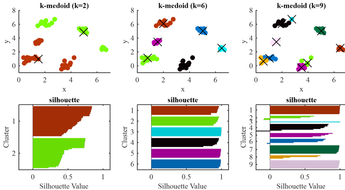
Figure 12. At the top (left to right), an example of clustering applied to a set of randomly generated data using the k-medoid algorithm for two, six, and nine clusters. Each cluster is visualised with a distinct colour, and a black x marks its medoid. At the bottom, the silhouette scores corresponding to each choice of k (number of clusters) are displayed. A high average silhouette score indicates the appropriate k for the dataset, which, in this case, is k = 6 .
