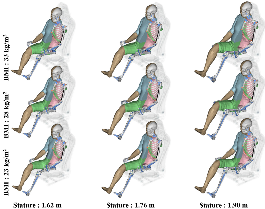
Figure 10. Illustration of morphed Human Body Models (HBMs) featuring male body geometries with a BMI range of 23–33 kg/m 2 and stature extending from 1.62 to 1.9 meters.
