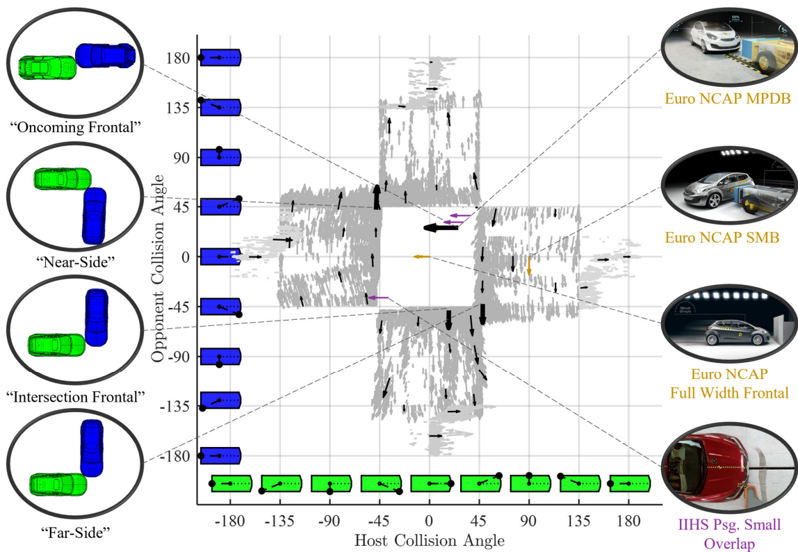
Figure 22. A “crash configuration map” depicting the expected crash scenarios after pre-crash interventions within SCP at urban intersections and SD—ref on highways. Crash configurations are shown as arrows, indicating the impact location by their origin and the relative movement direction of the involved vehicles. The arrow length corresponds to the closing speed. Grey arrows show all predicted configurations after the AEB intervention in Paper I; black arrows denote the representative subset (selected through clustering). The configurations analysed in Papers II–IV are detailed on the left and juxtaposed with standardised crash configurations from Euro NCAP and IIHS on the right. [source: adapted from euroncap.com and iihs.org]
