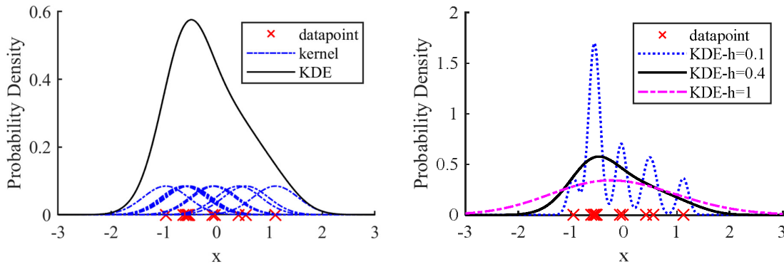
Figure 15. On the left, a random data set is presented along the x -axis (red x 's). A kernel (blue dashed lines) is placed at every data point. Summing these kernels generates the kernel density estimation of the PDF (solid black line). On the right, three PDFs derived from the same set of data points, utilising three different bandwidths. A low bandwidth produces a higher resolution (dotted blue line), whereas a higher value leads to a smoother PDF (dashed magenta line). Silverman’s method provides a balanced estimate (solid black line).
