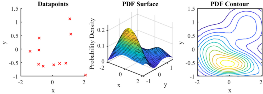
Figure 16. Kernel density estimation applied to a 2D dataset (on the left), with the estimated PDF as a 3D surface (in the centre). A corresponding contour plot (on the right) displays iso-probability lines for equal probability points in the space.
