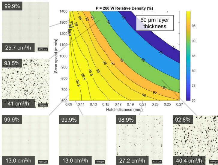
Figure A1. Comparison of predicted density at 60 \mu\text{m} layer thickness and micrographs of measured samples illustrating the accuracy of the regression model. Observations of how the porosity changes at different build rates \text{cm}^3/\text{h} can be seen in each micrograph. Each micrograph represents a 5 mm \times 5 mm area of sample cross-sections parallel with the build direction (BD).
