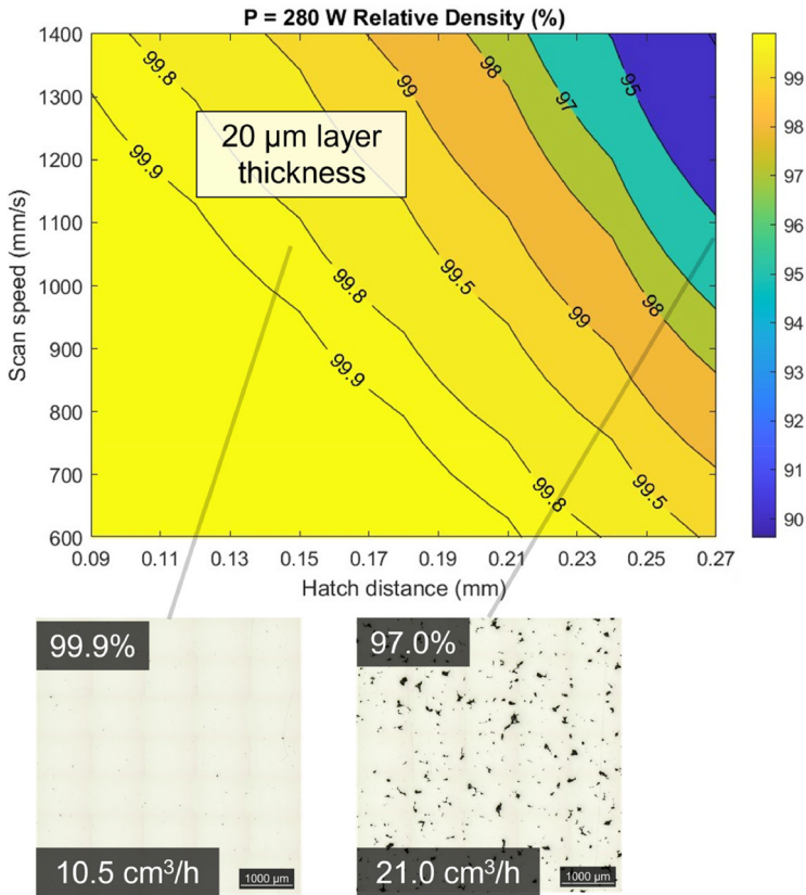
Figure A3. Comparison of predicted density at 20 \mu\text{m} layer thickness and micrographs of measured samples illustrating the accuracy of the regression model. Observations of how the porosity changes at different build rates \text{cm}^3/\text{h} can be seen in each micrograph. Each micrograph represents a 5 mm \times 5 mm area of sample cross-sections parallel with the build direction (BD).
