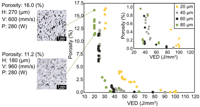
Figure 4. Porosity content vs. VED. Effect of VED ( \text{J}/\text{mm}^3 ) on the porosity (%) as measured by image analysis at 20, 40, 60, and 80 \mu\text{m} layer thickness.
