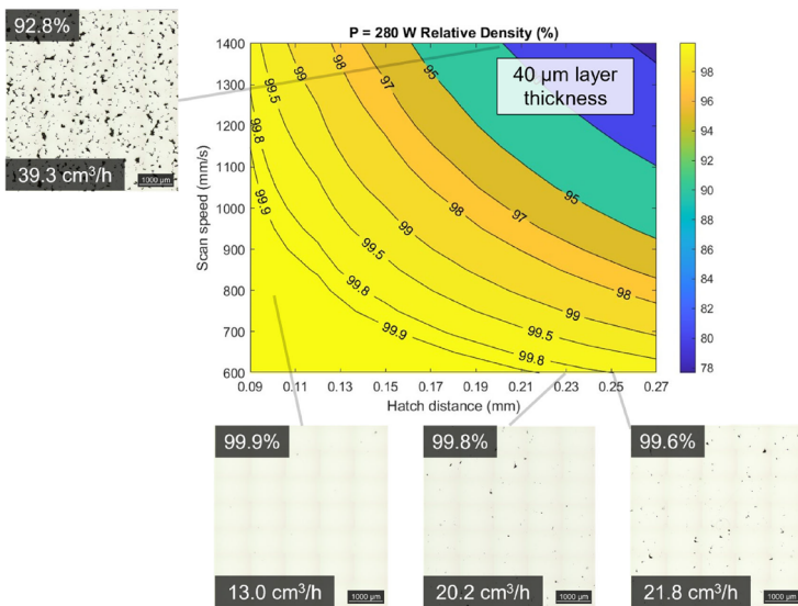
Figure A2. Comparison of predicted density at 40 \mu\text{m} layer thickness and micrographs of measured samples illustrating the accuracy of the regression model. Observations of how the porosity changes at different build rates \text{cm}^3/\text{h} can be seen in each micrograph. Each micrograph represents a 5 mm \times 5 mm area of sample cross-sections parallel with the build direction (BD).
