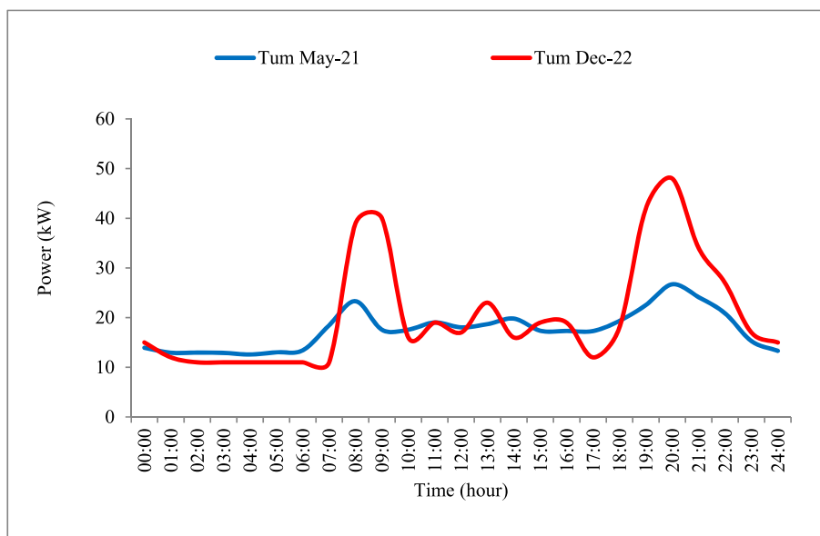
Fig. 9. The average load profiles at Tum in May 2021 and December 2022.
