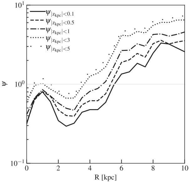
Figure A3. Radial profiles of \psi (physical equipartition between \mathbf{B} and CRs), or \langle e_{\text{CR}} \rangle_V / \langle u_B \rangle_V , in cylindrical annuli of varying height from the mid-plane for m12f. For a cylindrical annulus of a given height, in the inner disc where gas densities are high, magnetic energy densities can dominate CR energy densities at the factor of \sim 2 level for cylindrical heights \leq 1 kpc in this volume-averaged sense, with this trend increasing as more of the dense mid-plane gas is sampled (lower heights). In the outer disc, where gas densities are lower, CRs start to dominate the relative energy density, with the effect accentuated by sampling more ‘halo’ gas at larger heights above the disc, where e_{\text{CR}} tends to dominate u_B by factors of \sim 2 –4 for heights \leq 1 kpc at the very outer radii (Ponnada et al. 2022).
