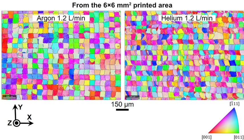
Figure 3. Extracted IPF maps of the reconstructed parent \beta grains in the building plane of the 6×6 mm 2 samples produced under Ar and He and a flow of 1.2 L/min.
