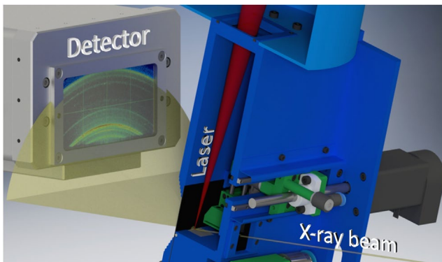
Figure 1. Diffraction geometry of the system during an operando measurement of the LPBF process. The X-ray beam enters the printer (in blue) from one side through a glassy carbon window, and is diffracted on the powder bed forming a diffraction cone collected by the high-speed detector, while the laser (red) scans the powder bed. 1
