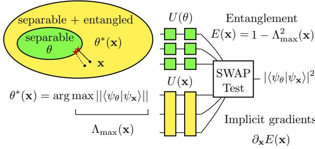
Figure 5.2: A geometric measure of entanglement defines the entanglement for a variational state \psi_{\mathbf{x}} using an optimization over all possible separable states \psi_{\theta} . This measure of entanglement E(\mathbf{x}) , therefore, does not have an analytical form, so it is not possible to write the gradient \partial_{\mathbf{x}} E(\mathbf{x}) analytically. However, implicit differentiation can compute this gradient and can be used to optimize the parameters \mathbf{x} to generate entangled states variationally as we show in Paper IV.
