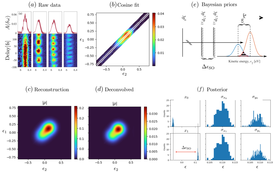
Figure 4.3: Bayesian estimation of the density matrix for a photoelectron. We focus on reconstructing the magnitude of the density matrix |\rho| from a partial estimate using prior information. (a) Raw data is converted to sub-diagonals through a cosine fit. (b) We only have access to a few sub-diagonals and wish to reconstruct the full matrix. (c) Bayesian estimation reconstructs the full matrix under a smooth model using Gaussian functions. (d) The underlying density matrix is estimated using a forward convolution in the model instead of deconvolving the result in (c). Prior knowledge from physics, e.g., the spin-orbit coupling determining the separation between peaks, can be enforced easily within the Bayesian model. (f) We obtain parameter samples that allow the calculation of uncertainties in an interpretable way.
