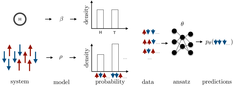
Figure 1.1: A classical coin flip can be modeled as a random experiment with two outcomes (a Bernoulli trial) by specifying the probability of heads. We can observe samples by flipping the coin to infer the probability of heads. Similarly, an interacting quantum system, e.g., spins, can be described by a density matrix \rho that defines probabilities for various measurement outcomes. The dimension of \rho grows exponentially with the system size, making it difficult to tackle larger problems using classical computers, necessitating a tunable quantum device such as a quantum computer. However, if specific constraints exist on the physical system, the probability distribution of outcomes could become simpler. An efficient and flexible ansatz, such as a neural network trained on data, could learn the underlying distribution and predict outcome probabilities or generate samples for outcomes efficiently.
