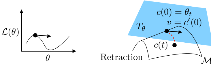
Figure 3.2: Gradient descent on a manifold \mathcal{M} starts by initializing \theta \in \mathcal{M} and calculating the cost gradient \nabla_{\theta}\mathcal{L}(\theta) . Unlike the usual update \theta' = \theta - \eta\nabla_{\theta}\mathcal{L}(\theta) , here, a descent direction v \in T_{\theta} is determined in the manifold's tangent space. The parameter update follows a curve on the manifold using a technique called retraction. The retraction ensures that the update respects the descent direction while keeping parameters on the manifold.
