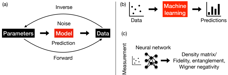
Figure 2.2: Many problems in the scientific domain can be framed as inverse problems. (a) Inverse problems involve parameter estimation from data using a forward model which is often ill-posed due to noisy or insufficient data. Regularization, constraints, and prior knowledge mitigate ill-posedness and the need for large amounts of data. (b) Machine learning offers an alternative to parameter estimation by predicting quantities of interest directly from data with an approximate model. (c) Neural networks can be used for such modeling, e.g., in quantum state tomography, where they can predict or approximate properties of quantum states from measurement data.
