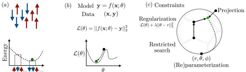
Figure 3.1: (a) Optimization could involve finding the lowest-energy configuration for a spin system. (b) Model fitting by minimizing a loss function using data. (c) Constraints can be handled in various ways, e.g., if the feasible set of parameters lies on a sphere, we could add penalty terms that add a cost to violating the constraint. Projections find the nearest feasible solution after an unconstrained optimization. A reparameterization could transform the constrained optimization into an unconstrained problem. Finally, some techniques only search the space of feasible solutions by cleverly traversing from one feasible point to another.
