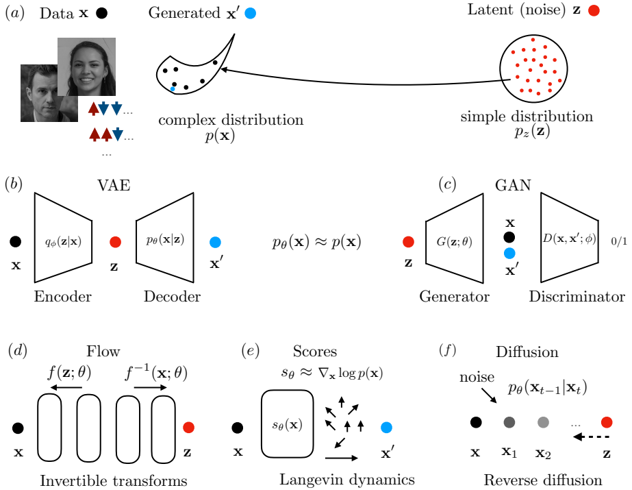
Figure 2.5: (a) Generative modeling with neural networks approximates a data distribution or sample from it using latent (noise) vectors. (b) VAEs maximize the ELBO with an encoder-decoder framework. (c) GANs directly generate samples using a neural network to assess their quality against a dataset. (d) Flow-based models learn invertible transformations of the data to noise that makes the likelihood tractable. (e) Score-based models approximate score function, i.e., the gradient of the log-likelihood that eliminates the intractable partition function. Langevin dynamics generate new data from the approximated score function. (f) Diffusion models reverse a diffusion process that gradually corrupts data by adding noise. The reverse process allows the generation of new data from noise after training.
