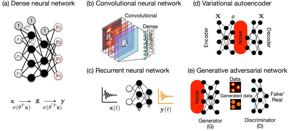
Figure 2.4: (a) A feed-forward, densely connected neural network applies linear and nonlinear transformations to create a learnable function. (b) Convolutional neural networks mimic the human visual cortex by extracting features through spatial filters and use these features, and a feed-forward network in the end, to predict labels. (c) Recurrent neural networks work with sequential data and emulate memory effects through self-connections. (d) Variational autoencoders learn data distributions via an encoder-decoder setup and generate new data resembling the input dataset. An easy-to-sample distribution generates random vectors that are then converted to data by the decoder. (e) Generative adversarial neural networks use competing networks to learn data distributions. The generator produces data from noise vectors and is trained by using a discriminator for assessment.
