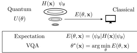
Figure 5.1: Variational quantum algorithms use a quantum computer to generate variational quantum states and compute a function e.g., an expectation value. These expectation values can define a parameterized function that a classical computer can optimize, such as the energy of some quantum system. The optimization objective could be to minimize the energy. Implicit differentiation allows the computation of the gradient of the VQA solution without having to keep track of the classical optimization saving on the memory cost associated with keeping track of all intermediate steps in the VQA that reverse-mode automatic differentiation would require. In quantum problems, storing such intermediate steps in classical memory might be impossible.
