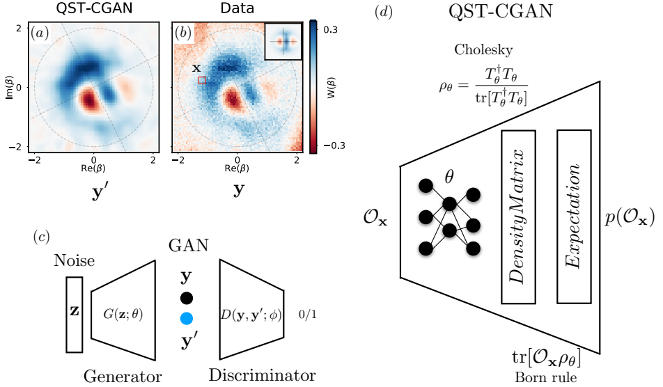
Figure 4.1: Generative models approximate an underlying probability distribution and learn it from data. We develop a method for quantum state tomography with conditional generative adversarial networks (QST-CGAN) in Papers I and II. QST-CGAN learns a representation of an underlying quantum state using experimental data. (a) Reconstruction of expectation values for parity measurements on the phase space by QST-CGAN. The measurement setting is given by a point in phase space specified by a complex number \beta . (b) The data is noisy and distorted from the ideal target state (inset), even if it contains the main features. Specifying the distortions mathematically in a model is difficult as we might not know the noise sources beforehand. However, a neural-network-based approach could still identify the state to classify it, as discussed in Paper II, or use the raw data's relevant features to estimate the density matrix. While standard generative adversarial networks generate unconditional samples (c), the QST-CGAN in (d) generates samples conditioned on an input measurement setting. This allows us to adapt such a generative model for approximating measurement probabilities p(\mathcal{O}_{\mathbf{x}}) . The black-box nature of the generator is simplified by forcing a density-matrix representation internally that obeys quantum-mechanical constraints. The Born rule can then predict expectation values. However, interpretability comes at the cost of scalability as the dimension of the density-matrix representation now restricts us to small system sizes.
