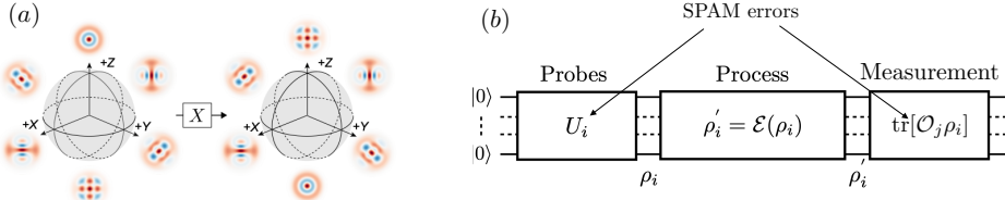
Figure 4.2: Quantum process tomography (QPT) characterizes quantum operations such as (a) transformations of a quantum state that represents some logical information. A bosonic encoding implements computational states by encoding them as orthogonal states of light, e.g., |2\rangle, \frac{|0\rangle+|4\rangle}{\sqrt{2}} . An operation such as a NOT (X) gate is a physical operation transforming one state to another. (b) QPT proceeds by preparing probe states, applying the target operation, and performing various measurements on the result. State-preparation and measurement (SPAM) errors need to be accounted for to get the true characterization of the target process \mathcal{E} . We incorporate estimated SPAM errors in the formulation of the QPT reconstruction in Paper IX.
