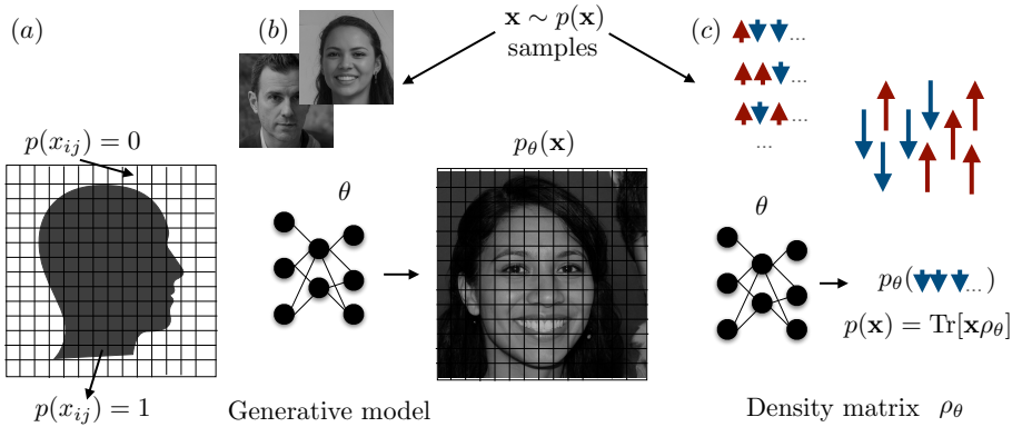
Figure 2.3: (a) Generative modeling of an underlying distribution using samples of data. The probability distribution specifying whether a pixel should be black or white to construct a human face can be complex and intractable. (b) A neural network approximates and learns the underlying probability distribution from samples of data, e.g., human faces. Once the distribution is approximated, new samples can be drawn that resemble human faces. All faces in the above figure are computer-generated; these human faces never existed [151, 152]. (c) In quantum physics, we want to model complex quantum systems to predict probabilities for measurement outcomes or other properties. The density matrix \rho allows us to predict probabilities using the Born rule. Neural-network-based models can be used to learn an efficient approximation for the underlying density matrix (or exactly, as in Papers I and II).
