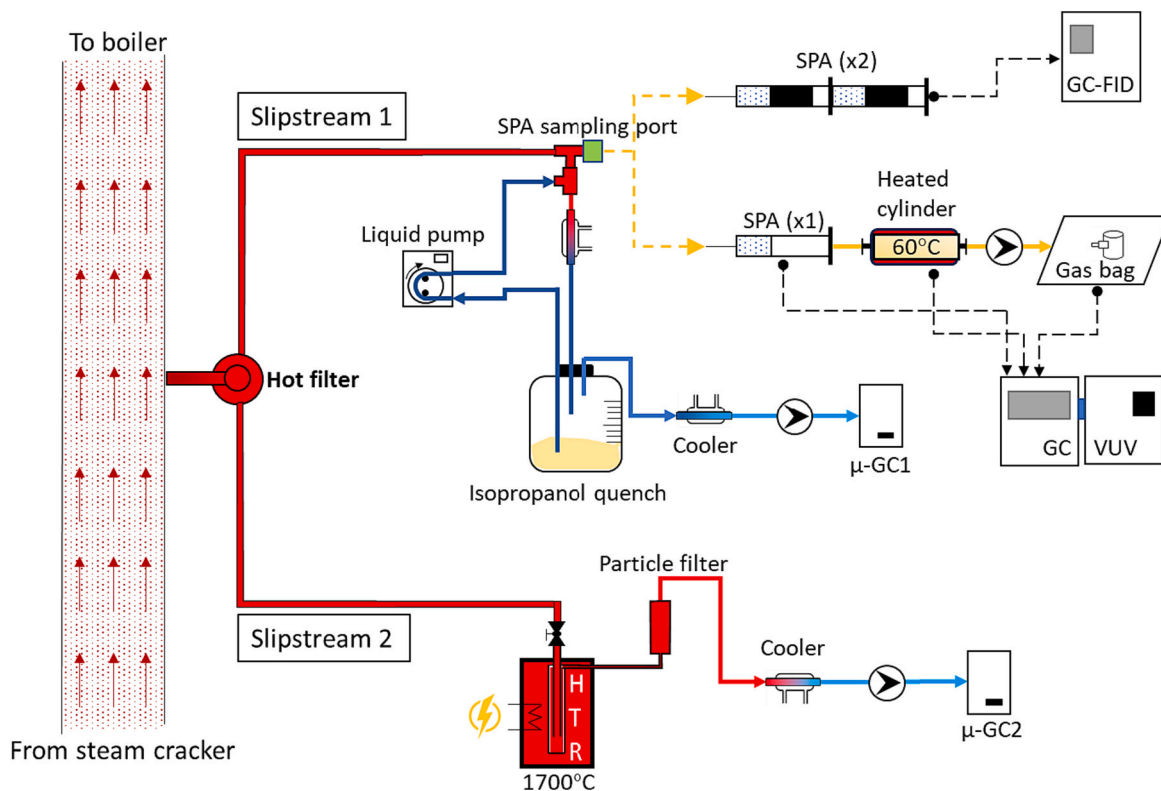
Fig. 4. Simplified schematic of the gas sampling system, including the two parallel slipstreams, and the SPA-sampling position. The hot filter is positioned at ‘point 11’ (see Fig. 2). Red colored lines are the heat-traced lines at 350 °C. The remainder of the piping correspond to the unheated side of the slipstreams. The dotted line represents offline characterization of the individual samples, while the continuous line represents online GC measurements. (For interpretation of the references to colour in this figure legend, the reader is referred to the web version of this article.)
