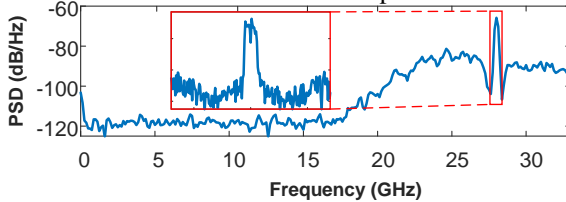
Fig. 6. Spectrum of the remote radio head output signal.
