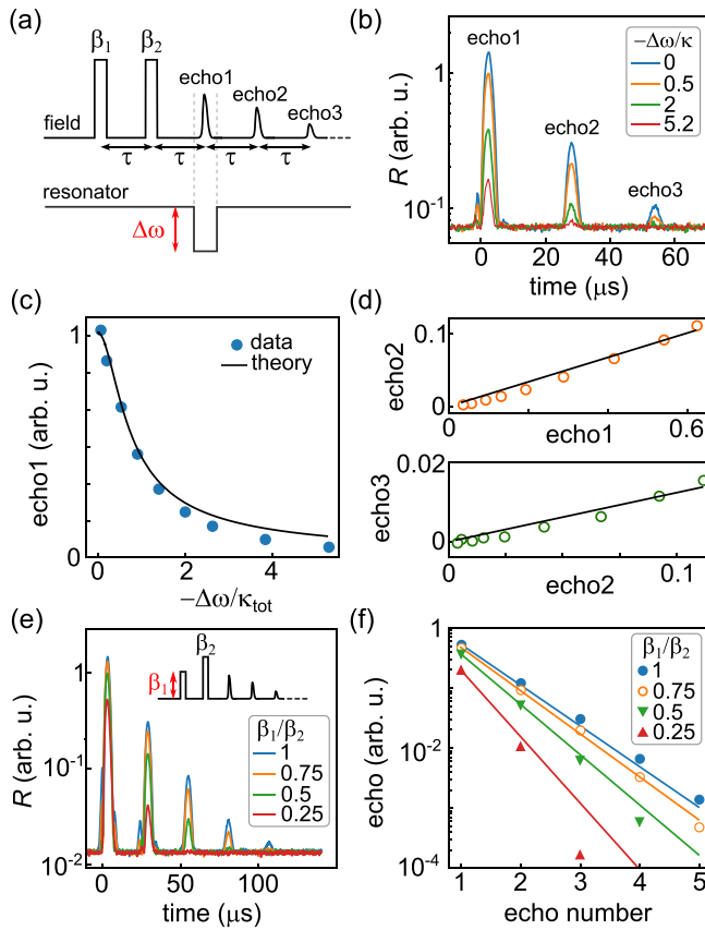
FIG. 2. SSE response vs intra-cavity field. (a) An experimental sequence consisting of two control pulses of flip angles \beta_1 and \beta_2 , and duration of 2 \mu\text{s} with a 20 \mu\text{s} long resonator detuning pulse across echo1 of varying \Delta\omega . (b) SSE traces at different \Delta\omega and same flip angles \beta = \beta_1 = \beta_2 . Larger noise floor is because of the larger measurement bandwidth BW \sim 100 \text{ MHz} compared to other plots acquired at BW of 2 \text{ MHz} . (c) Measured (symbols) and theoretical (curve) echo amplitude against different resonator detunings. (d) Scaling of echo{2, 3} amplitudes (measured: symbols and fits: lines) with corresponding changes in echo{1,2}. (e) SSE traces for different flip angles \beta_1 of the first control pulse and fixed \beta_2 . The sequence is shown in the inset. (f) SSE magnitude decay for different \beta_1 vs echo number. Solid lines are calculated from Eq. (1). For all plots C = 3 .
