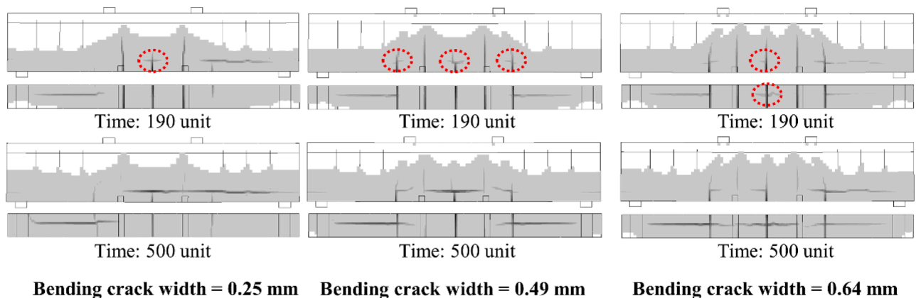
Fig. 16. Crack patterns of beams based on Case D with different bending crack widths. In each subfigure, both the front and bottom views of the beam are presented. The red-dotted circle indicates the starting locations of the corrosion-induced cracks.
