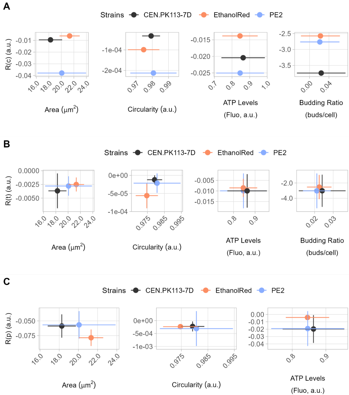
Figure 4.3. Relationship between function performance and different robustness types. Three S. cerevisiae strains were grown under feast-starvation oscillations for 16 h and four functions were monitored (budding ratio, area, circularity, and ATP levels). For each function, the performance is presented in correlation to (A) robustness across conditions R(c) , (B) robustness over time R(t) , and (C) robustness across populations R(p) . Unpublished data (Torello et al. 2024).
