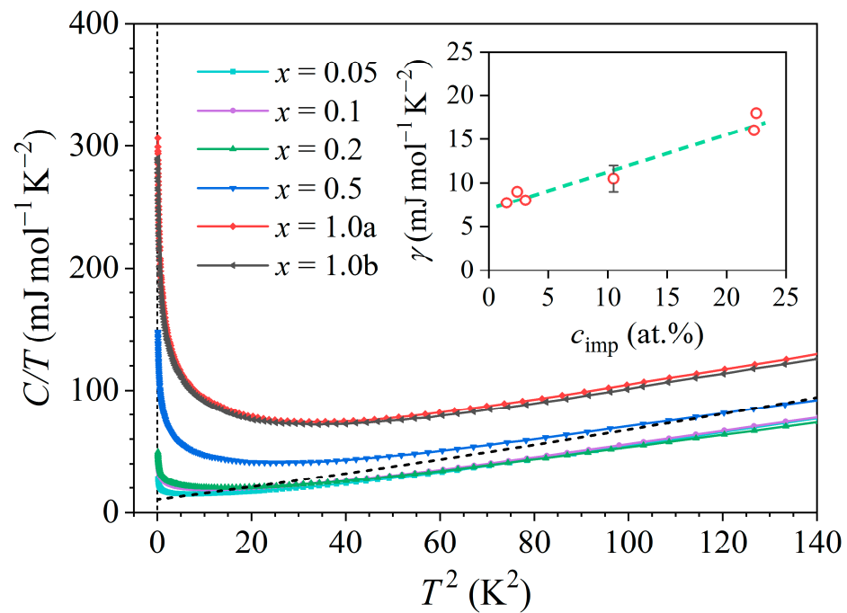
Figure 11. Zero-field specific heat of the six Ce_xLaLuScY samples at temperatures below 12 K in a C/T vs. T^2 plot. Dashed line is a \gamma + \alpha T^2 fit for the x = 0.5 sample. The inset shows the electronic coefficient \gamma as a function of the cerium concentration c_{imp} .
