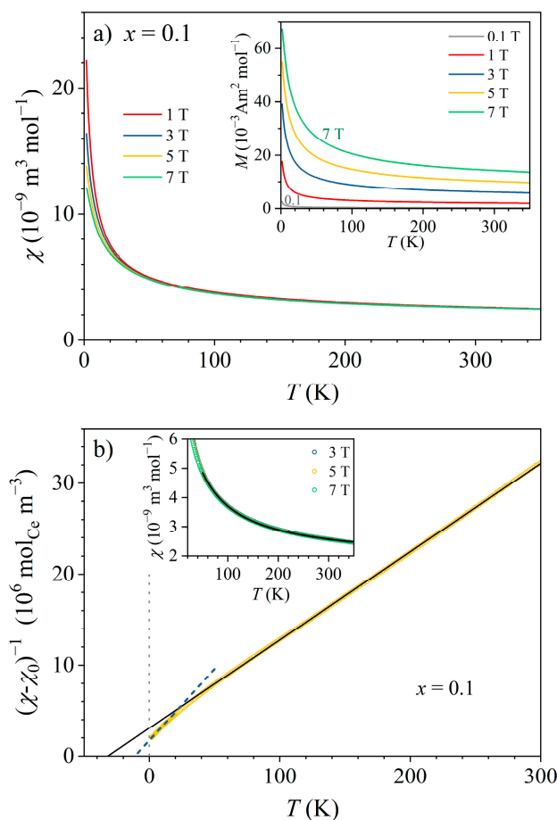
Figure 9. (a) Magnetic susceptibility \chi = M/H of the x = 0.1 sample in the temperature range 1.8–350 K in different magnetic fields (indicated in the legend). The inset shows the temperature-dependent magnetization M(T) curves. (b) (\chi - \chi_0)^{-1} versus temperature for the magnetic field of 5 T. The solid line is the Curie–Weiss fit at temperatures above 50 K, while the dashed line is the Curie–Weiss fit in the low-temperature range 1.8–9 K. The inset shows the total susceptibility \chi vs. T on an expanded vertical scale, together with the fit with Equation (3) (solid curve) in the temperature range 50–300 K (the experimental data in magnetic fields 3, 5, and 7 T are indistinguishable on the graph).
