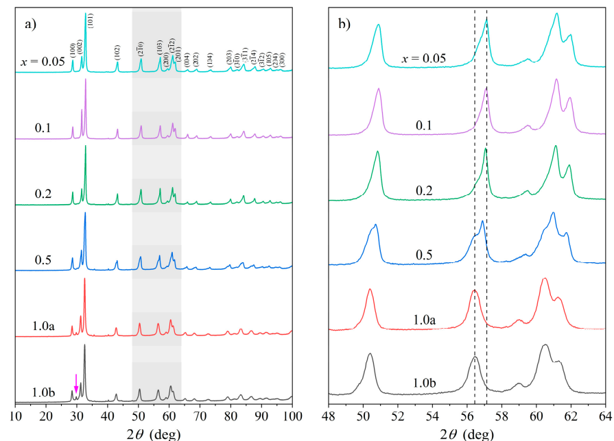
Figure 1. (a) XRD patterns of the Ce_xLaLuScY ( x = 0.05\text{--}1.0 ) HEAs at room temperature, with the Ce content x increasing from top to bottom. Miller indices hkl of the hcp-phase reflections are indicated in the x = 0.05 pattern. The arrow in the x = 1.0b pattern marks the most intense peak (111) of the ccp minority phase (at 2\theta \approx 30^\circ ). (b) Zoomed-in parts of the XRD patterns in the range of diffraction angles 48^\circ < 2\theta < 64^\circ (shaded light gray in panel (a)). The evolution of the doublet of peaks at 2\theta = 56\text{--}57^\circ with the cerium content is marked by the dashed vertical guidelines.
