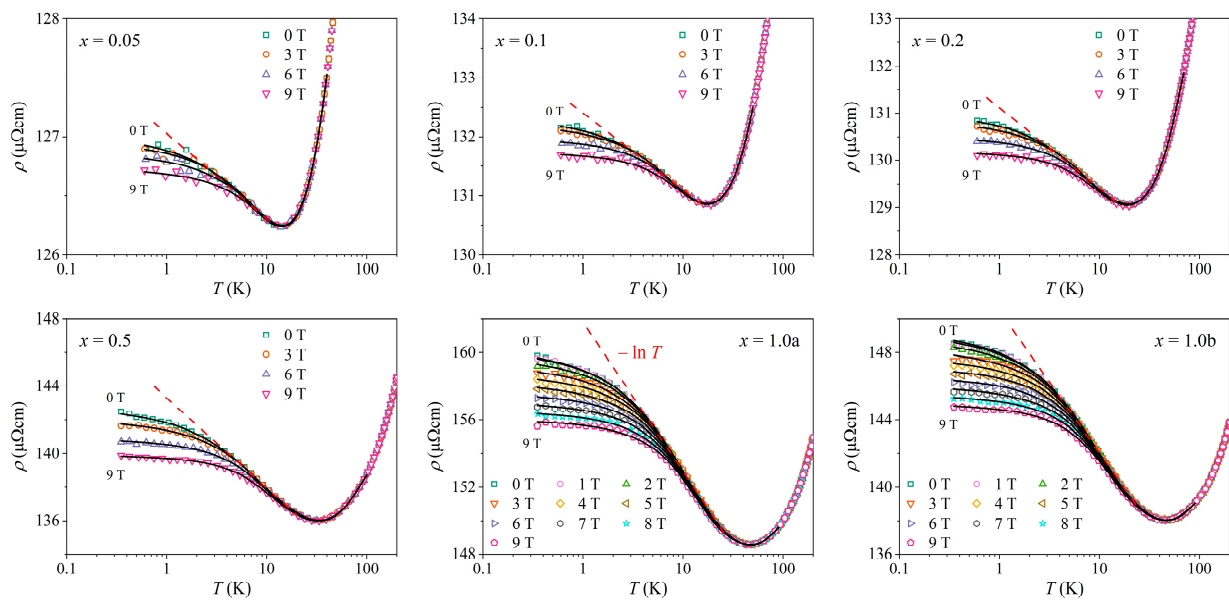
Figure 7. Temperature-dependent resistivity \rho in magnetic fields B = 0 – 9 T on a logarithmic temperature scale, shown in a separate panel for each sample. The red dashed lines indicate the \rho \propto -\ln T dependence below the resistivity minimum. Solid curves are fits with the Hamann formula in Equation (1), which is described in the text.
