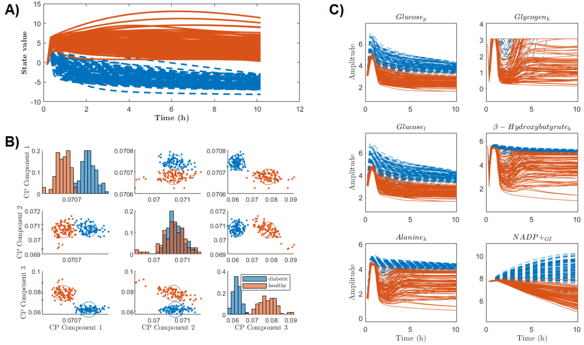
Figure 12: Identification of metabolotypes in simulated data. A) Clustering of individuals via the fourth pDMDC latent dynamic states. B) Clustering of CP scores. C) Clusters (blue and red) color-coded in contributing raw data metabolites.
