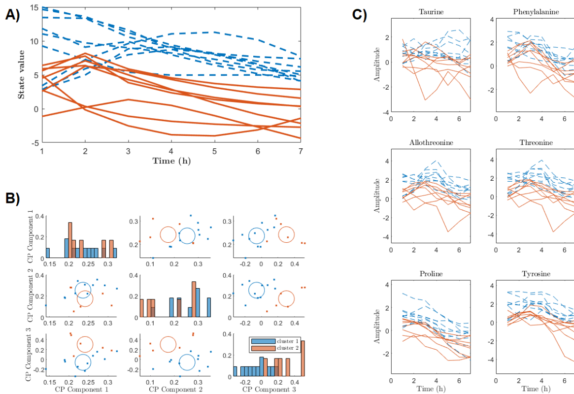
Figure 11: Identification of metabolotypes in measured data. A) Clustering of individuals via the first pDMDc latent dynamic states. B) Clustering of CP scores. C) Clusters (blue and red) color-coded in contributing raw data metabolites.
