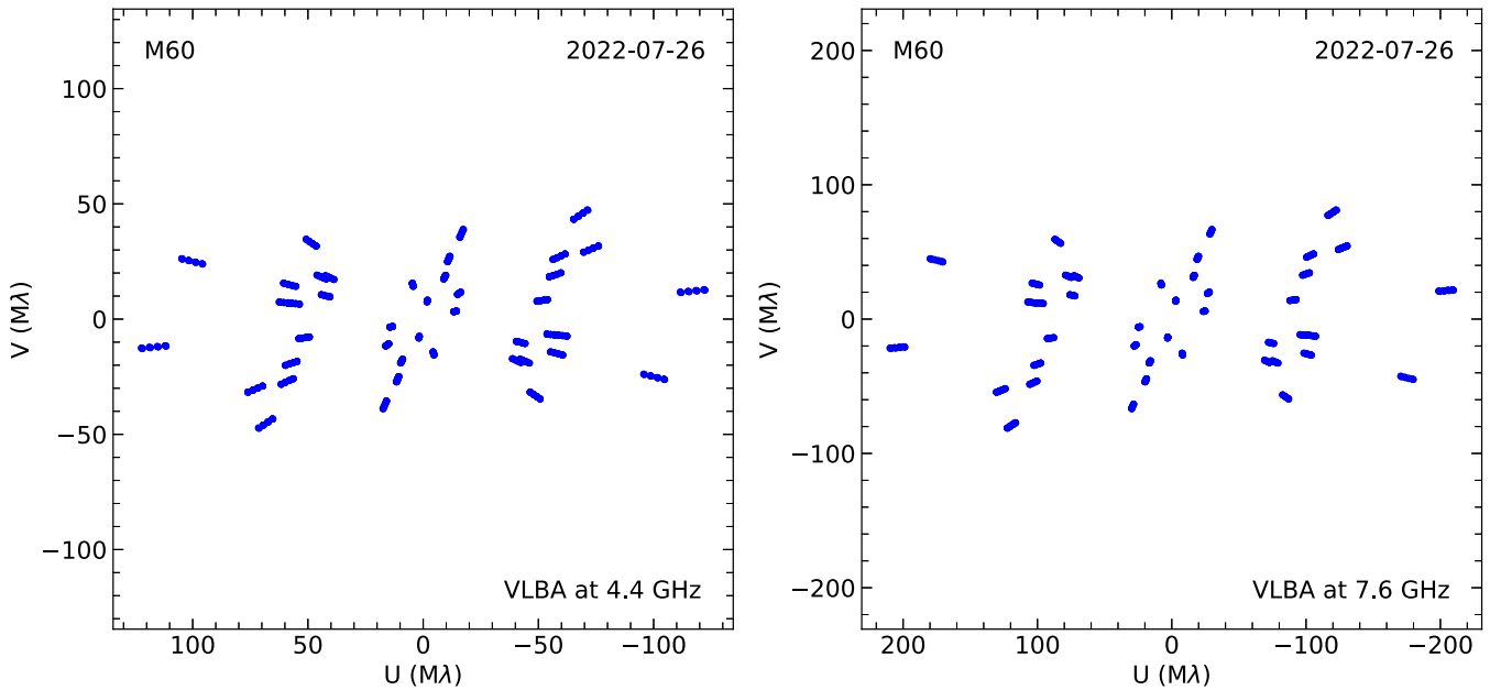
Figure 1. The (u, v) coverage for M60 at 4.4 GHz (left) and 7.6 GHz (right). The (u, v) coordinates for each pair of antennas are the baseline length projected from the source in units of the observing wavelength \lambda and are given for conjugate pairs.
