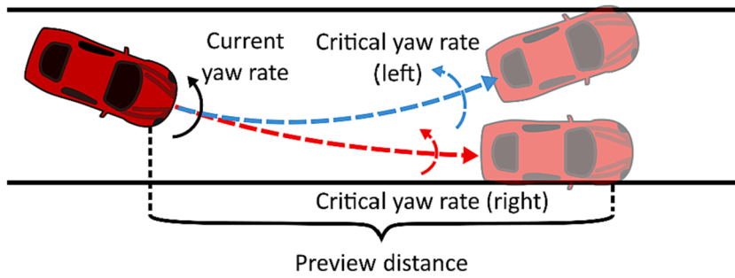
Fig. 8. An illustration of critical normalized yaw rate. The dashed lines depict the estimated vehicle trajectories corresponding to the left (blue) and right (red) critical yaw rate, with the front left or right tire of the car exiting the lane at the preview distance. In the depicted scenario, the vehicle would have departed from the lane to the right at a distance shorter than the preview distance (and not departed the lane at all to the left), had the current yaw rate been sustained. Thus, in this case, both the right and left critical yaw rate would rotate the vehicle toward the left to make it depart the (left or right) lane at the predefined preview distance. (For interpretation of the references to colour in this figure legend, the reader is referred to the web version of this article.)
