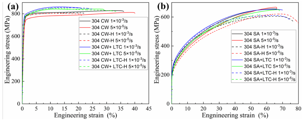
Figure 5.5 Tensile stress-strain curves of untreated and LTC treated specimens with and without hydrogen charging. (a) Cold worked condition and (b) Solution annealed condition
