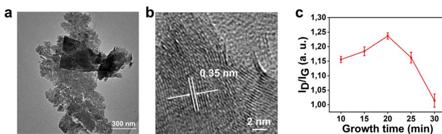
Fig. 2. Atomic structure characterization of graphene nanopikes. (a) TEM image of graphene nanopikes scratched from the substrate. (b) High-resolution TEM image of graphene nanopikes, demonstrating the atomic structure. (c) Quantification of defects density of graphene nanopikes at different growth time. The Raman intensity ratio of D peak and G peak ( I_D/I_G ) of graphene nanopikes was plotted as a function of growth time. (A colour version of this figure can be viewed online.)
