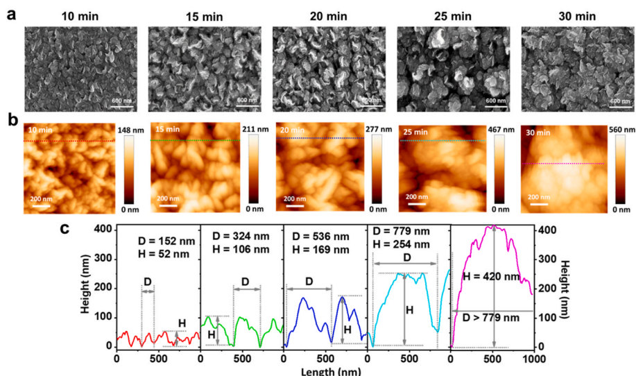
Fig. 1. Morphology and dimension characterization of graphene nanopikes. (a) SEM images of graphene nanopikes grown on silicon substrate at a growth time of 10, 15, 20, 25, and 30 min, respectively. (b) AFM height images of graphene nanopikes at different growth times. The scan area of AFM images was 1 \times 1 \mu\text{m}^2 . The dash lines in the images marked the positions where the cross-sectional profiles were extracted. (c) The correspondence cross-sectional profiles of each graphene sample extracted from AFM images above, showing the mean diameter (D) and the height (H) of graphene nanopikes produced at different growth times. (A colour version of this figure can be viewed online.)
