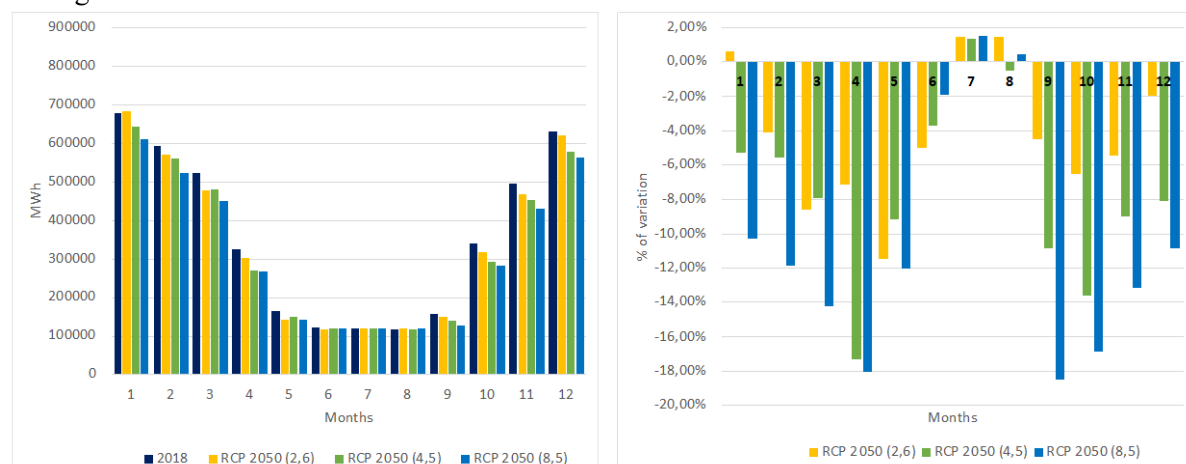
Figure 2. Monthly final energy demand (left); variation in final energy demand between TM2018 and the three RCP scenarios (right)
