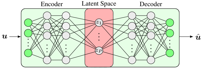
Figure 3.4: An example of an AE composed of two NNs with fully-connected architecture. The encoder and decoder NNs of the AE is connected by a shared layer (i.e., the latent representations).
