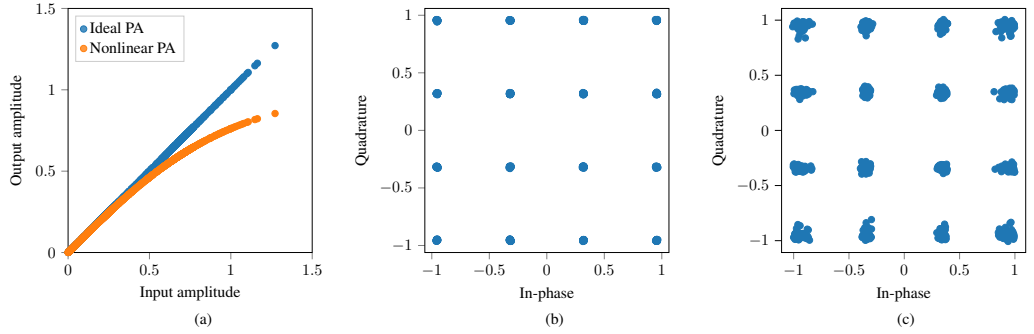
Figure 2.6: An example that illustrates the impact of using a nonlinear PA. (a) PA response; (b) Normalized received signal when PA output power is low; (c) Normalized received signal when PA output power is high.
